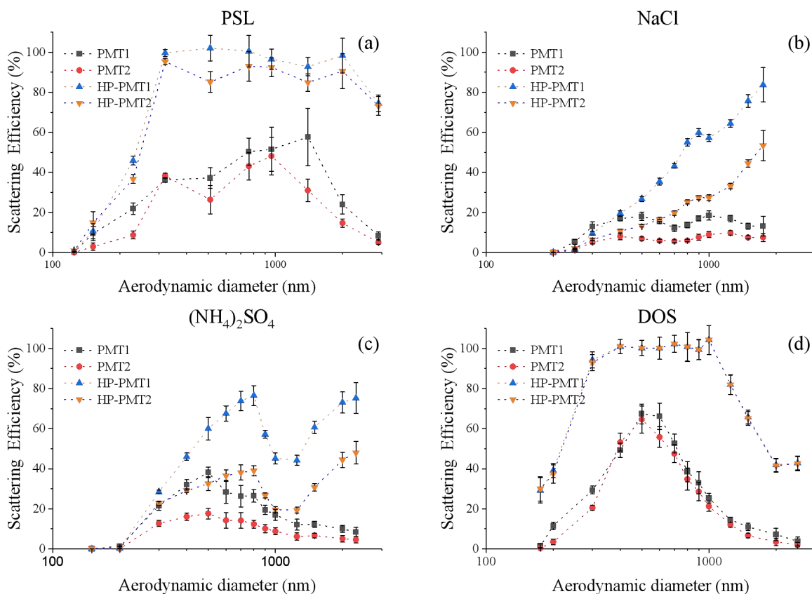
525 Figure 4: Comparison of HP-SPAMS and SPAMS for different particle sizing scattering efficiency ranged from 100–3000 nm. The PMT1 and PMT2 represent the scattering efficiencydetection-efficiencies of the two photomultiplier tubes of SPAMS, respectively, and HP-PMT1 and HP-PMT2 are the scattering efficiencydetection-efficiencies of the two photomultiplier tubes of HP-SPAMS- scattering efficiency .
