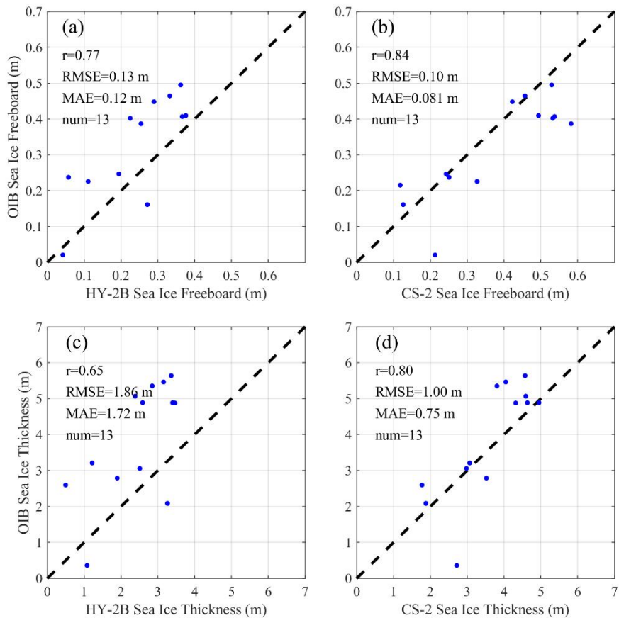
810 Figure 8. Comparative scatter plots between two satellite products and OIB collected in April 2019: (a) HY-2B sea ice freeboard vs. OIB sea ice freeboard, (b) AWI CS-2 sea ice freeboard vs. OIB sea ice freeboard, (c) HY-2B sea ice thickness vs. OIB sea ice thickness and (d) AWI CS-2 sea ice thickness vs. OIB sea ice thickness.
