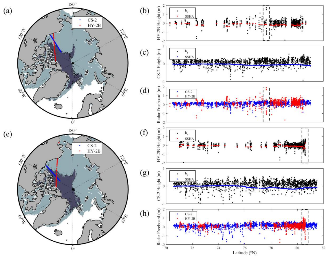
790 Figure 4. (a) (e) Cryosat-2 (blue) and HY-2B (red) tracks (acquired on April 4, 2020, and March 13, 2020, respectively) selected for comparison. FYI regions: light shading, MYI regions: dark grey shading. (b) (f) HY-2B relative surface elevations of floes (black dots) and SSHAs (red dots) corresponding to the tracks shown in panels (a) and (e), respectively. (c) (g) Cryosat-2 relative surface elevations of floes (black dots) and SSHAs (red dots) corresponding to the tracks shown in panels (a) and (e), respectively. (d) (h) Cryosat-2 (blue) and HY-2B (red) radar freeboard values corresponding to the tracks shown in panels (a) and (e), respectively.
