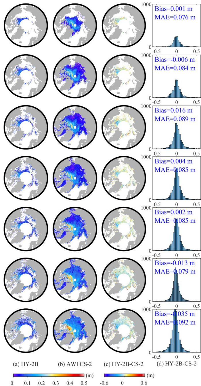
795 Figure 5. Comparisons and differences between the HY-2B radar freeboard and AWI CS-2 radar freeboard recorded from October 2019 to April 2020: (a) HY-2B radar freeboards, (b) CS-2 radar freeboards, (c) spatial differences between HY-2B and CS-2 radar freeboards, and (d) a histogram of differences between HY-2B and CS-2 radar freeboards.
