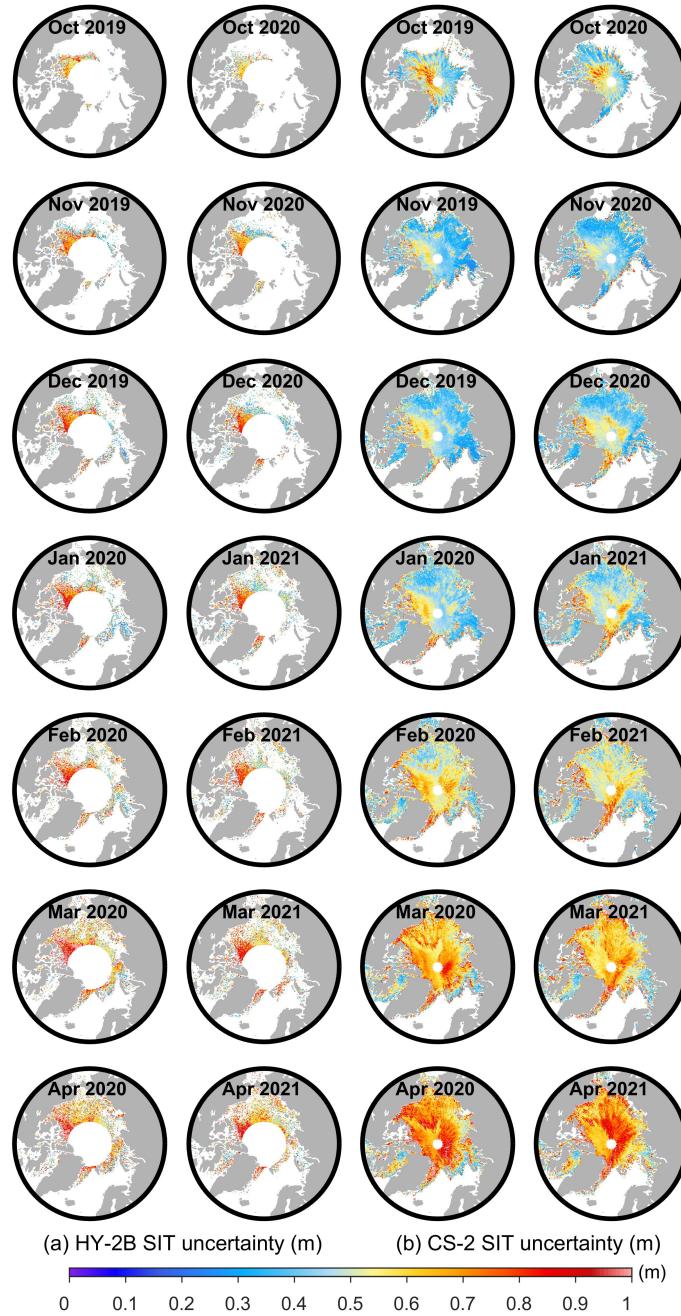
830 Figure 12. Monthly comparisons between HY-2B sea ice thickness uncertainties and CS-2 sea ice thickness uncertainties from October 2019 to April 2020 and from October 2020 to April 2021: panel (a) shows the HY-2B sea ice thickness uncertainties, and panel (b) shows the CS-2 sea ice thickness uncertainties.
