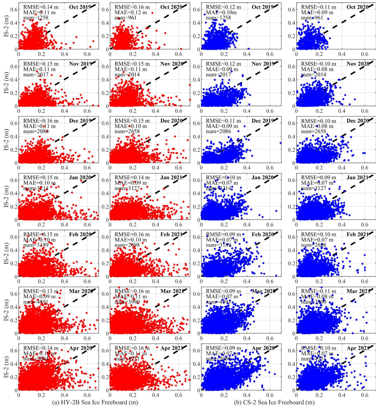
815 Figure 9. Monthly comparisons between HY-2B sea ice freeboard and ICESat-2 sea ice freeboard and between CryoSat-2 sea ice freeboard and ICESat-2 sea ice freeboard values: panel (a) shows comparisons between HY-2B and ICESat-2 in red points, and panel (b) shows comparisons between CS-2 and ICESat-2 in blue points.
