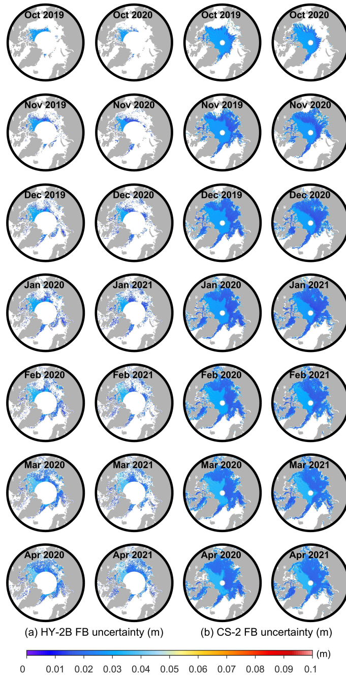
825 Figure 11. Monthly comparisons between HY-2B sea ice freeboard uncertainties and CS-2 sea ice freeboard uncertainties from October 2019 to April 2020 and from October 2020 to April 2021: panel (a) shows the HY-2B sea ice freeboard uncertainties, and panel (b) shows the CS-2 sea ice freeboard uncertainties.
