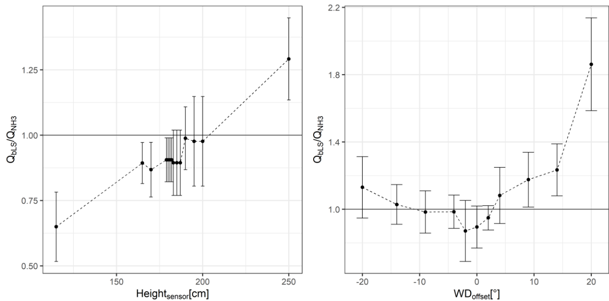
14 15 Figure S4 - Sensitivity analysis of recovered fractions Q_{bLS}/Q of ammonia based on the height of the 16 concentration sensor and wind direction offset ( WD_{offset} ) for Line 3 CRDS at 15 m distance and inlet 17 height at 187 cm height in release VIII-DK.
