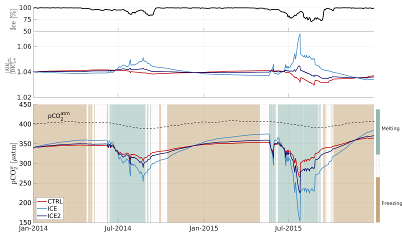
Figure 1. Model outputs for a grid cell representative of Central Beaufort Gyre ( 78^\circ N, 150^\circ W) over 2014-2015. (a): Ice concentration. (b): Surface seawater alkalinity to DIC ratio for the CTRL (no ice carbon flux; red line), ICE ( [Alk]_{ice} = 540 \text{ mmol m}^{-3} , [DIC]_{ice} = 300 \text{ mmol m}^{-3} ; light blue line) and ICE2 ( [Alk]_{ice} = 415 \text{ mmol m}^{-3} , [DIC]_{ice} = 330 \text{ mmol m}^{-3} ; dark blue line) runs. (c): Ice melt and formation ( >3 \text{ mm day}^{-1} ; background color); observed atmospheric pCO_2 at the Alert weather station (dashed black line) and simulated surface seawater pCO_2 (solid lines) for the three above-mentioned runs.
