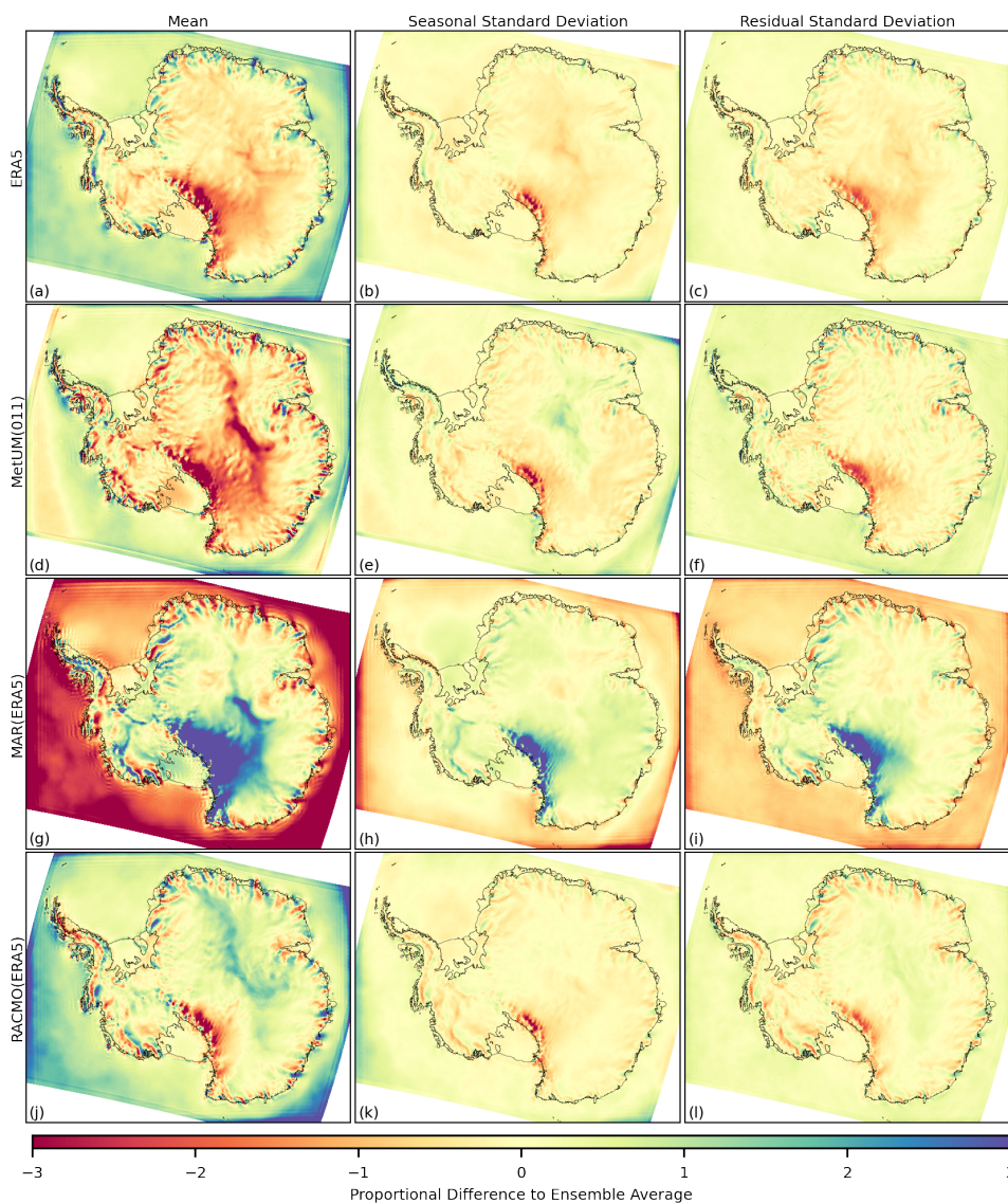
Figure 4. The difference to the ensemble average for the 1981-2018 time series of snowfall, in the mean (a,d,g,j), the standard deviation of the seasonal component (b,e,h,k) and the standard deviation of the residual component (c,f,i,l). The ensemble includes: ERA5 (a,b,c); MetUM(011) (d,e,f); MAR(ERA5) (g,h,i); and RACMO(ERA5) (j,k,l). Differences at each grid cell are expressed as a proportion of average inter-annual variation and so do not have units.
