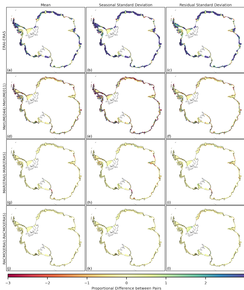
Figure B3. The difference for the 1981-2018 time series of melt, in the mean (a,d,g,j), the standard deviation of the seasonal component (b,e,h,k) and the standard deviation of the residual component (c,f,i,l) between the following pairs of outputs: ERA-Interim relative to ERA5 (a,b,c); MetUM(044) relative to MetUM(011) (d,e,f); MAR(ERAI) relative to MAR(ERA5) (g,h,i); RACMO(ERAI) relative to RACMO(ERA5) (j,k,l). Differences at each grid cell are expressed as a proportion of average inter-annual variation and so do not have units.
