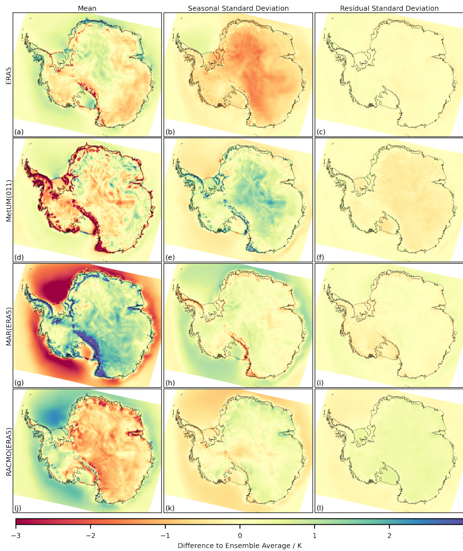
Figure 5. The difference to the ensemble average for the 1981-2018 time series of near-surface air temperature, in the mean (a,d,g,j), the standard deviation of the seasonal component (b,e,h,k) and the standard deviation of the residual component (c,f,i,l). The ensemble includes: ERA5 (a,b,c); MetUM(011) (d,e,f); MAR(ERA5) (g,h,i); and RACMO(ERA5) (j,k,l).
