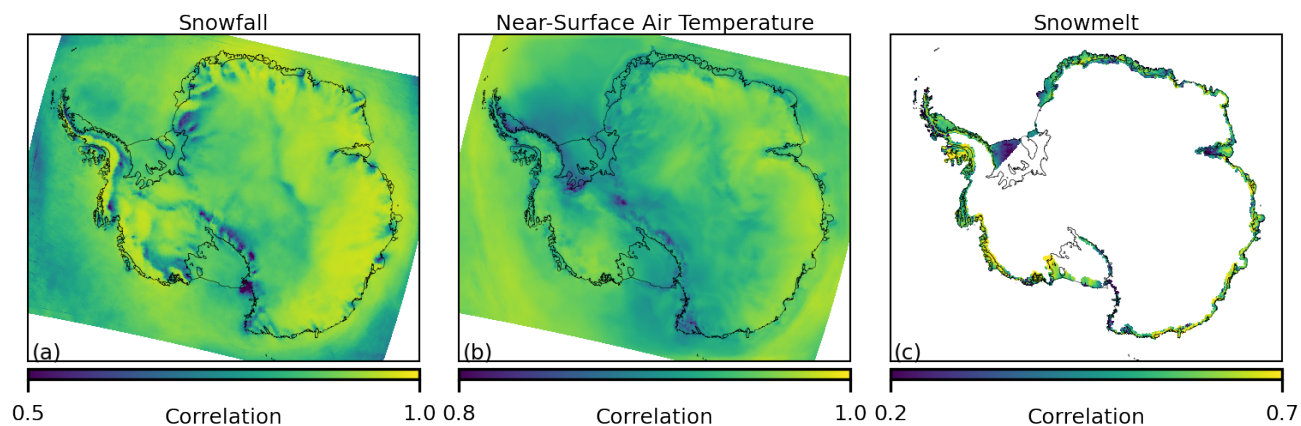
Figure 3. The median correlation by grid-cell in the residual component of the monthly time series between the 28 unique model pairs for snowfall (a), near-surface air temperature (b) and melt (c).
