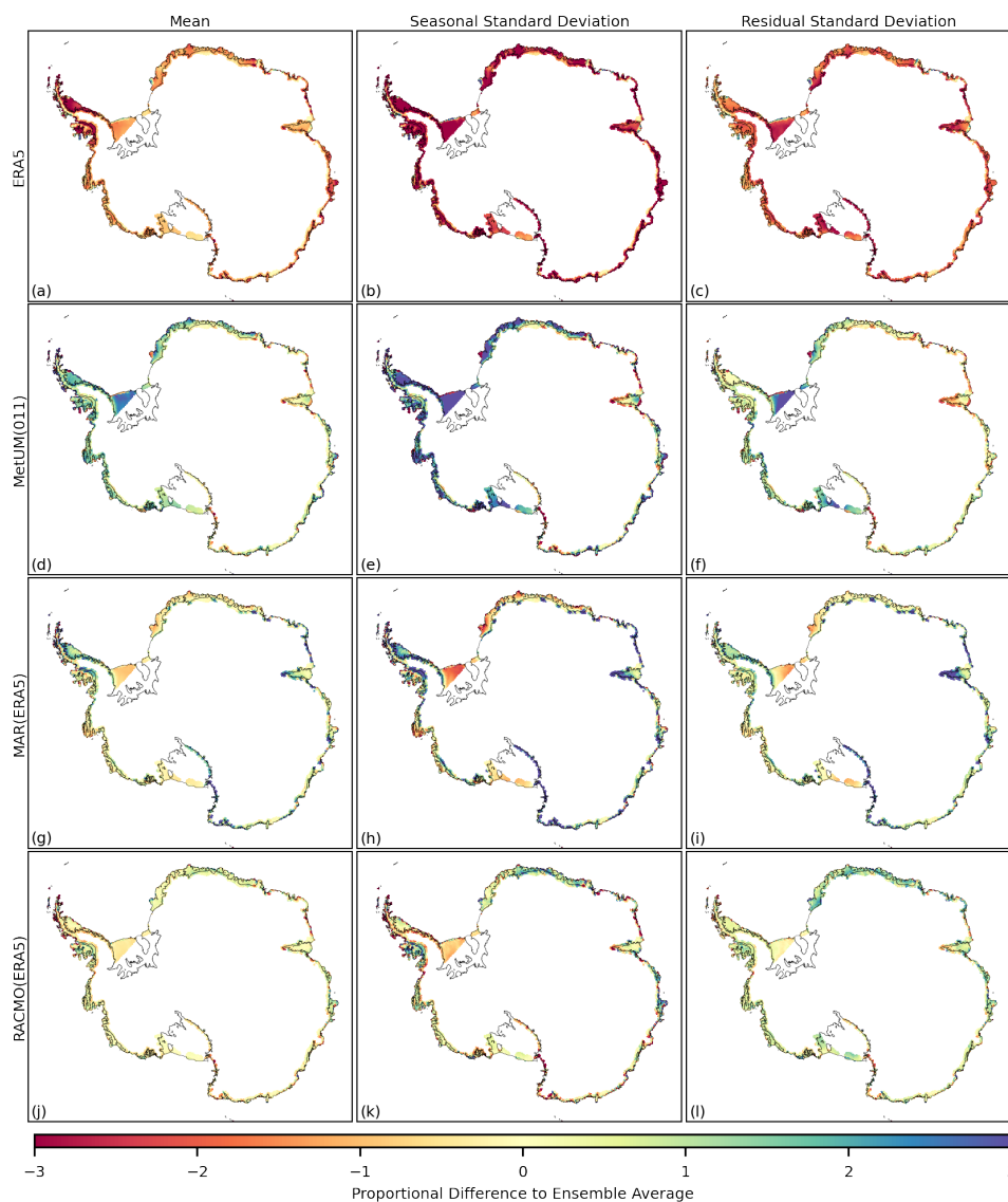
Figure 6. The difference to the ensemble average for the 1981-2018 time series of melt, in the mean (a,d,g,j), the standard deviation of the seasonal component (b,e,h,k) and the standard deviation of the residual component (c,f,i,l). The ensemble includes: ERA5 (a,b,c); Me-tUM(011) (d,e,f); MAR(ERA5) (g,h,i); and RACMO(ERA5) (j,k,l). Differences at each grid cell are expressed as a proportion of average inter-annual variation and so do not have units.
