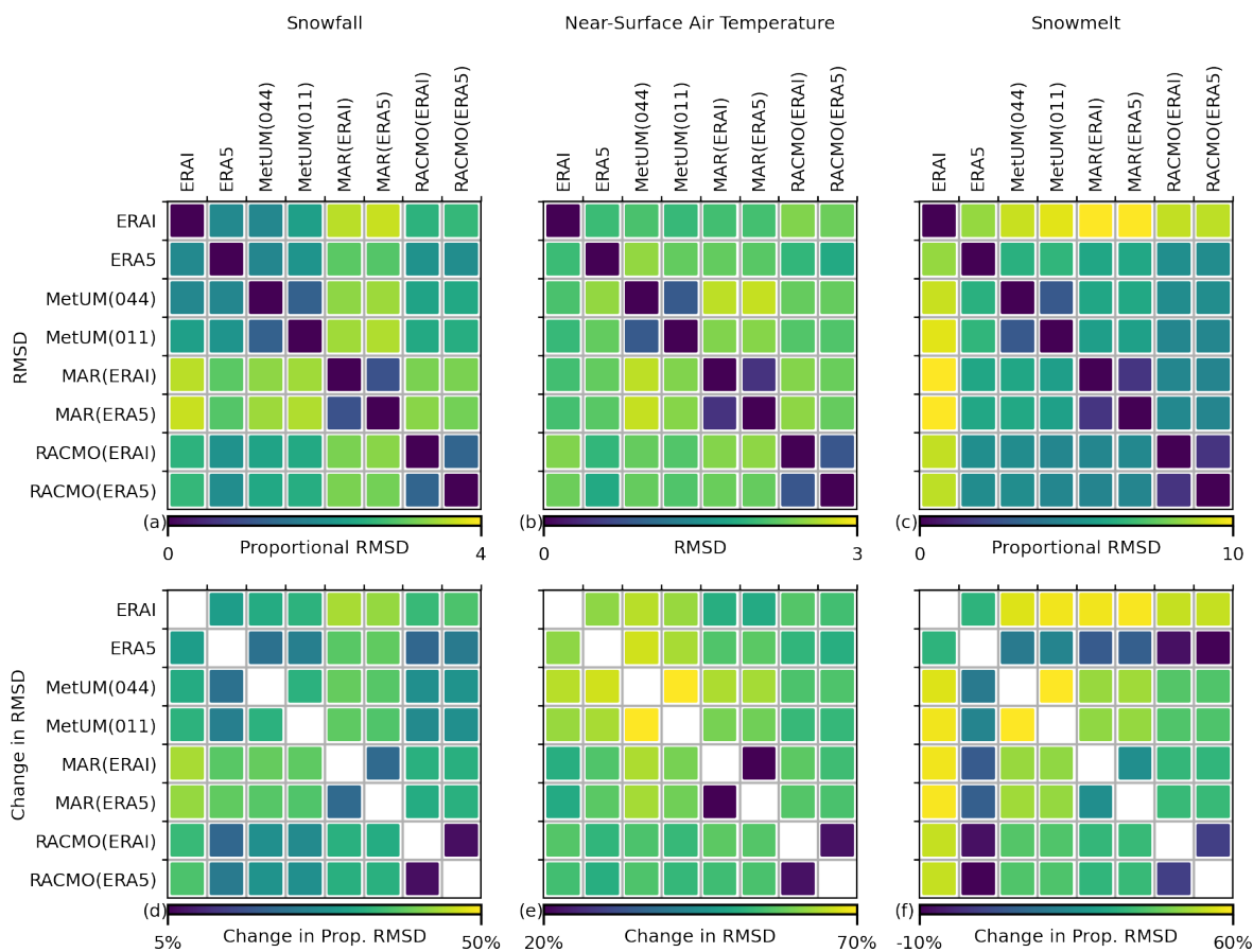
Figure 7. The RMSD/proportional RMSD for snowfall (a), near-surface air temperature (b) and melt (c) between models averaged over the ice-sheet. After adjusting the mean and seasonal/residual standard deviations of all outputs to the ensemble average the percentage reduction in RMSD/proportional RMSD is plot for snowfall (d), near-surface air temperature (e) and melt (f).
