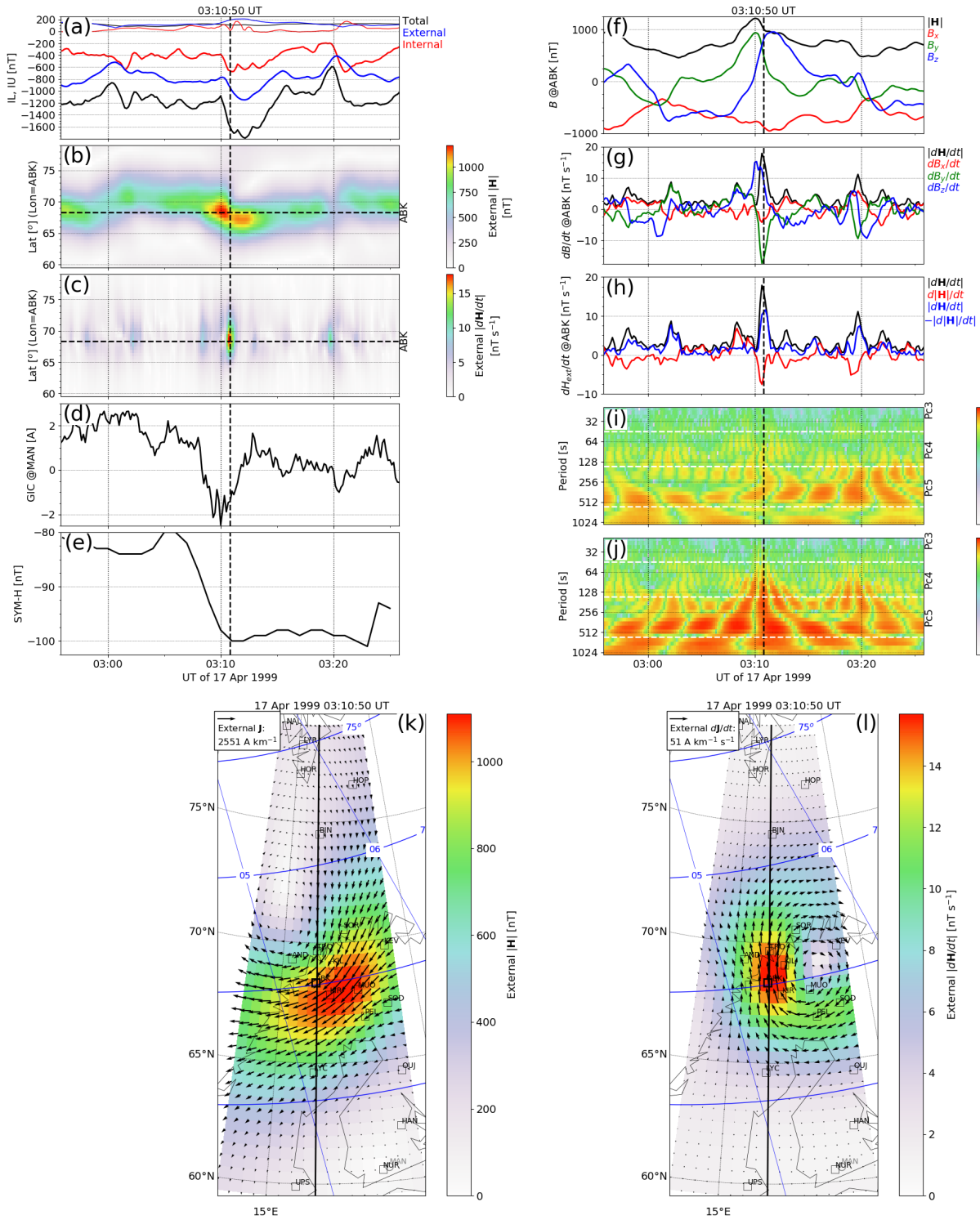
Figure 12. Data in a format similar to Fig. 5 \pm 15 min around the event on 17 Apr 1999 at 03:10:50 UT.
