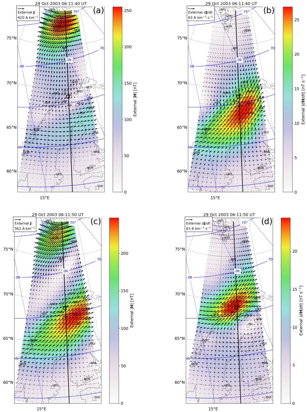
Figure 4. (a): External equivalent current density ( \mathbf{J} , arrows) and external horizontal magnetic field on ground ( |\Delta \mathbf{H}| , color) on 29 Oct 2003 at 06:11:40 UT when the largest external |d\mathbf{H}/dt| between 1994 and 2018 was measured at stations IVA, PEL, RVK, and DOB. (b): 10 s time derivative of external \mathbf{J} ( d\mathbf{J}/dt , arrows) and of external \Delta \mathbf{H} ( |d\mathbf{H}/dt| , color). (c)–(d): The same as (a)–(b), but at 06:10:50 UT, when the the largest external |d\mathbf{H}/dt| was measured at stations KEV, MAS, KIL, ABK, and MUO. In each panel, a black vertical line passing through the station KIL indicates the locations from which latitude profiles are extracted to create a time series representation of the parameters in Fig. 3.
