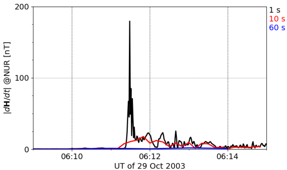
Figure 14. Time derivative of the total horizontal magnetic field ( |dH/dt| ) derived from 1 s, 10 s, and 1 min data at NUR on 29 October 2003 between 06:09:00 and 06:15:00 UT.
