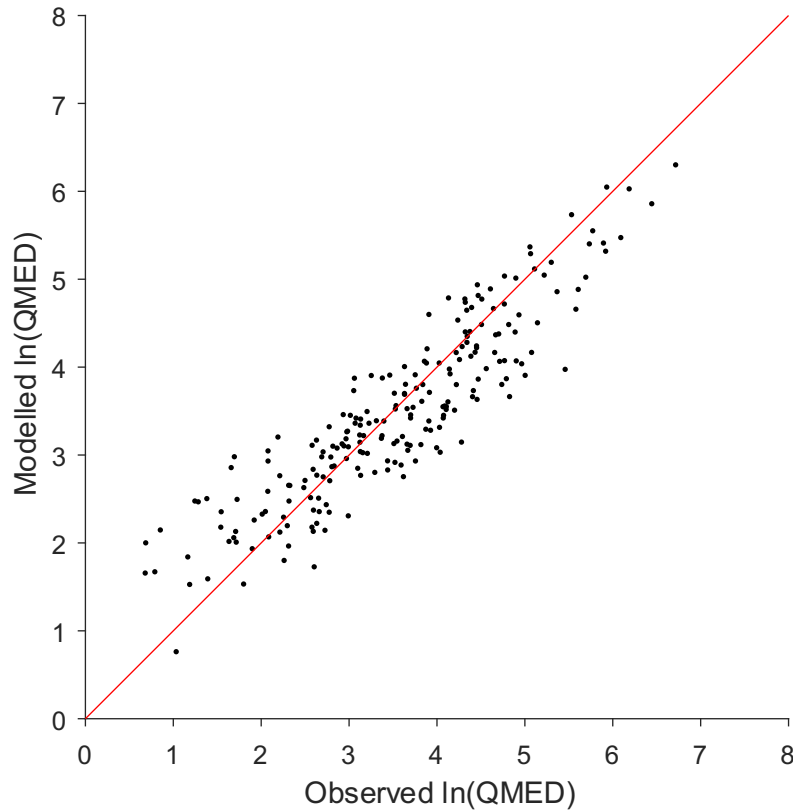
260 Figure S1: Plot of observed vs. modelled index flood (natural logarithm of QMED in \text{m}^3\text{s}^{-1} ).
