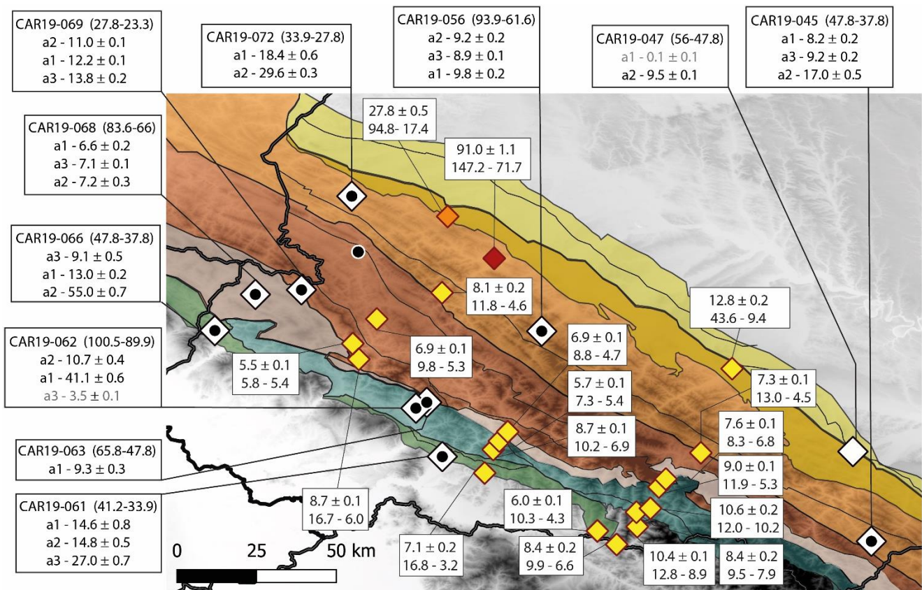
Figure 3: AFT data from this study shown as radial plots (centred on the central age, which is reported below the sample code as CA); individual single-grain ages in radial plots are coloured according to Dpar value. Grey band in radial plots indicates depositional age, dashed lines are different age populations (P1, P2, etc.); red dashed line is minimum age. Coloured circles on map show AFT central ages from previous studies (Nakapelyukh et al., 2017, 2018; Andreucci et al., 2013, 2015). Base map shows different nappes, with colour scheme as in Figure 1.
