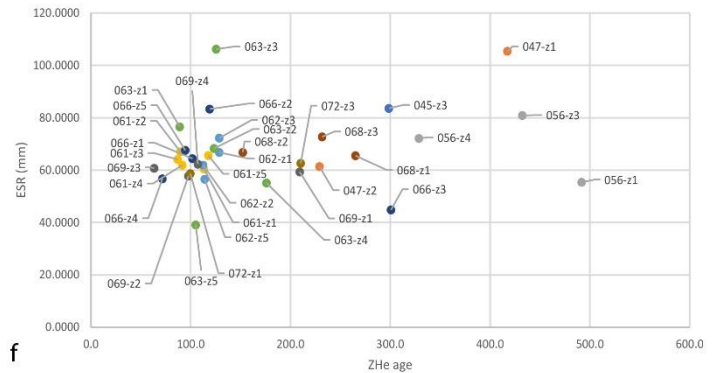
Figure A 1: Circle colour refer to a sample, the same colour code is applied for all graphs. a) Graphic of the AHe single grain age compared to the stratigraphic age. CAR19-066_a2 is the only non-reset grain. b) ZHe single grain age compared to the stratigraphic age. ZHe are non-reset and mark the sediment source age of exhumation. c) AHe single grain age as a function of eU (ppm) content. d) ZHe single grain age as a function of eU (ppm) content. e) AHe single-grain age as a function of ESR (equivalent sphere radius, in mm). f) ZHe single-grain age as a function of ESR.
