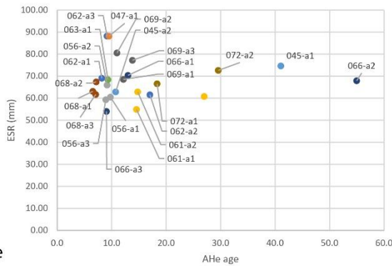
Figure A 1: Circle colour refer to a sample, the same colour code is applied for all graphs. a) Graphic of the AHe single grain age compared to the stratigraphic age. CAR19-066_a2 is the only non-reset grain. b) ZHe single grain age compared to the stratigraphic age. ZHe are non-reset and mark the sediment source age of exhumation. c) AHe single grain age as a function of eU (ppm) content. d) ZHe single grain age as a function of eU (ppm) content. e) AHe single-grain age as a function of ESR (equivalent sphere radius, in mm). f) ZHe single-grain age as a function of ESR.
