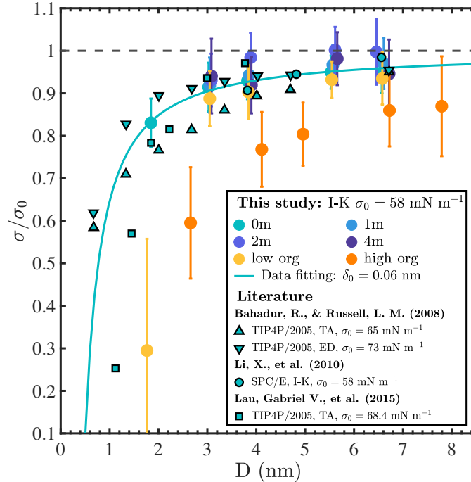
Figure 4. Normalized surface tension ( \sigma/\sigma_0 ) of droplets as a function of droplet diameter ( D ). Colored circles show results obtained in this study using the SPC/E water model and the Irving-Kirkwood (I-K) pressure tensor method; symbols with black edge show previous MD simulation results obtained for pure water droplets at ambient temperature using the TIP4P/2005 or SPC/E water models and the test-area (TA), energy difference (ED) or Irving-Kirkwood (I-K) methods (Bahadur and Russell, 2008; Li et al., 2010; Lau et al., 2015); the light blue solid line shows a fit of our 0 m surface tension data to the second-order Helfrich expansion, which yields the Tolman length \delta_0 = 0.06 nm.
