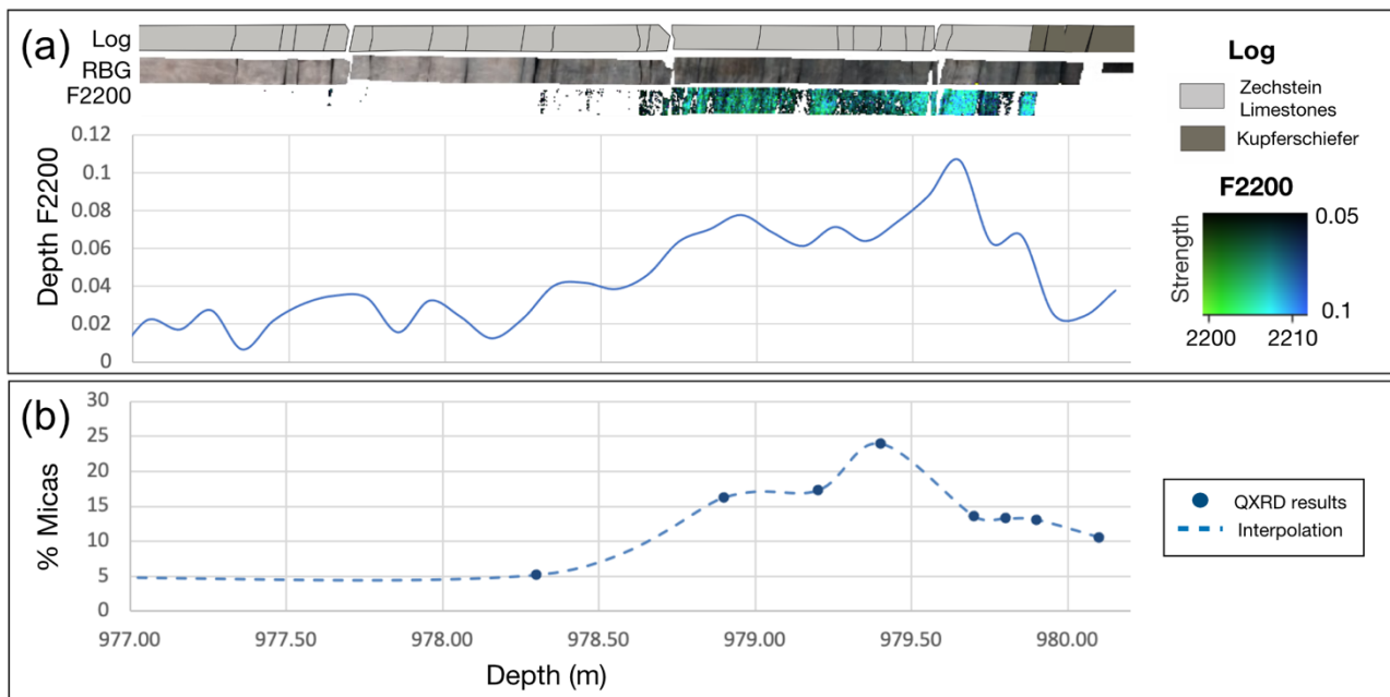
365 Figure 10. Distribution of the mica/clay-related absorption feature in the Kupferschiefer cores. (A) Log, RGB and F2200 map in the limestone and Kupferschiefer of drill core 131 and (B) results of QXRD for micas (from Kehrner, 2016).
