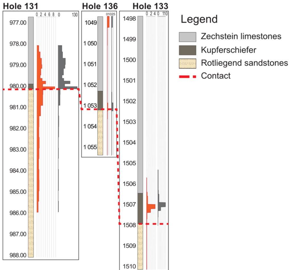
155 Figure 3. Lithology, copper (red in wt.%) and silver (grey in g/t) grades in the drill cores available for this study.
