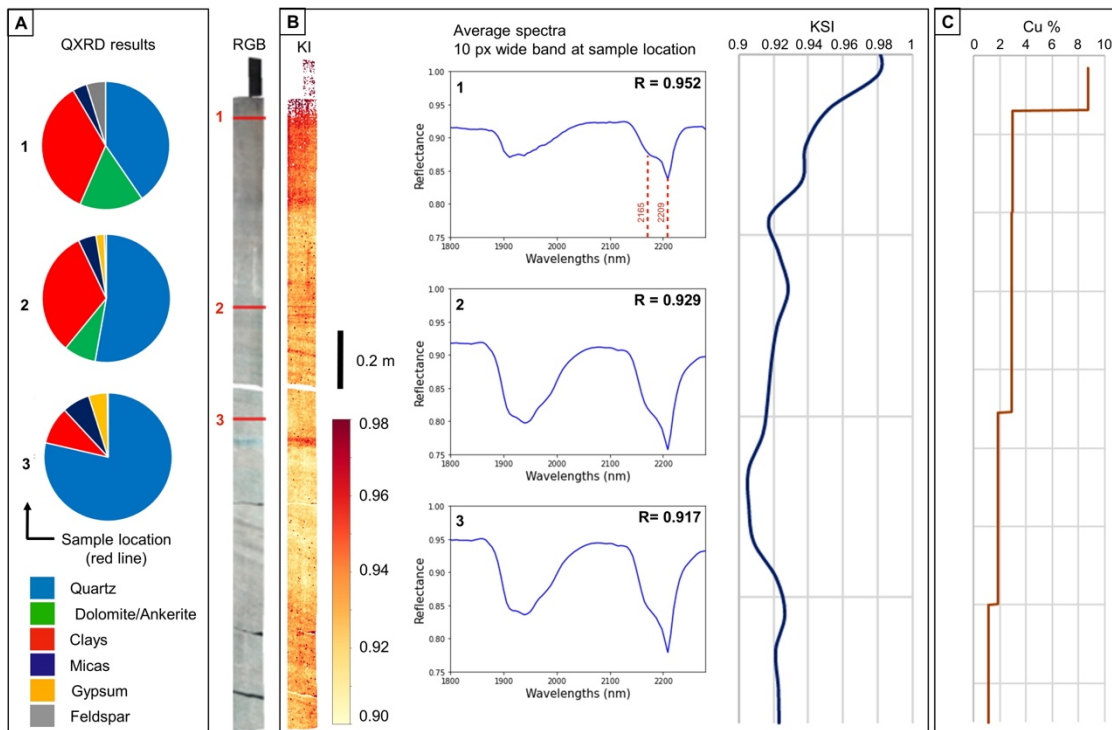
380 Figure 11. (A) QXRD results (Kehrer, 2016) for 3 samples at various depths in drill core 131 (1, 2 and 3); (B) KI map sandstones and organic-rich shales; average spectra in a 10 pixels wide band ( \approx 1 cm) at QXRD samples location; KI average along the core and (C) copper grade.
