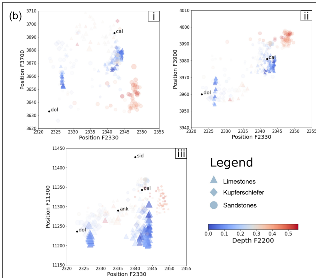
Figure 6. Example spectra (A) showing the dominant carbonate absorption positions in the SWIR-MWIR-LWIR spectral range. The 10-cm averaged position of these features (i. F3700; ii. F3900; iii. F11300) are plotted in (B) using the F2330 feature as a reference. Size is proportional to the depth of the feature on the y-axis and transparency to the depth of the F2330 feature. The colour indicates the depth of the F2200 feature and serves as a proxy for clay mineral abundance. Black points (cal=calcite; dol=dolomite; sid=siderite; ank=ankerite) show reference positions from the USGS spectral library (Kokaly et al., 2017) and Green and Schodlok (2016) for F11300.
