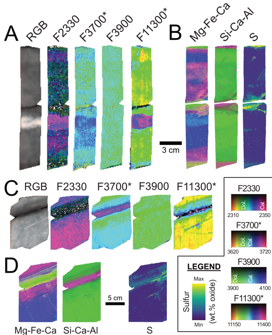
305 Figure 8. Comparison of hyperspectral imaging (HSI) data and spatially-resolved chemical ( \mu XRF) data for validation. (A) HSI data for sample 1 from drill core 136, 1048.7–1048.85 m depth, and (B) corresponding \mu XRF data displayed as false-colour RGB images. (C) HSI data for sample 2 from drill core 136, 1049.4–1049.5 m depth, and (D) corresponding \mu XRF data.
