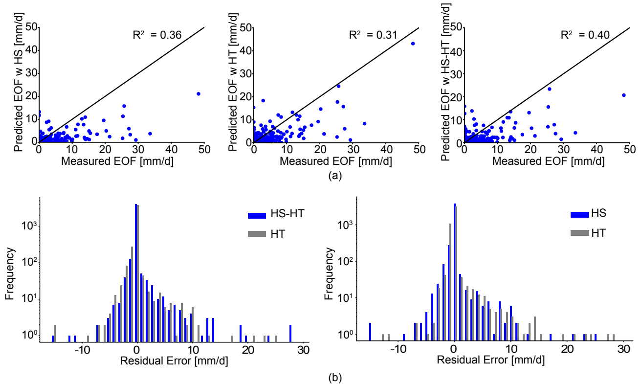
Figure 6. (a) Comparison of the observations with the predictions of daily EOF runoff for the Maumee domain by the XGBoost models trained using the HS, HT, and HS-HT [.. 17 ] approaches, respectively. (b) Comparison of residual errors between the observations and the predictions of daily EOF runoff for the Maumee domain by the XGBoost models trained using the HS-HT, HS, and HT [.. 18 ] approaches, respectively.
