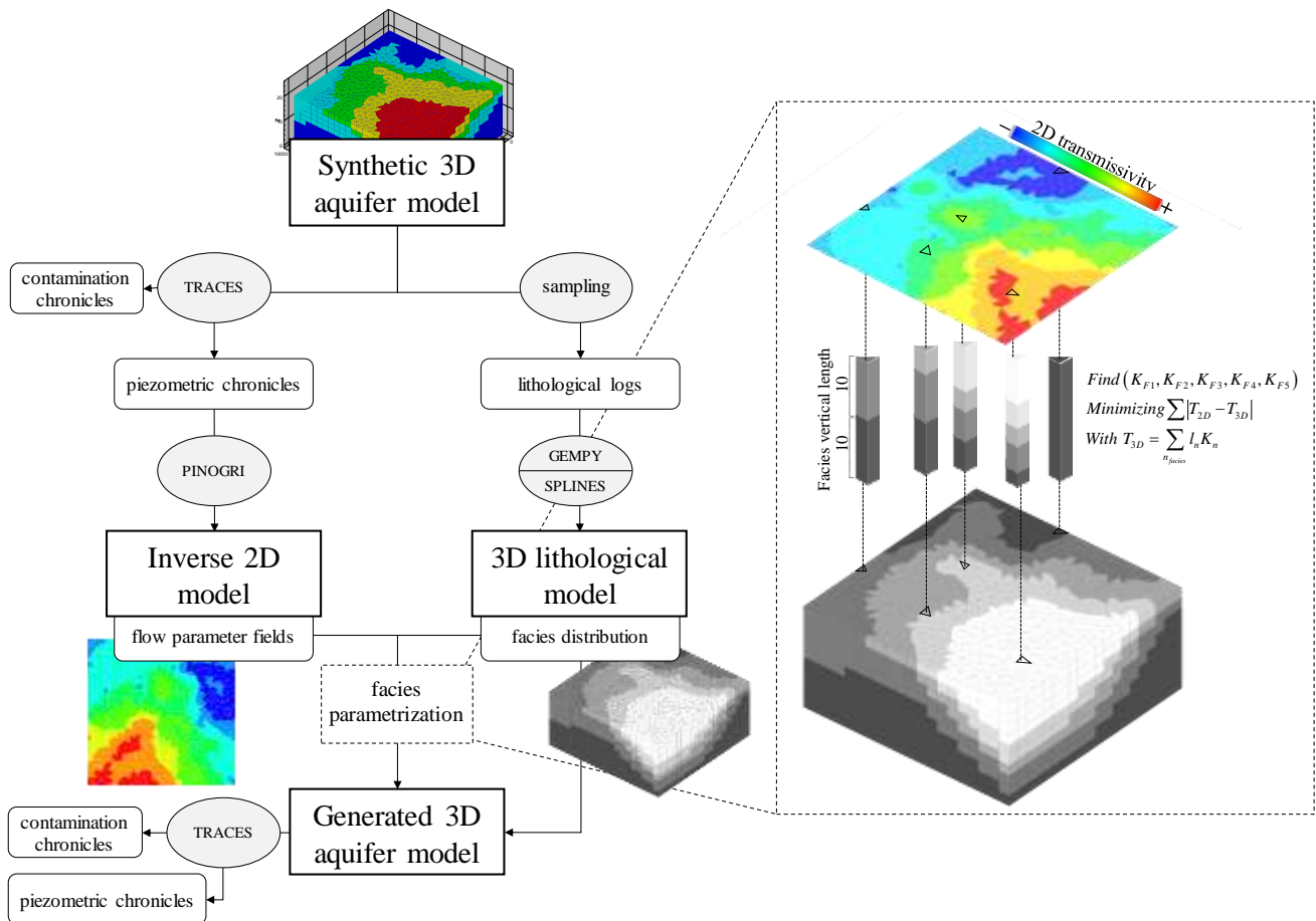
70 Figure 1: Methodology flowchart – TRACES: Transport of Radioactive Elements in Subsurface (Hoteit & Ackerer, 2004); PINOGRI: Parameter Inversion Numerically Optimized for Groundwater Issues (Rambourg et al., 2020); GEMPY: Open-source 3D geological modelling (de la Varga et al., 2019); SPLINES: QGIS/SAGA multilevel b spline interpolation (Lee et al., 1997).
