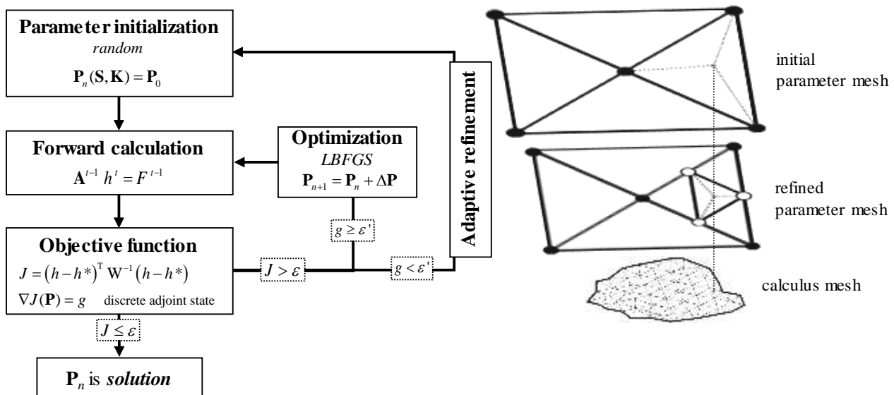
195 Figure 4: Inversion algorithm (adapted from Rambourg et al., 2020).
