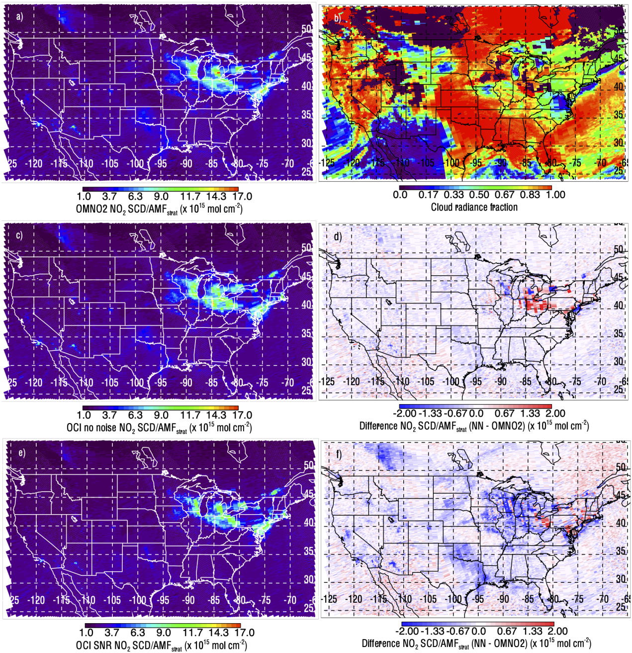
Figure 5. Data from 28 January 2005 (day not used in fitting) for NO 2 SCDs normalized by the stratospheric air mass factor (normalized SCD); (a) Normalized SCDs from OMI OMNO2 algorithm; (b) Cloud radiance fraction for the NO 2 fitting window from OMNO2; (c), (e): Normalized SCDs from the NN algorithm evaluated at each OMI pixel using OCI spectral characteristics and fitting window of 355–500 nm with no noise and with the SNR model of Fig. 1(b), respectively; (d), (f): corresponding differences with respect to OMNO2 normalized SCDs for the results shown in (c) and (e), respectively.
