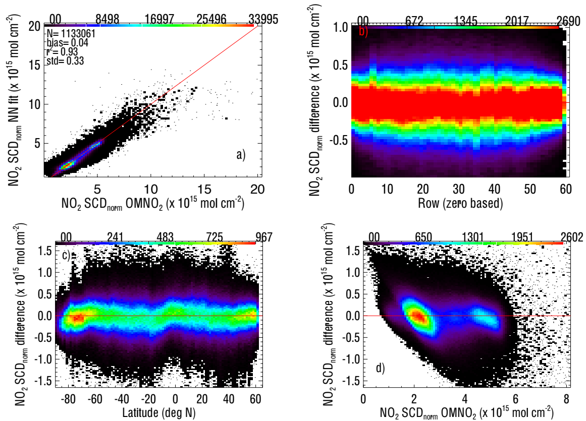
Figure 4. Global data from 28 February 2005 from a training using where each point represents the result that would be obtained using the OCI spectral characteristics and SNR from Fig. 1b multiplied by 2 with fitting window 355-500 nm; a) Density distribution (numbers along the top) of \text{NO}_2 target OMNO 2 SCD (all results here are normalized (as indicated by the norm subscript) with respect to the stratospheric air mass factor) versus those from the NN training with statistics include standard deviation of the difference (std), fraction of variance explained ( r^2 ), and mean of difference between NN and target (bias); b-d) density distribution of the \text{NO}_2 SCD difference (NN SCD - OMNO 2 SCD) as a function of OMI row number, latitude, and \text{NO}_2 SCD, respectively.
