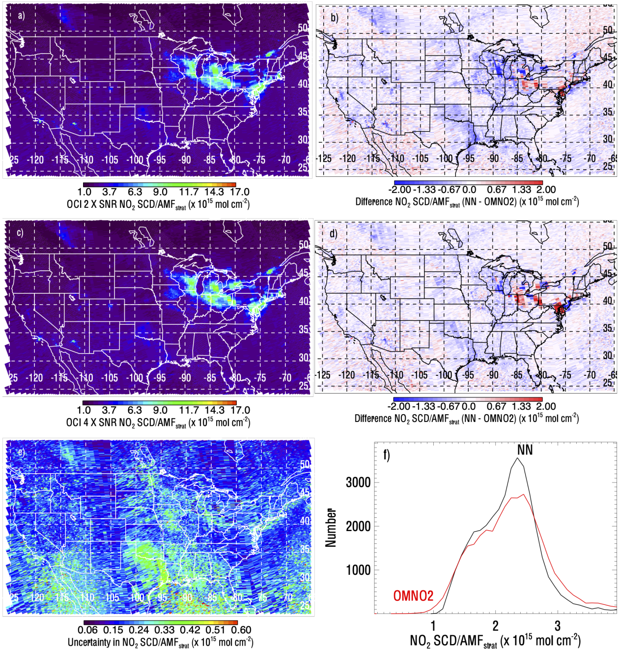
Figure 6. Similar to Fig. 5 showing data from 28 January 2005 (day not used in fitting): (a), (c) \text{NO}_2 SCDs normalized by the stratospheric air mass factor (normalized SCD) and for NN algorithms trained on data sets using OCI spectral characteristics and fitting window of 355–500 nm, evaluated at each OMI pixel using 2\times and 4\times the SNR from the model of Fig. 1(b), respectively; (b), (d): corresponding differences with respect to OMNO2 normalized SCDs shown in Fig. 5(a); (e) fitting uncertainties in normalized SCD from OMNO2; (f) histograms of the lower end of normalized SCDs from OMNO2 and the NN model with 2\times the OCI SNR.
