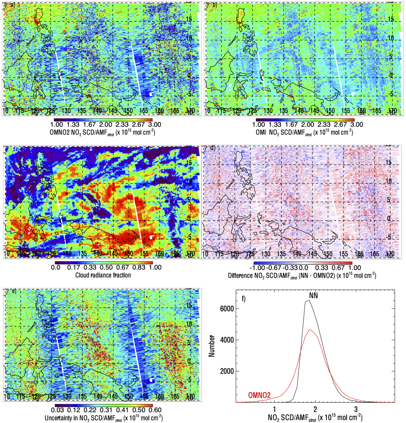
Figure 9. Normalized NO 2 SCDs from 28 January 2005 over the tropical Pacific region from (a) OMNO2 and (b) NN applied at OMI spectral resolution and with the OMNO2 fitting window 402–465 nm; (c) cloud radiance fraction; (d) difference between the NN and OMNO2 normalized SCDs; (e) normalized SCD fitting uncertainties from OMNO2; (f) histograms of the normalized SCDs corresponding to the area shown in (a).
