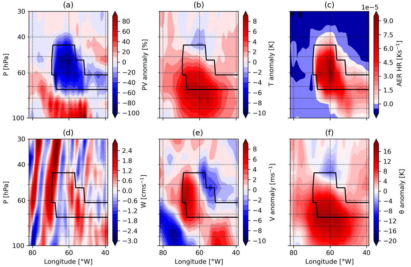
Figure 6. Same as Fig.5 but for a fixed latitude ( 36^\circ N). Panel (e) contains the meridional velocity anomaly.
