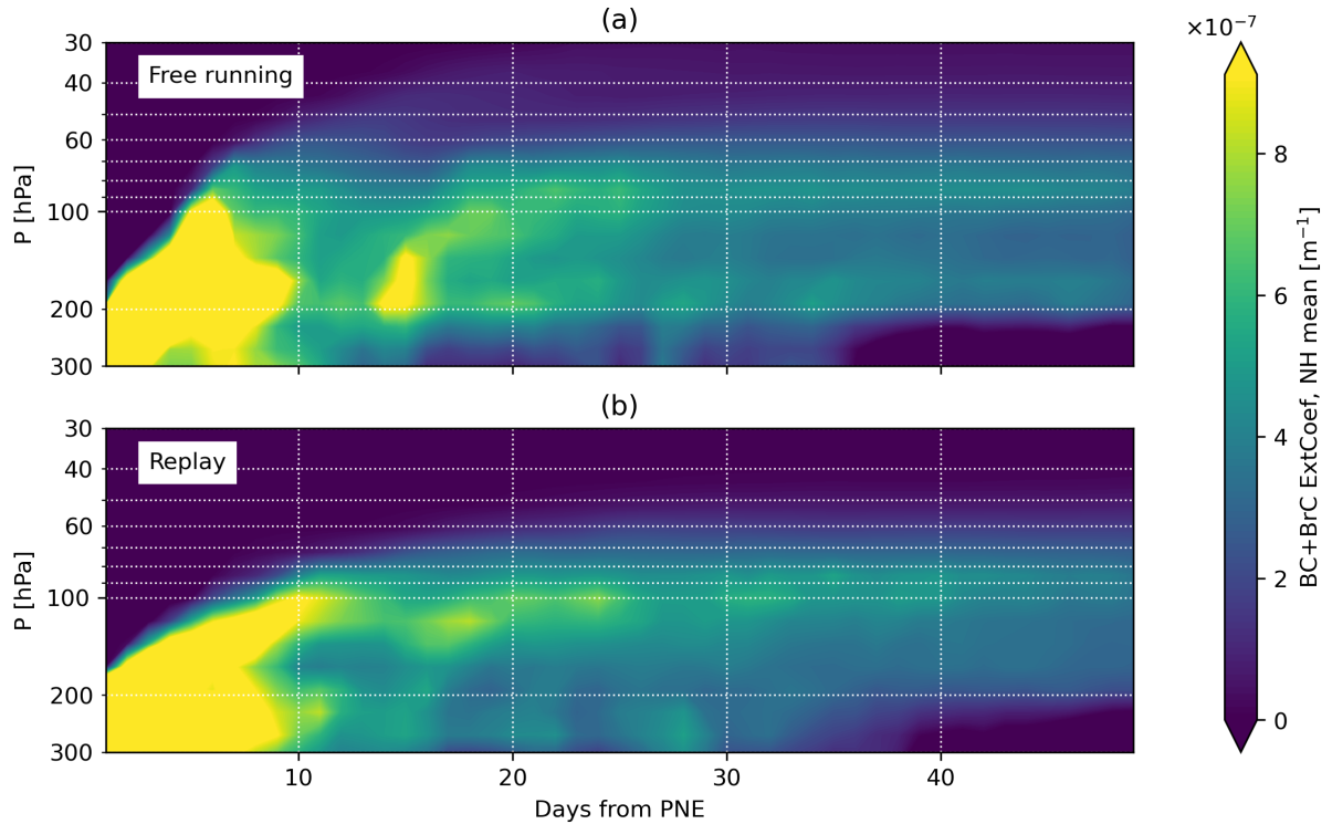
Figure A2. Time evolution of the horizontal average over the northern hemisphere of the 550 nm extinction coefficient of carbonaceous aerosols.
