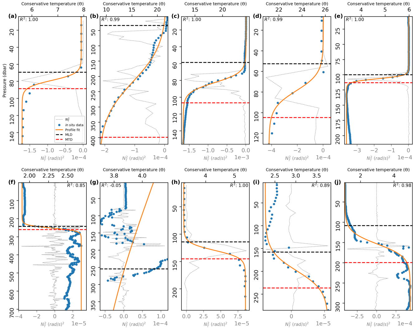
Figure 1. Location of the MTD and the MLD in temperature profiles. (a) 52.95^{\circ}S and 90.05^{\circ}W on 01/23/2003. (b) 60.00^{\circ}S and 116.86^{\circ}W on 08/12/2015. (c) 25.13^{\circ}S and 93.47^{\circ}W on 01/12/2013. (d) 55.42^{\circ}S and 162.63^{\circ}W on 08/12/2020. (e) 1.90^{\circ}S and 126.07^{\circ}W on 08/25/2013. (f) 63.23^{\circ}N and 54.20^{\circ}W on 02/08/2010. (g) 20.02^{\circ}N and 41.14^{\circ}W on 12/15/2015. (h) 56.07^{\circ}N and 174.91^{\circ}W on 02/20/2014. (i) 49.00^{\circ}N and 174.69^{\circ}W on 12/13/2017. (j) 61.84^{\circ}N and 54.27^{\circ}W on 02/01/2016. Goodness of fit is shown at the top of each profile with R^2
