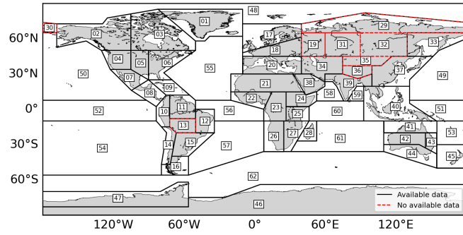
Figure 4. Reference regions of AR6-WGI. The regions used for comparison are those delimited in black.
