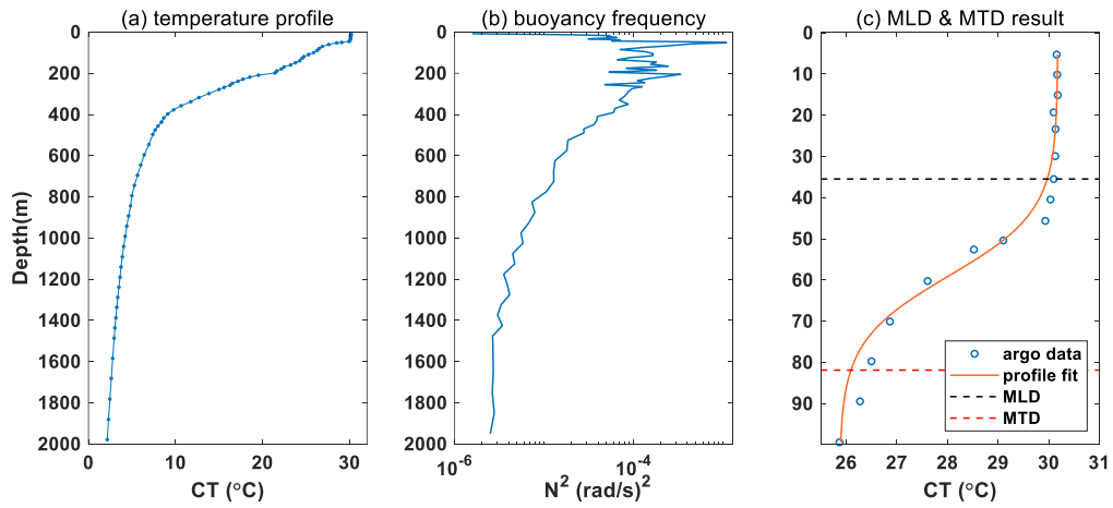
Figure. Example ARGO data of no. 2902688_104 (date: 2019/07/26, position: 127.98°E, 15.65°N), (a) conservative temperature, (b) buoyancy frequency profile and (c) MLD and MTD calculated by the provided code.
