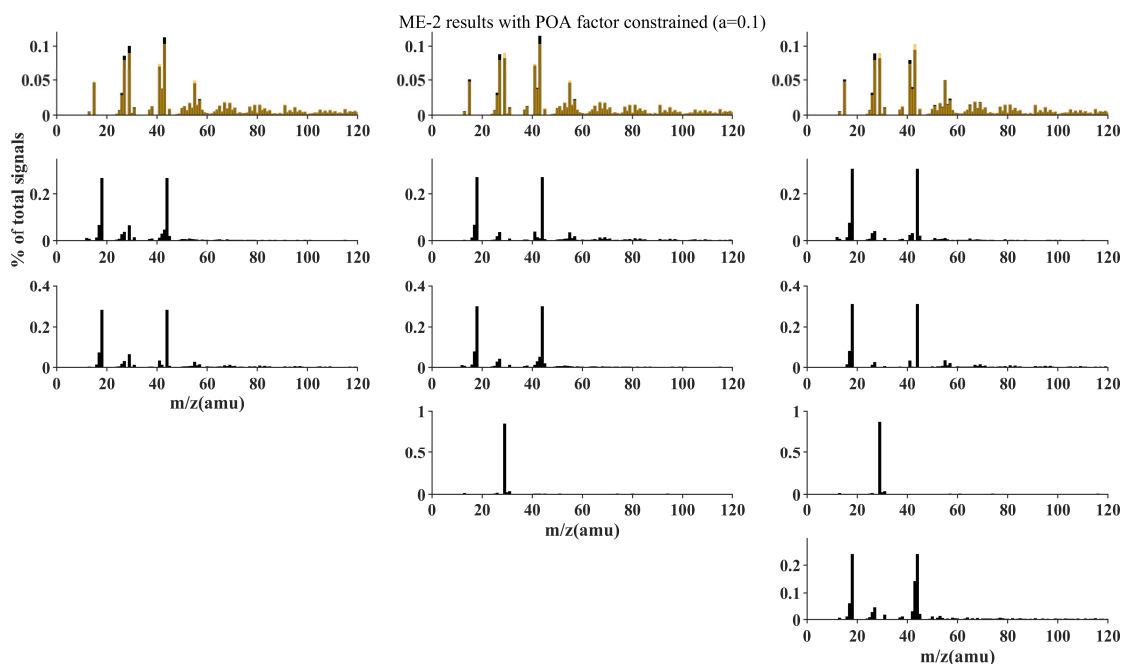
Figure AR7: Mass spectra of 3-5 factor solution from ME-2 analysis ( a=0.1 ) with POA factor constrained for autumn. Yellow bar stands for priori POA factor mass spectra from unconstrained 2-factor solution.
