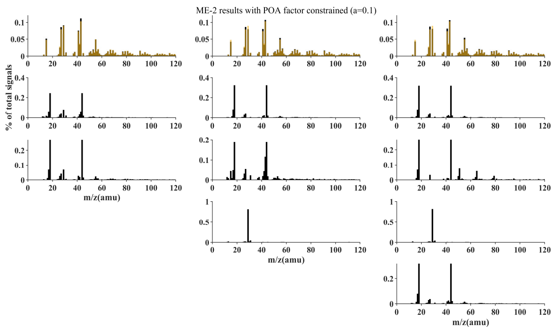
Figure AR6: Mass spectra of 3-5 factor solution from ME-2 analysis ( a=0.1 ) with POA factor constrained for summer. Yellow bar stands for priori POA factor mass spectra from unconstrained 2-factor solution.
