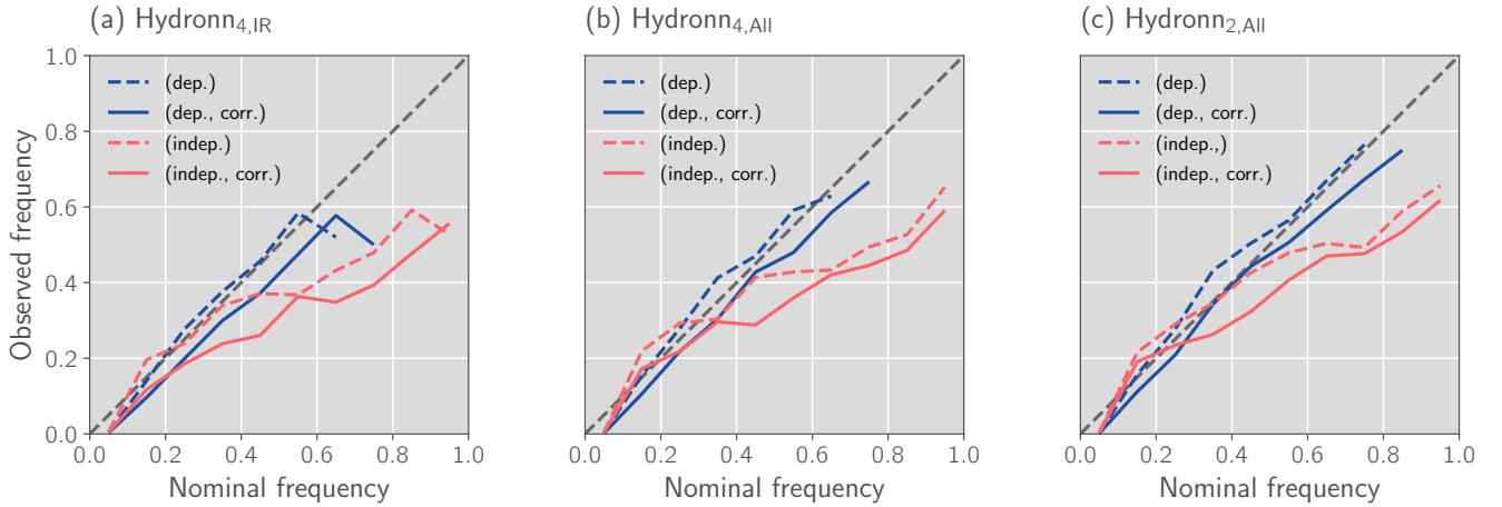
Figure 17. Calibration of the probabilistic precipitation event detection for precipitation exceeding 5 \text{ mm h}^{-1}
