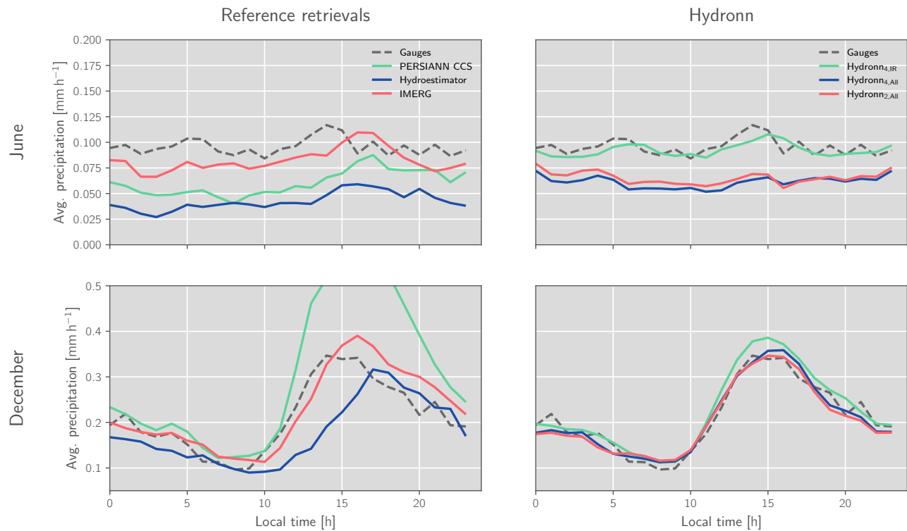
Figure 13. Measured and retrieved daily cycles of precipitation. The first column displays the daily cycles retrieved by the three reference retrievals (solid lines) and the gauge measurements (dashed line) for reference. The second column corresponding diurnal cycles for the three Hydronn configurations. The first row shows the results for June 2020 and the second results for December 2020.
