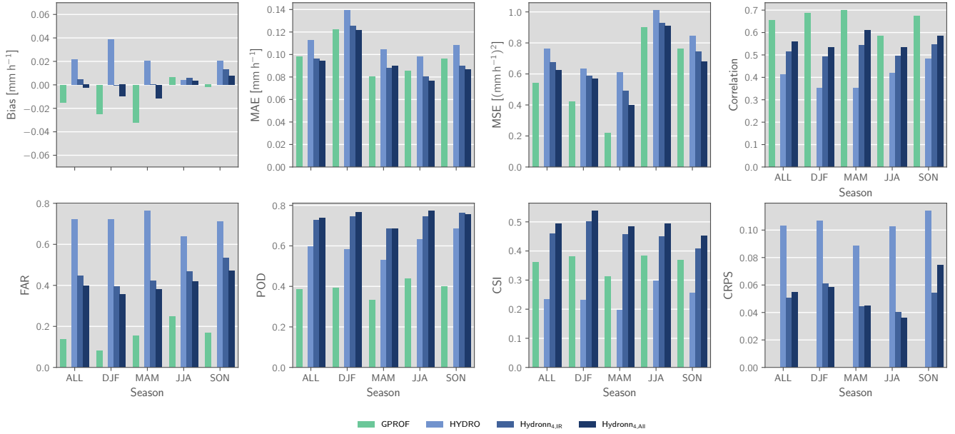
Figure 10. Retrieval accuracy with respect to GPM CMB for overpasses on the 1st, 6th, 11th 16th 21st and 26th day of each month of 2020 over the domain R2. Each panel shows the average of a metric over the full year as well as its seasonal variability.
