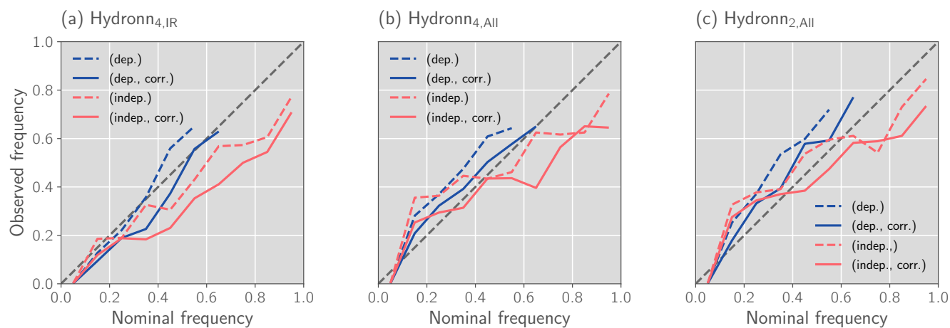
Figure A3. Like Fig. 17 but for June 2020.
