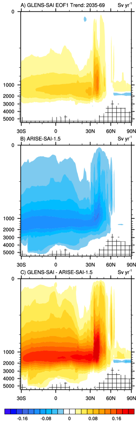
Figure A6: Latitude-depth structure of ensemble-mean changes in the leading mode of the overturning circulation scaled by the linear trend in PC1 from 2035 to 2069 for (a) GLENS-SAI, (b) ARISE-SAI-1.5, and (c) their difference.
