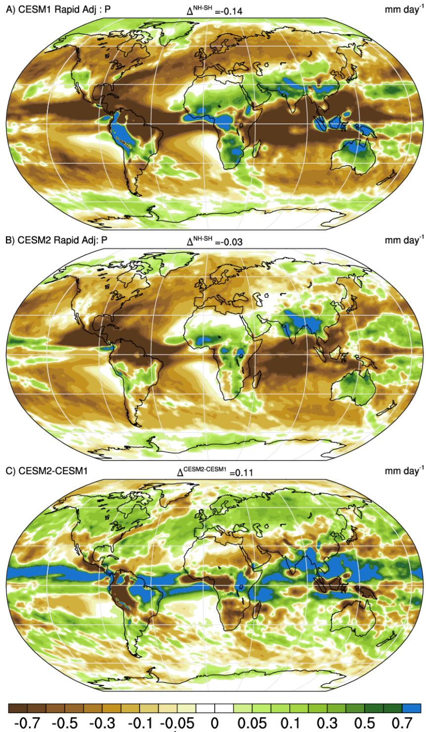
400 Figure A8. Rapid adjustments of precipitation (mm day -1 ) to CO 2 based on 4xAMIP-AMIP simulation differences in (a) CESM1, (b) CESM2, and (c) their difference (b-a).
