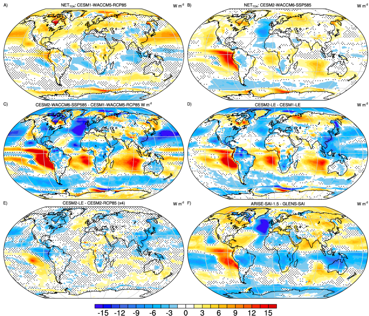
360 Figure A1. Normalized response in net incoming top-of-atmosphere radiative flux (RTMT) estimated from the change between 2020-39 and 2050-69 per degree global warming for unmitigated (a) CESM1-WACCM5-RCP85 and (b) CESM2-WACCM6-SSP585 simulations, and (c) their difference (b-a). Also shown is (d) the analogous difference for the CESM1-LE and CESM2-LE and (e) the CESM2-RCP85 and CESM2-LE (scaled by 4). The difference between the geoengineered climate states in ARISE-SAI-1.5 and GLENS-SAI is shown in (f). Units for all panels are W m -2 K -1 , except in (f) where units are W m -2 , and stippled regions indicate 365 differences that are less than twice the ensemble standard error.
