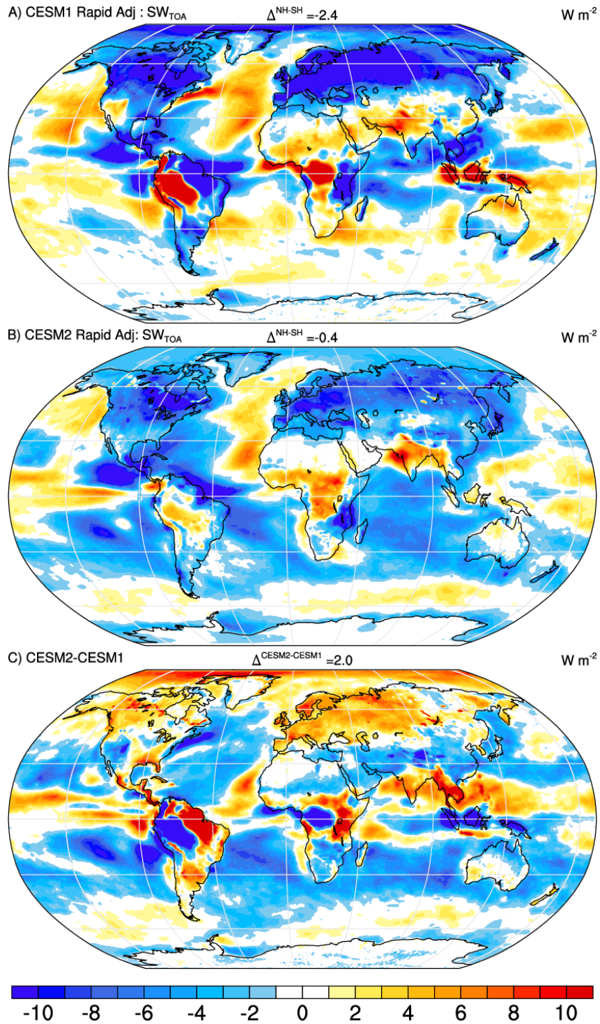
Figure 4: Estimates of the rapid adjustment of TOA net absorbed SW flux to CO_2 for CESM1 (a), CESM2 (b), and their difference (c) based on estimates from 4\times CO_2 AMIP and AMIP simulations. Differences in the hemispheric means are shown in panel titles. All units are W m^{-2} .
