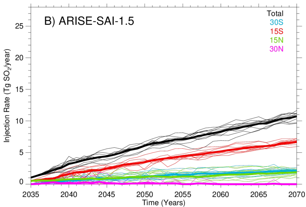
Figure 1: Evolution of yearly sulfur dioxide injections ( \text{Tg SO}_2 \text{ yr}^{-1} ) over time at the four injection latitudes for (a) GLENS-SAI and (b) ARISE-SAI-1.5 from 2035 to 2070.
