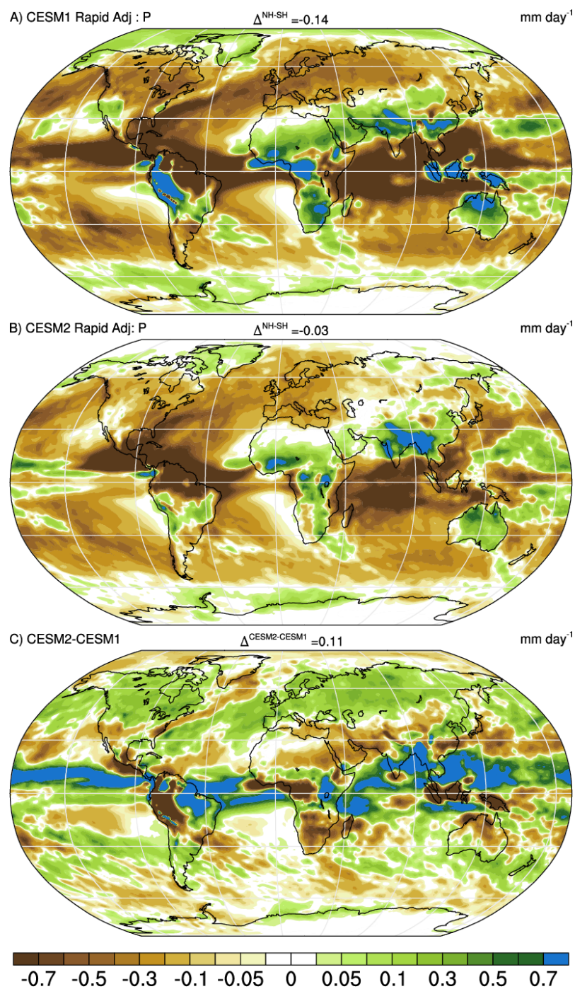
340 Figure 6: The rapid adjustment of total precipitation to CO 2 quadrupling for CESM1 (a), CESM2 (b), and their difference (c) based on estimates from 4xCO 2 AMIP and AMIP simulations. Differences in the hemispheric means are shown in panel titles. All units are mm day -1 .
