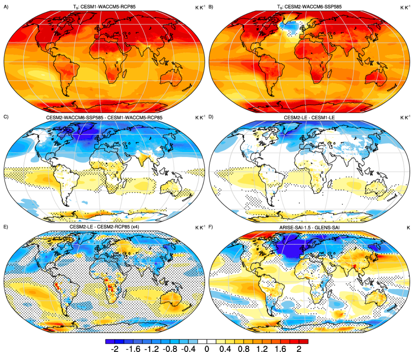
315 Figure 2: Normalized response in near surface air temperature ( T_s ) estimated from the change between 2020–2039 and 2050–2069 per degree global warming for unmitigated (a) CESM1-WACCM5-RCP85 and (b) CESM2-WACCM6-SSP585 simulations, and (c) their difference (b-a). Also shown is (d) the analogous difference for the CESM1-LE and CESM2-LE and (e) the CESM2-RCP85 and CESM2-LE (multiplied by 4 for clarity using a single colorbar). The difference between the geoengineered climate states in 320 ARISE-SAI-1.5 and GLENS-SAI is shown in (f). Units for all panels are K K^{-1} , except in (f) where units are K , and stippled regions indicate differences that are less than twice the ensemble standard error.
