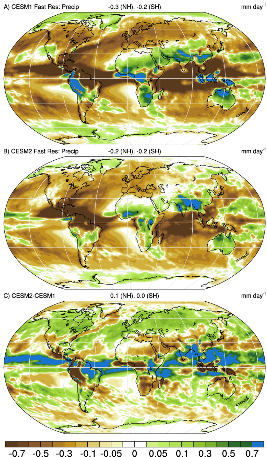
360 Figure A7. Rapid adjustments of precipitation (mm day -1 ) to CO 2 based on 4xAMIP-AMIP simulation differences in (a) CESM1, (b) CESM2, and (c) their difference (b-a).
