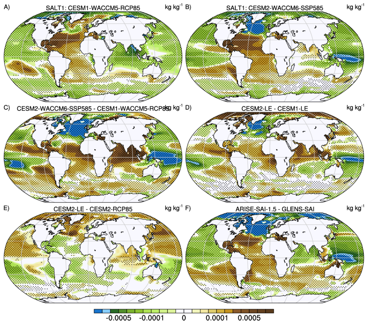
355 Figure A6. Response in surface salinity estimated from the change between 2020-39 and 2050-69 for unmitigated (a) CESM1-WACCM5-RCP85 and (b) CESM2-WACCM6-SSP585 simulations, and their difference (c). Also shown is the analogous difference for (d) the CESM1-LE and CESM2-LE (d) and (e) the CESM2-RCP85 and CESM2-LE. The difference between the geoengineered climate states in ARISE-SAI-1.5 and GLENS-SAI is shown in (f).
