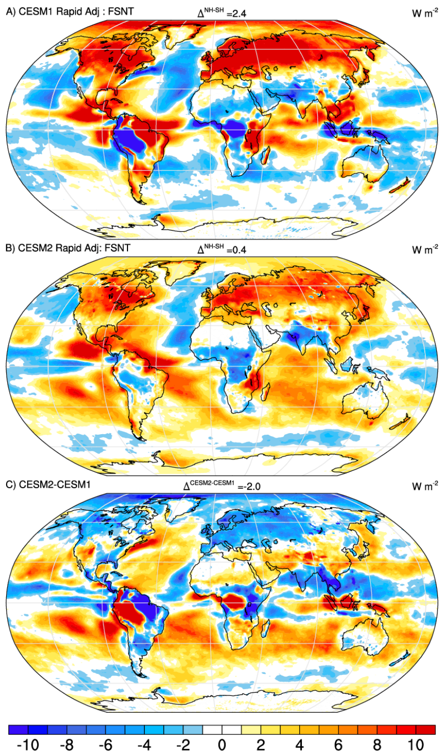
295 Figure 4: Estimates of the rapid adjustment of TOA net SW flux to CO 2 for CESM1 (a), CESM2 (b), and their difference (c) based on estimates from 4xCO 2 AMIP and AMIP simulations. Differences in the hemispheric means are shown in panel titles. All units are W m -2 .
