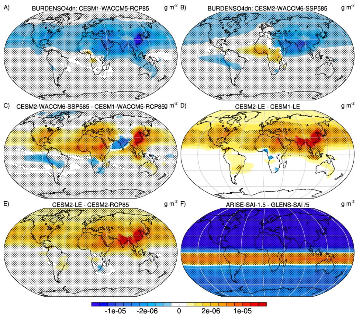
310 Figure 7: Absolute change in sulfate aerosol burdens (BURDENSO4dn) estimated from the difference between 2020-39 and 2050-69 for unmitigated (a) CESM1-WACCM5-RCP85 and (b) CESM2-WACCM6-SSP585 simulations, and (c) their difference (b-a). Also shown is (d) the analogous difference for the CESM1-LE and CESM2-LE and (e) the CESM2-RCP85 and CESM2-LE. The difference between the geoengineered climate states in ARISE-SAI-1.5 and GLENS-SAI is shown in (f). Units for all panels are \text{g m}^{-2} and stippled regions indicate differences that exceed twice the ensemble standard error. The difference field in (f) is scaled by 1/5^{\text{th}} .
