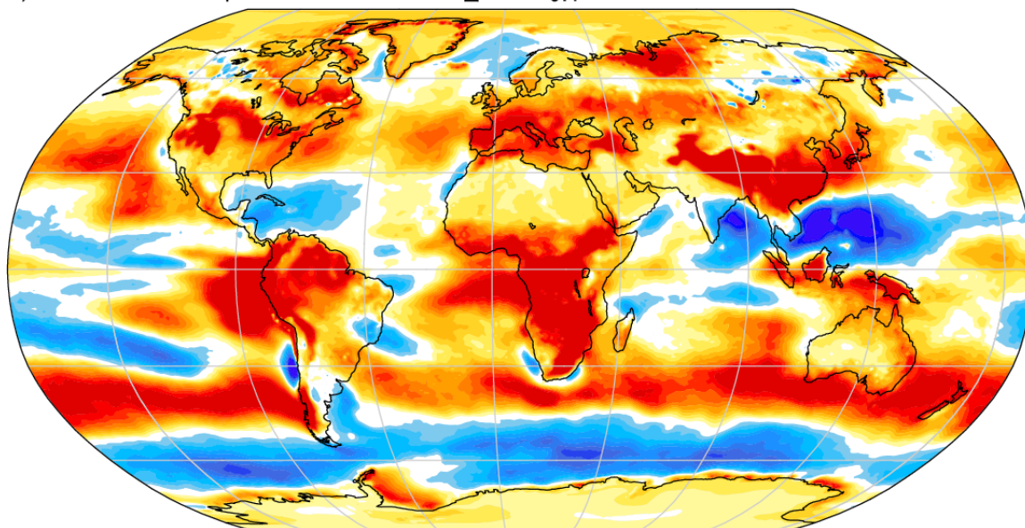
B) CESM2 Slow Response: FSNT \Delta^{NH-SH} = -0.1
