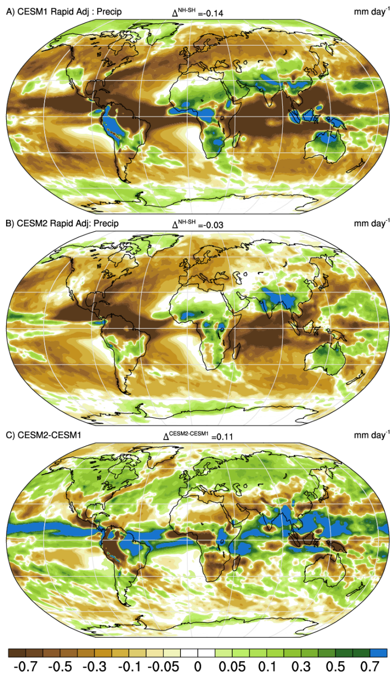
305 Figure 6: The rapid adjustment of total precipitation to CO 2 quadrupling for CESM1 (a), CESM2 (b), and their difference (c) based on estimates from 4xCO 2 AMIP and AMIP simulations. Differences in the hemispheric means are shown in panel titles. All units are mm day -1 .
