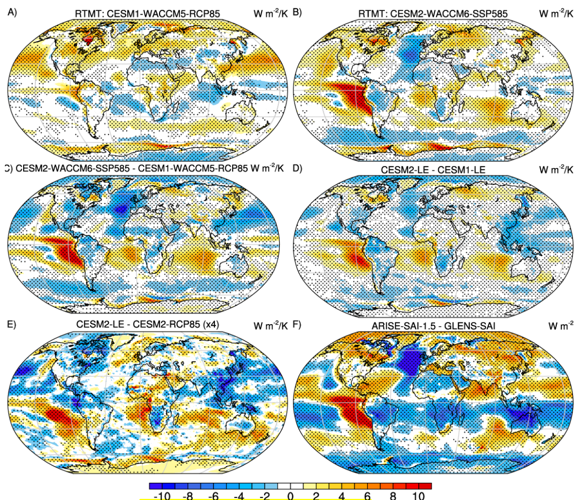
325 Figure A1. Normalized response in net top-of-atmosphere radiative flux (RTMT) estimated from the change between 2020-39 and 2050-69 per degree global warming for unmitigated (a) CESM1-WACCM5-RCP85 and (b) CESM2-WACCM6-SSP585 simulations, and (c) their difference (b-a). Also shown is (d) the analogous difference for the CESM1-LE and CESM2-LE and (e) the CESM2-RCP85 and CESM2-LE (scaled by 4). The difference between the geoen지니어ed climate states in ARISE-SAI-1.5 and GLENS-SAI is shown in (f). Units for all panels are W m^{-2} K^{-1} , except in (f) where units are W m^{-2} , and stippled regions indicate differences that exceed twice the ensemble standard error.
