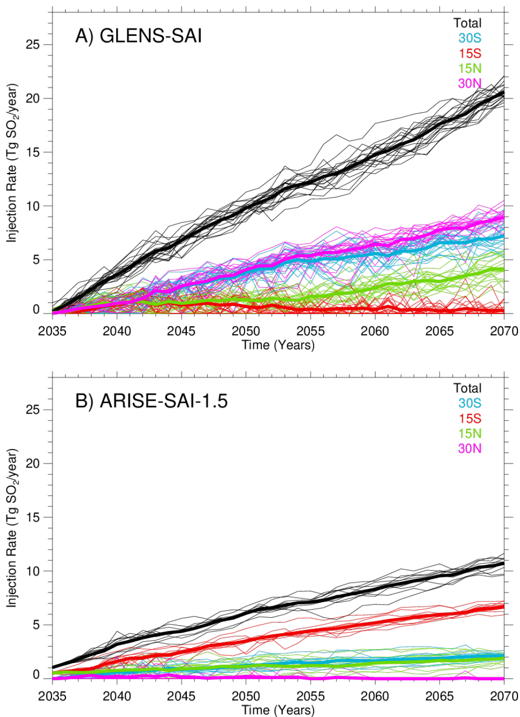
Figure 1: Evolution of yearly sulfur dioxide injections (Tg SO 2 yr -1 ) over time at the four injection latitudes for (a) GLENS-SAI and (b) ARISE-SAI-1.5 from 2035 to 2070.
