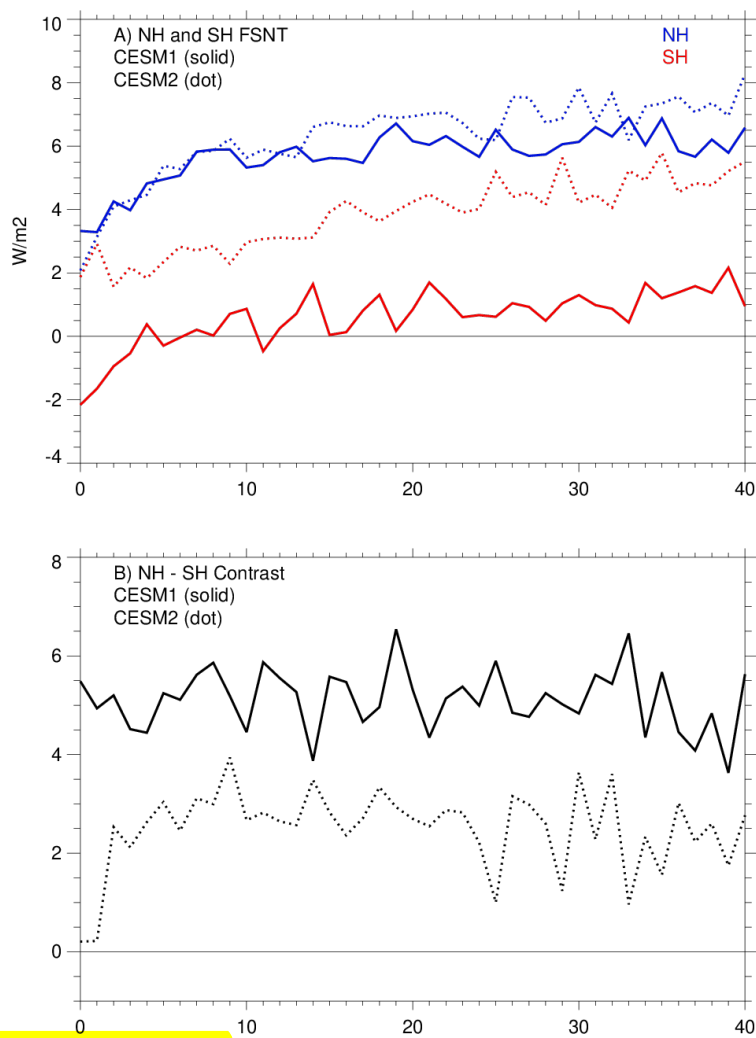
350 Figure A5. Timeseries of hemispheric mean fluxes (a) and their differences (b) in abrupt4xCO 2 simulations.
