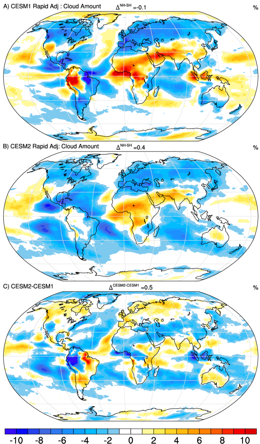
Figure A3. Rapid adjustments of cloud amount (%) to CO 2 based on 4xCO 2 AMIP-AMIP simulation differences in (a) CESM1, (b) CESM2, and (c) their difference (b-a).
