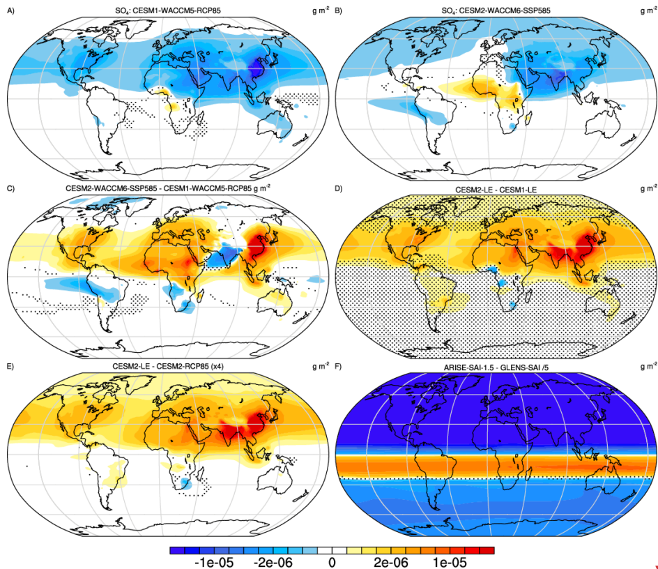
Figure 7: Absolute change in sulphate aerosol burdens ( \text{SO}_4 ) estimated from the difference between 2020-39 and 2050-69 for unmitigated (a) CESM1-WACCM5-RCP85 and (b) CESM2-WACCM6-SSP585 simulations, and (c) their difference (b-a). Also shown is (d) the analogous difference for the CESM1-LE and CESM2-LE and (e) the CESM2-RCP85 and CESM2-LE. The difference between the geoengineered climate states in ARISE-SAI-1.5 and GLENS-SAI is shown in (f). Units for all panels are \text{g m}^{-2} and stippled regions indicate differences that are less than twice the ensemble standard error. The difference field in (f) is scaled by 1/5^{\text{th}} .
