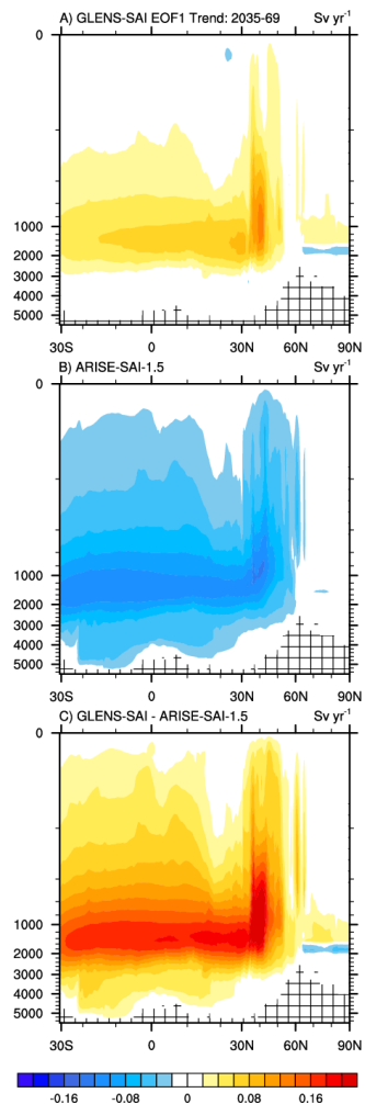
Figure A6: Latitude-depth structure of ensemble-mean changes in the leading mode of the overturning circulation* scaled by the linear trend in PC1 from 2035 to 2069 for (a) GLENS-SAI, (b) ARISE-SAI-1.5, and (c) their difference.
