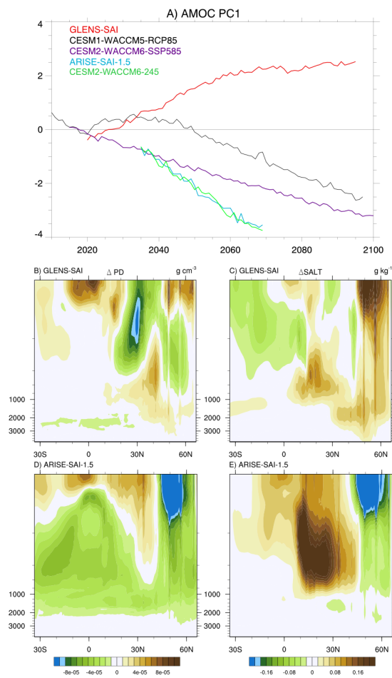
Figure 5: (a) Changes in the normalized leading principal component of the Atlantic Meridional Overturning Circulation, which is unitless , in unmitigated (CESM1-WACCM5-RCP85, CESM2-WACCM6-SSP245, CESM2-WACCM6-SSP585) and mitigated (GLENS-SAI, ARISE-SAI-1.5) experiments. Also shown are changes between 2020-2039 and 2050-2069 in the latitude-depth structure in the Atlantic Ocean of ocean potential density (PD, b, d, units of \text{g cm}^{-3} ) and salinity (SALT, c, e, units of \text{g kg}^{-1} ) for GLENS-SAI (b, c) and ARISE-SAI-1.5 (d, e), respectively.
