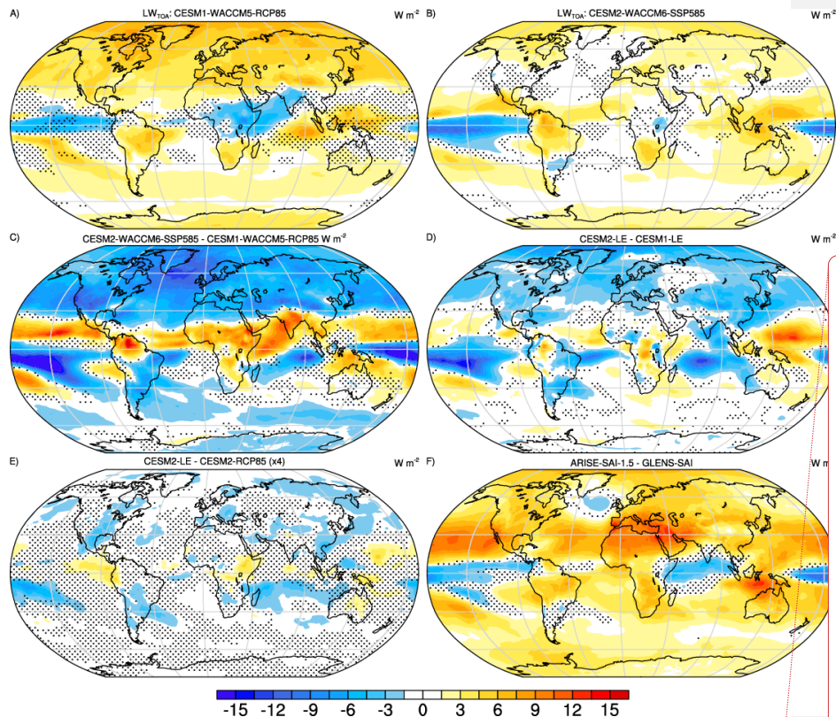
Figure A2. Normalized response in net outgoing top-of-atmosphere longwave flux ( LW_{TOA} ) per degree global warming estimated from the change between 2020-39 and 2050-69 for unmitigated (a) CESM1-WACCM5-RCP85 and (b) CESM2-WACCM6-SSP585 simulations, and (c) their difference (b-a). Also shown is (d) the analogous difference for the CESM1-LE and CESM2-LE and (e) the CESM2-RCP85 and CESM2-LE (scaled by 4). The difference between the geoengineered climate states in ARISE-SAI-1.5 and GLENS-SAI is shown in (f). Units for all panels are W m^{-2} K^{-1} , except in (f) where units are W m^{-2} , and stippled regions indicate differences that are less than twice the ensemble standard error.
