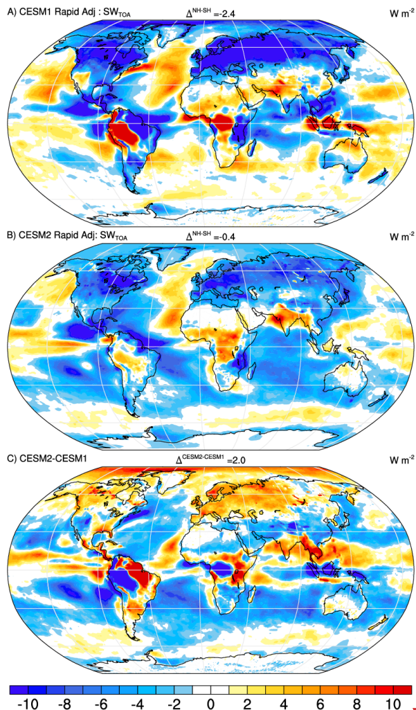
Figure 4: Estimates of the rapid adjustment of TOA net absorbed SW flux to CO 2 for CESM1 (a), CESM2 (b), and their difference (c) based on estimates from 4xCO 2 AMIP and AMIP simulations. Differences in the hemispheric means are shown in panel titles. All units are W m^{-2} .
