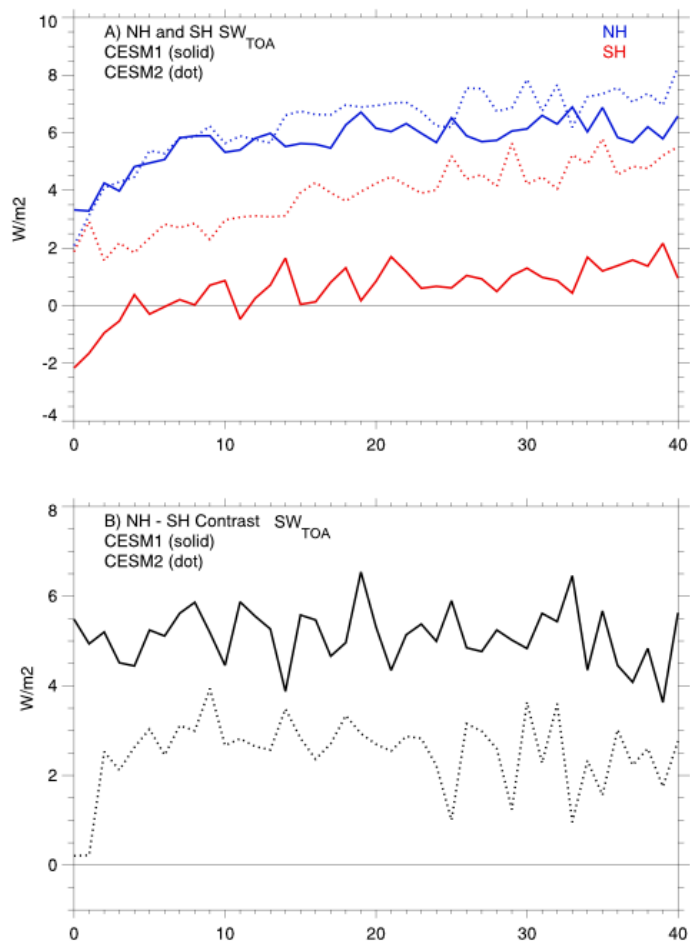
520 Figure A5. Timeseries of hemispheric mean absorbed TOA shortwave fluxes in CESM1 and CESM2 (a) and their differences (b) in abrupt4xCO 2 simulations.
