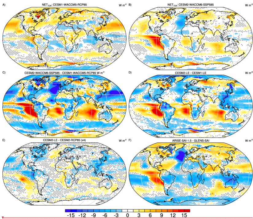
Figure A1. Normalized response in net incoming top-of-atmosphere radiative flux (RTMT) estimated from the change between 2020-39 and 2050-69 per degree global warming for unmitigated (a) CESM1-WACCM5-RCP85 and (b) CESM2-WACCM6-SSP585 simulations, and (c) their difference (b-a). Also shown is (d) the analogous difference for the CESM1-LE and CESM2-LE and (e) the CESM2-RCP85 and CESM2-LE (scaled by 4). The difference between the geoengineered climate states in ARISE-SAI-1.5 and GLENS-SAI is shown in (f). Units for all panels are W m^{-2} K^{-1} , except in (f) where units are W m^{-2} , and stippled regions indicate differences that are less than twice the ensemble standard error.
