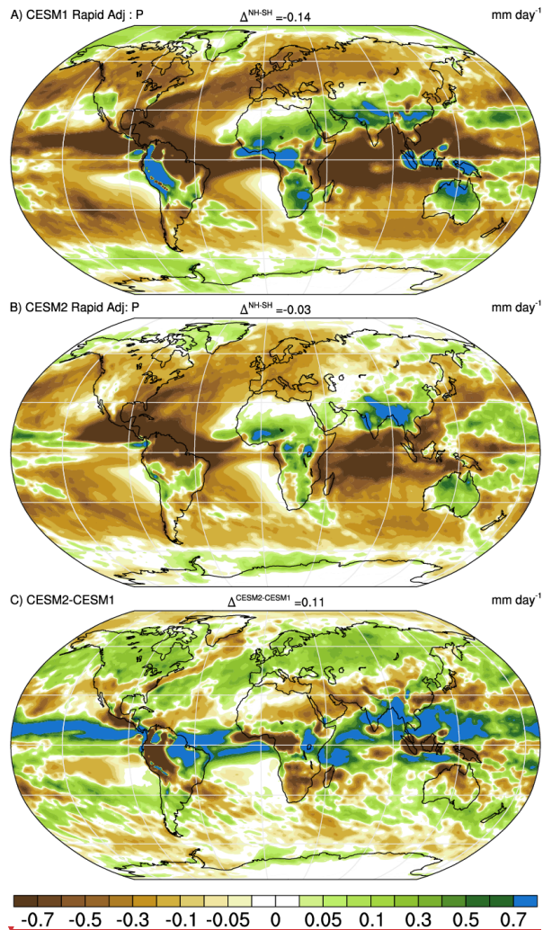
Figure A8. Rapid adjustments of precipitation (mm day -1 ) to CO 2 based on 4xAMIP-AMIP simulation differences in (a) CESM1, (b) CESM2, and (c) their difference (b-a).
