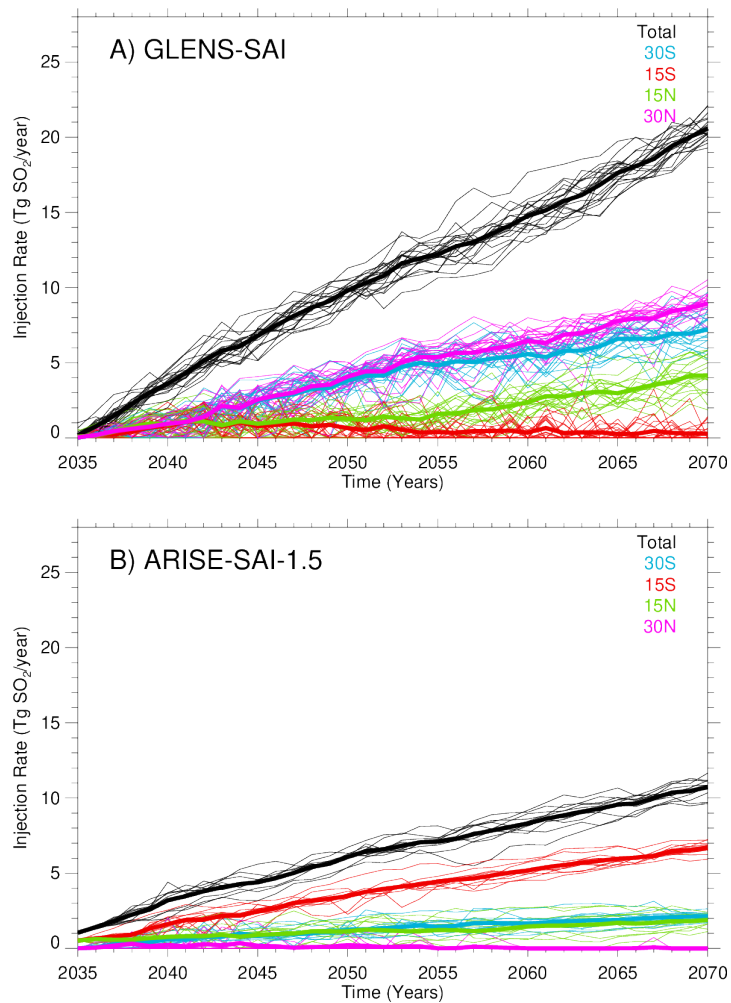
420 Figure 1: Evolution of yearly sulfur dioxide injections (Tg SO 2 yr -1 ) over time at the four injection latitudes for (a) GLENS-SAI and (b) ARISE-SAI-1.5 from 2035 to 2070.
