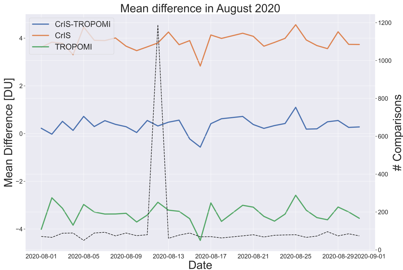
Figure 10. Global stratospheric column mean difference (in DU) between co-located MLS retrievals and CrIS-TROPOMI (blue), CrIS (orange) and TROPOMI (green) over the month of August in 2020. The number of co-located retrievals is shown in the black line.
