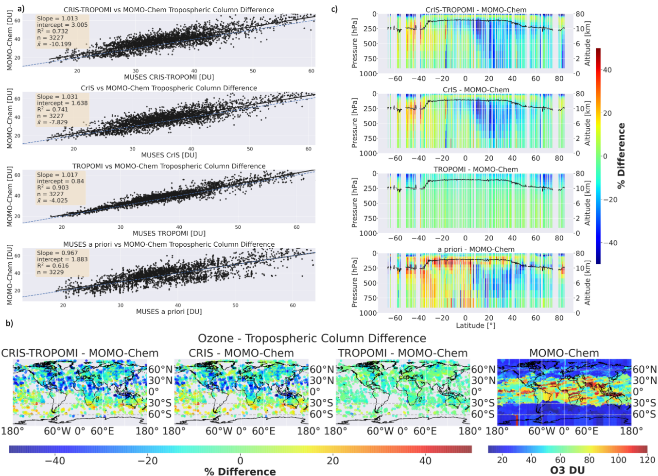
Figure 14. Cross-comparisons of JPL MOMO-Chem with CrIS-TROPOMI, CrIS and TROPOMI for the tropospheric column level on August 12 2020. The structure of the figure is the same as shown in Fig. 13.
