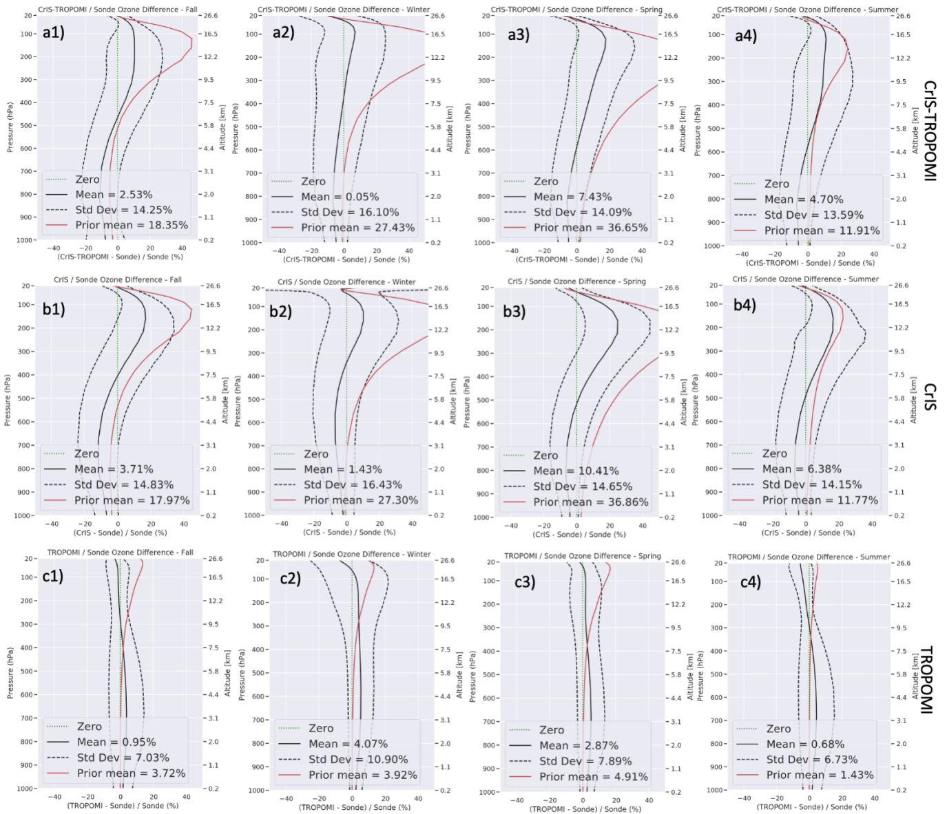
Figure 15. Ozonesonde comparisons MUSES CrIS-TROPOMI, CrIS and TROPOMI ozone retrievals. The columns represent the comparisons over different seasons (1=Fall, 2=Winter, 3=Spring, 4=Summer), the rows represent the instrument comparisons (a=CrIS-TROPOMI, b=CrIS, c=TROPOMI). The solid black lines are the mean difference, the dashed black lines are \pm 1\sigma , the red line is the a priori profile and the dashed green line is the zero line, these values for the tropospheric columns are indicated on the plots.
