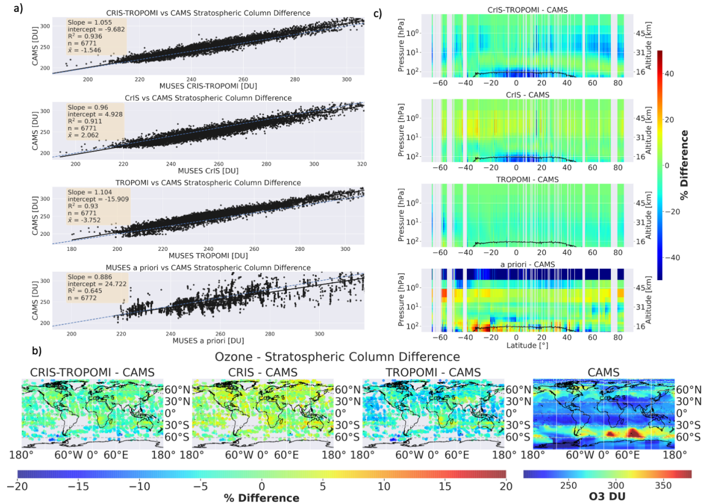
Figure B1. Cross-comparisons of CAMS-reanalysis with CrIS, TROPOMI and CrIS-TROPOMI on August 12 2020 for the stratospheric profile. The structure of this figure is as Fig. 9.
