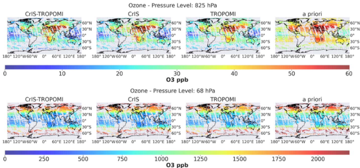
Figure 7. Global distributions of ozone on August 12 2020 in ppb, comprising of \sim 10k quality retrievals. The results shown in the left hand column are from the CrIS-TROPOMI retrievals, followed by CrIS, TROPOMI and the a priori in the right hand column. Each row indicates the ozone concentrations from an example pressure level; the first row is 825 hPa, the second row is 68 hPa. These pressure levels were chosen to represent a wide range of atmospheric conditions (lower troposphere, upper troposphere and stratosphere), as well as to coincide with peaks in the CrIS-TROPOMI AK.
