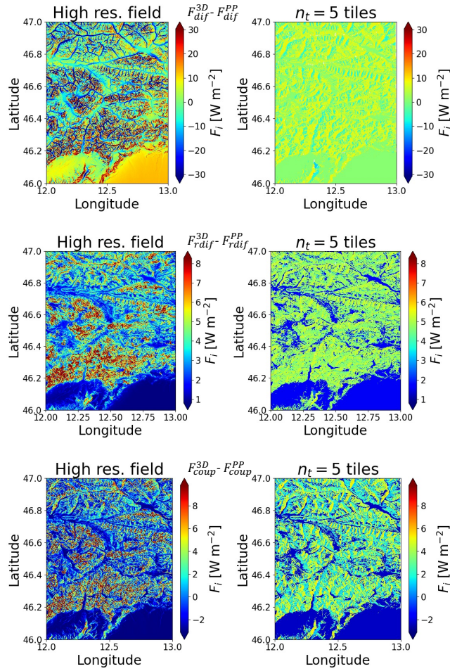
Figure 16. Downward radiation differences between 3D and PP fluxes for high resolution predictions (left column) and predictions for 5 tiles (right column) for each flux component. Results are shown for a representative case of cloudy sky conditions and \cos\theta_0 = 0.4 . Direct and reflected direct fluxes are zero in this case.
