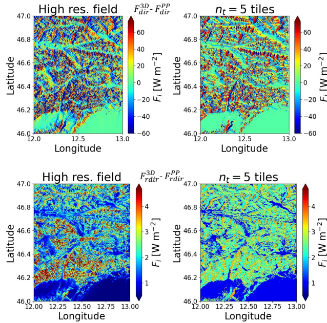
Figure 14. Downward radiation differences between 3D and PP fluxes for high resolution predictions (left column) and predictions for 5 tiles (right column) for each flux component. Results are shown for a representative case of clear sky conditions and \cos\theta_0 = 0.4 for direct flux (top panels) and reflected-directed flux (bottom).
