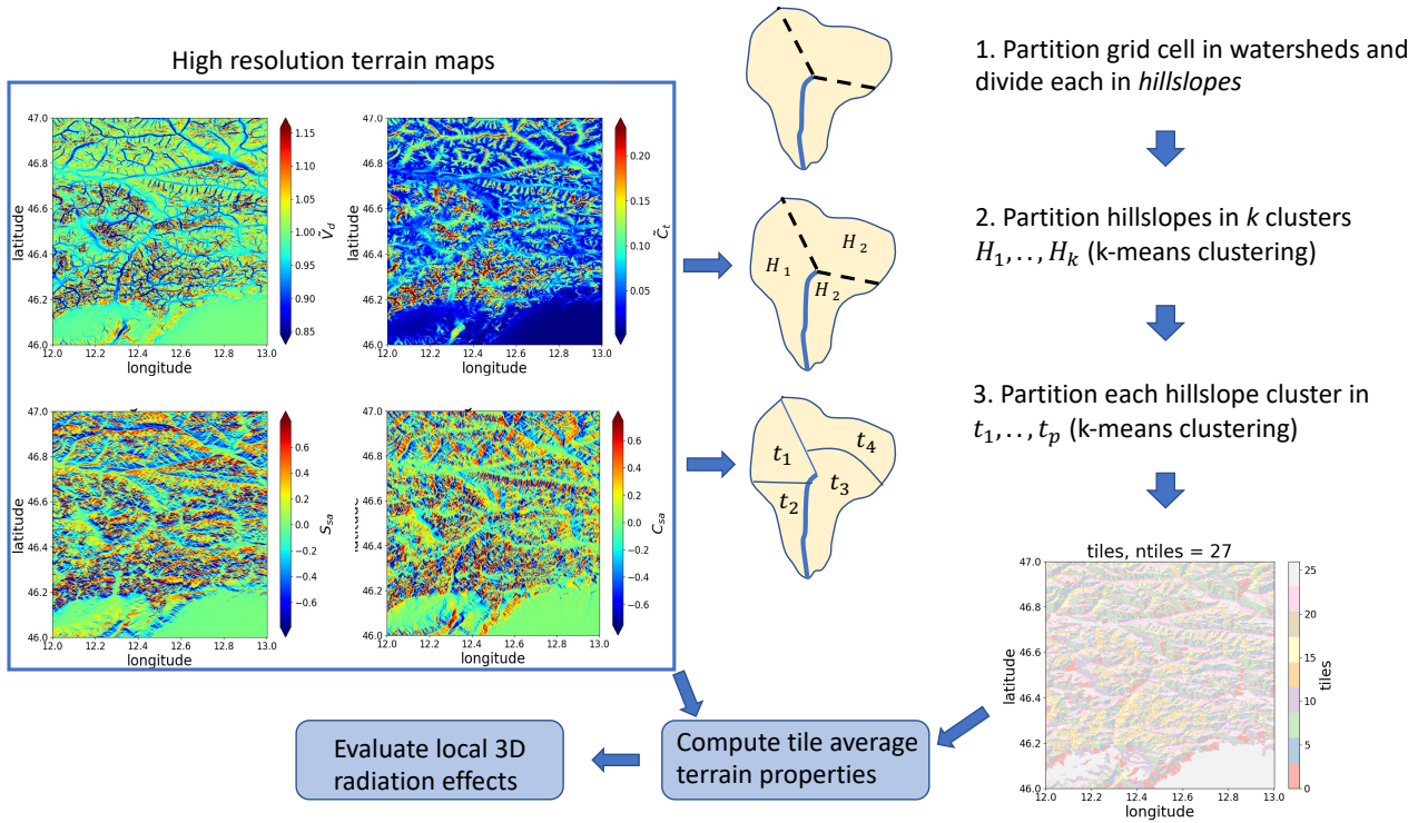
Figure 3. Schematic representation of the land clustering workflow. Land elevation maps are used to compute the variables of interest (sky and terrain view factors, and functions of terrain slope and aspect) which are then used in the hierarchical clustering step, which yields a map of homogeneous land units used to parameterize radiation-topography interactions. The delineation of channel network, watersheds and hillslopes follows the approach developed by (Chaney et al., 2018)
