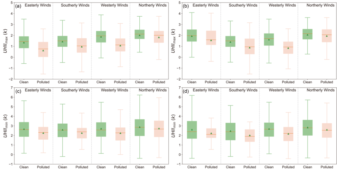
Figure 3: Distribution of UHII under different wind and pollution conditions. Panel (a) and (c) are classified based on the wind direction in urban areas, while panel (b) and (d) are based on wind direction in rural areas. Green triangles represent average values, red lines are median values; box chart values from the bottom to up are the mean value minus one time of standard deviation, 25% quantile line, 75% quantile line, and the mean value plus one time of the standard deviation.
