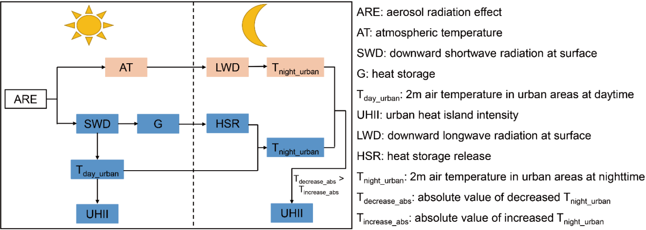
Figure 2: Flow chart shows how UHII is changed at daytime and nighttime, assuming that rural areas are not influenced by ARE. Pink boxes show increasing trend while blue ones show decreasing trend.
