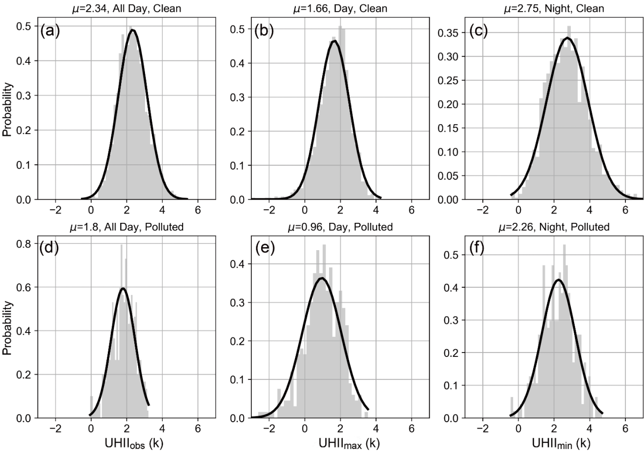
Figure 1: Probability distribution of UHII obs (a, d), UHII max (b, e) and UHII min (c, f) under different pollution conditions. The bold curve in each subgraph is normal distribution curve, and \mu denotes the average value.
