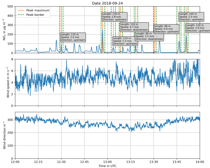
Figure 2. Example of the measured \text{NO}_x concentration, wind speed and wind direction at DURH (5 s time resolution). Ship peaks identified in the \text{NO}_x concentration are marked with an orange line, their borders are green dashed lines. The text box at each peak shows the ship length in m, the speed over ground in \text{m s}^{-1} and the direction of travel (upstream or downstream). Peaks without a label are most likely also caused by passing ships, but in these cases, unambiguous assignment of a source was not possible.
