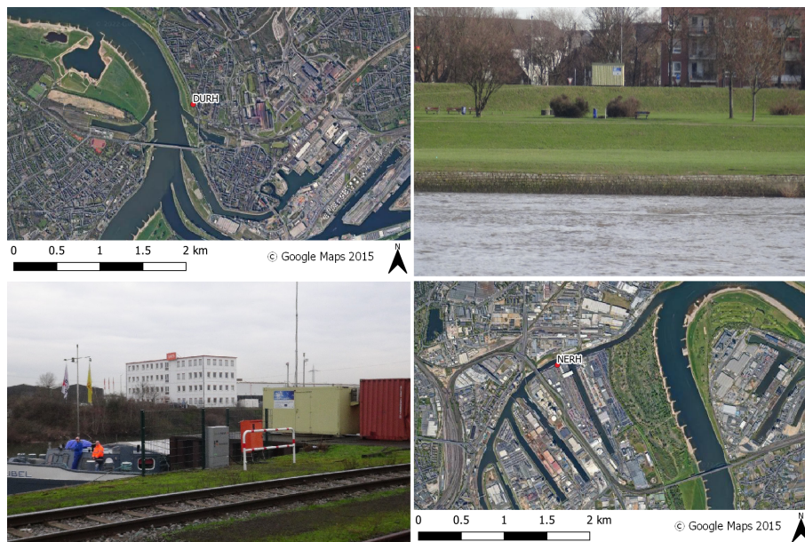
Figure 1. Views of the two different measurement sites used in this study. The upper row shows a satellite image of the DURH station and a picture of the measurement container as seen from the Rhine. The lower row shows a picture of the measurement container in the NERH and a satellite picture of its location.
