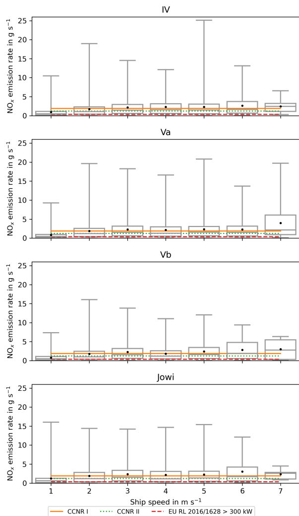
Figure 10. Boxplots of NO x emission rates for ship classes IV, Va, Vb and Jowi as a function of ship speed over ground, derived from data measured at DURH. Mean value is shown as a black dot, median value as grey line. The limits given by the CCNR I, CCNR II and EU RL2016/1628 regulations were converted from g kWh -1 to g s -1 and are shown as lines (see Table 6 for more details).
