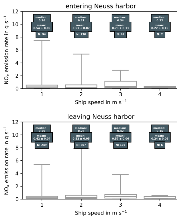
Figure 12. NO x emission rates for ship class IV and their dependence on the direction of travel and ship speed over ground, derived from data measured at NERH.
