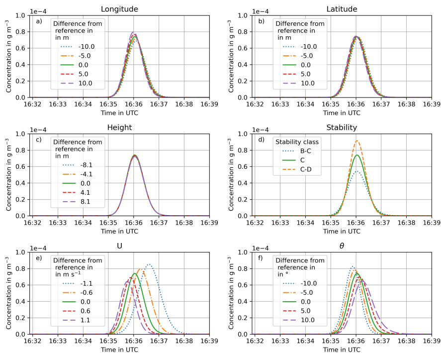
Figure C1. Monte-Carlo simulations for the example plume shown in Figure 4. In each plot one parameter has been changed within its respective uncertainty and the resulting model peaks are shown. The uncertainties shown in the plot legends are always expressed as deviation from the reference simulation, e.g. in plot a) -10 m means that the ship positions have systematically been moved 10 m to the west, while 10 m means each position has been moved 10 m to the east. The reference simulation (no uncertainty) is shown as a green solid line.
