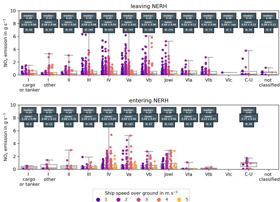
Figure 11. NO x emission rates for all ship classes, derived from measurements at NERH. Single measurements are colour-coded to the respective mean ship speed during the measurement.
