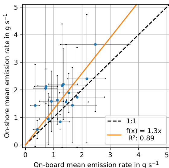
Figure 9. Scatter plot of on-board and on-shore emission rates. Each dot represents the mean value for one ship, errorbars indicate respective standard deviations. For ships with more than one main engine, the number of engines has been taking into account for the on-board emission rates. See also Table 4.
