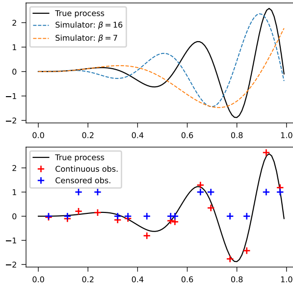
Figure 1. (upper) Synthetic true model and realizations of computational model runs; (lower) Continuous-Uncensored and binary observations of the true process
