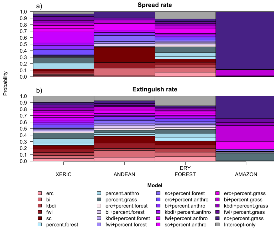
Figure 6. Barplots of Akaike weights - the probability that each model candidate is truly the best-approximating model - for each ecoregion and parameter. Models that contain both a FDI and land cover covariate are colored purple, those that contain only a FDI are colored red, those that only contain a land cover variable are colored blue, and the Intercept-only model are colored grey.
