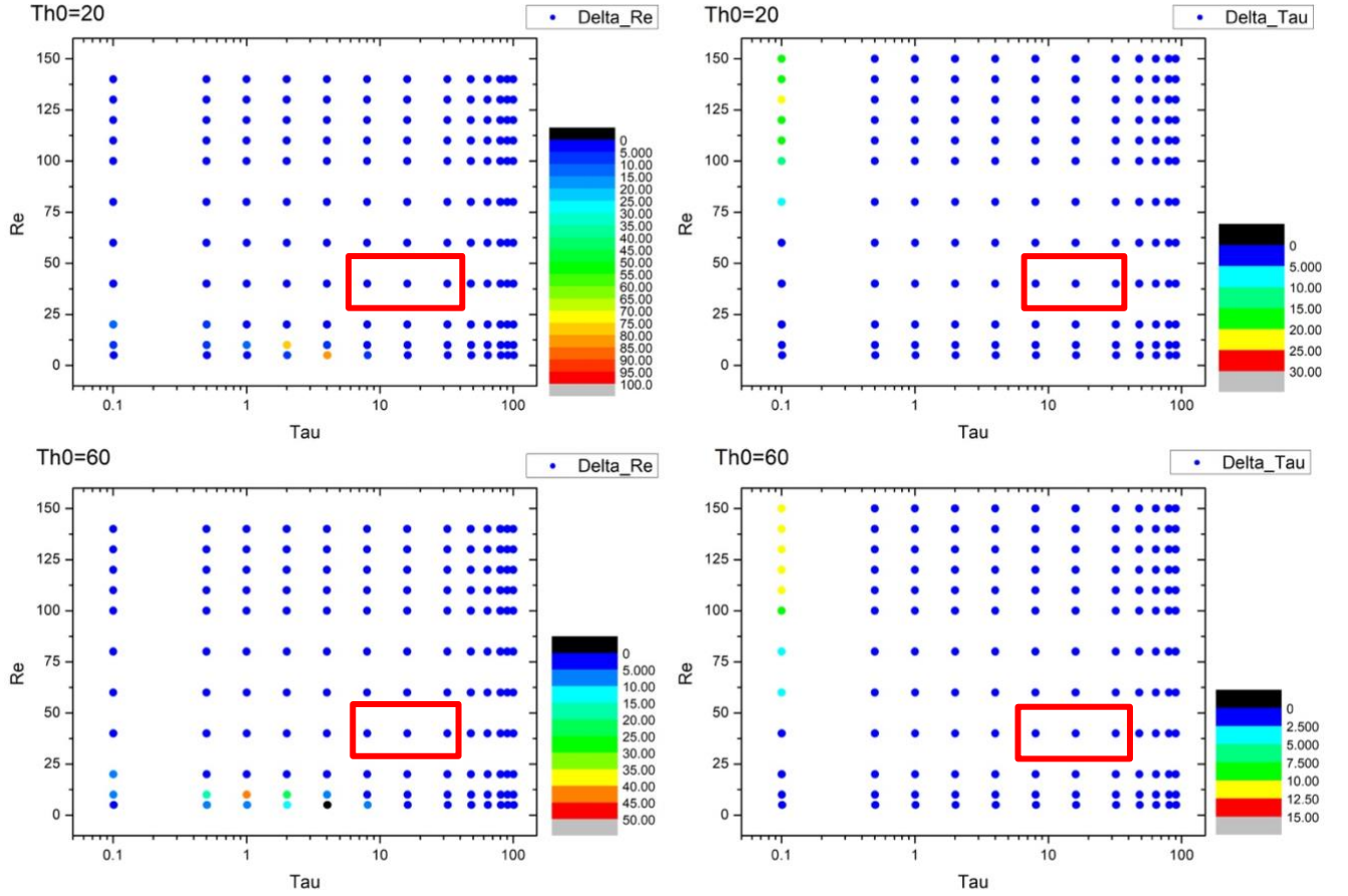
310 Figure 12: Error distributions of COT and CDR from the Nakajima-King diagram for deep convective clouds at \text{pix\_BND1\_max} . Upper left panel: distribution of \Delta \text{Re} for a solar zenith angle of 20^\circ . Upper right panel: distribution of \Delta \text{tau} for a solar zenith angle of 20^\circ . Lower left panel: distribution of \Delta \text{Re} for a solar zenith angle of 60^\circ . Lower right panel: distribution of \Delta \text{tau} for a solar zenith angle of 60^\circ . The red frames show the presence of typical deep convective clouds. COT = 8 or 32, CDR = 40 \mu\text{m} .
