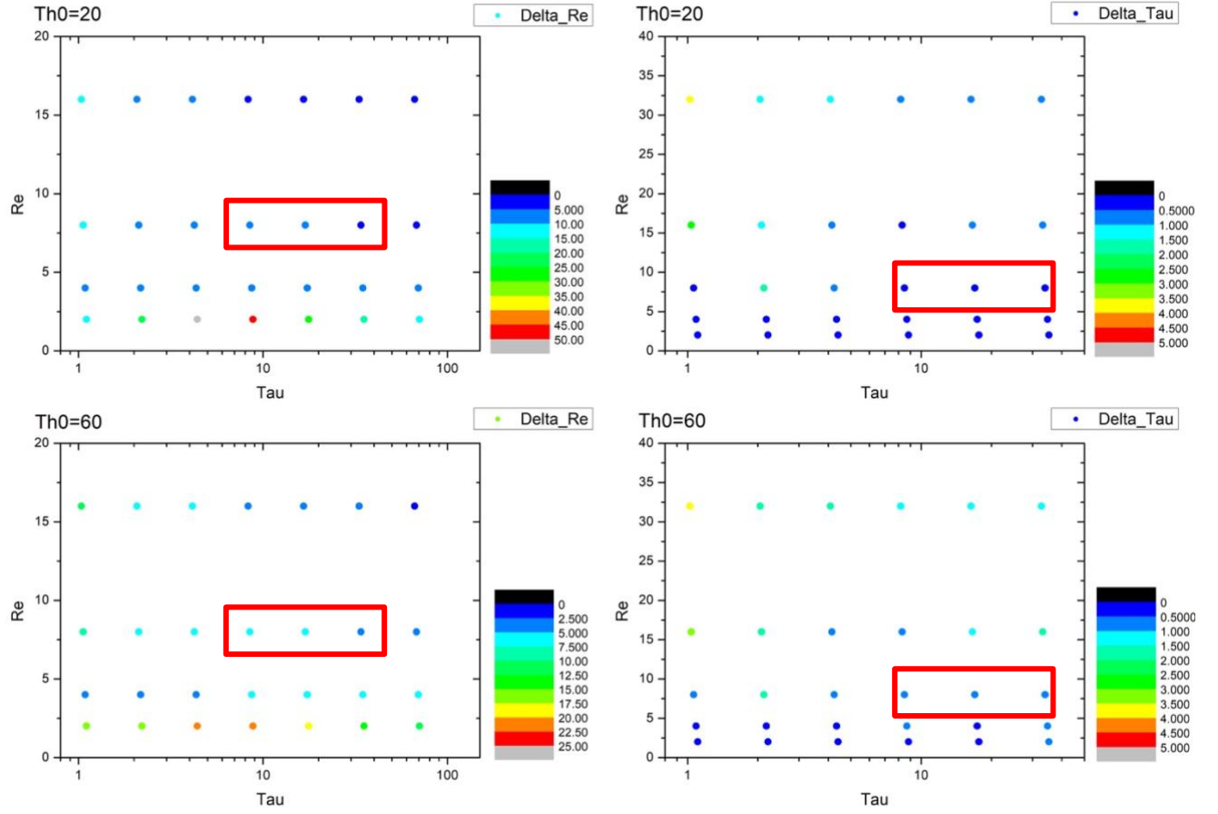
Figure 10: Error distributions of COT and CDR from the Nakajima-King diagram for shallow warm clouds at \text{pix\_BND3\_max} . Upper left panel: distribution of \Delta r_e for a solar zenith angle of 20^\circ . Upper right panel: distribution of \Delta \tau for a solar zenith angle of 20^\circ . Lower left panel: distribution of \Delta r_e for a solar zenith angle of 60^\circ . Lower right panel: distribution of \Delta \tau for a solar zenith angle of 60^\circ . The red frames show the presence of typical shallow warm clouds. COT = 8 or 32, CDR = 8 \mu\text{m} .
