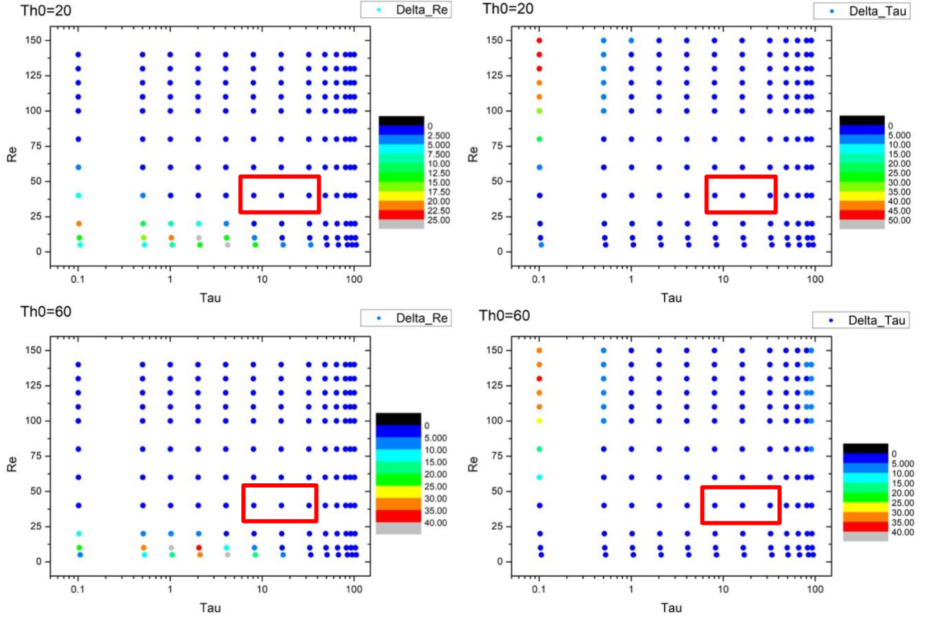
Figure 14: Error distributions of COT and CDR from the Nakajima-King diagram for deep convective clouds at pix_BND3_max. Upper left panel: distribution of \Delta r_e for a solar zenith angle of 20^\circ . Upper right panel: distribution of \Delta \tau for a solar zenith angle of 20^\circ . Lower left panel: distribution of \Delta r_e for a solar zenith angle of 60^\circ . Lower right panel: distribution of \Delta \tau for a solar zenith angle of 60^\circ . The red frames show the presence of typical deep convective clouds. COT = 8 or 32, CDR = 40 \mu\text{m} .
