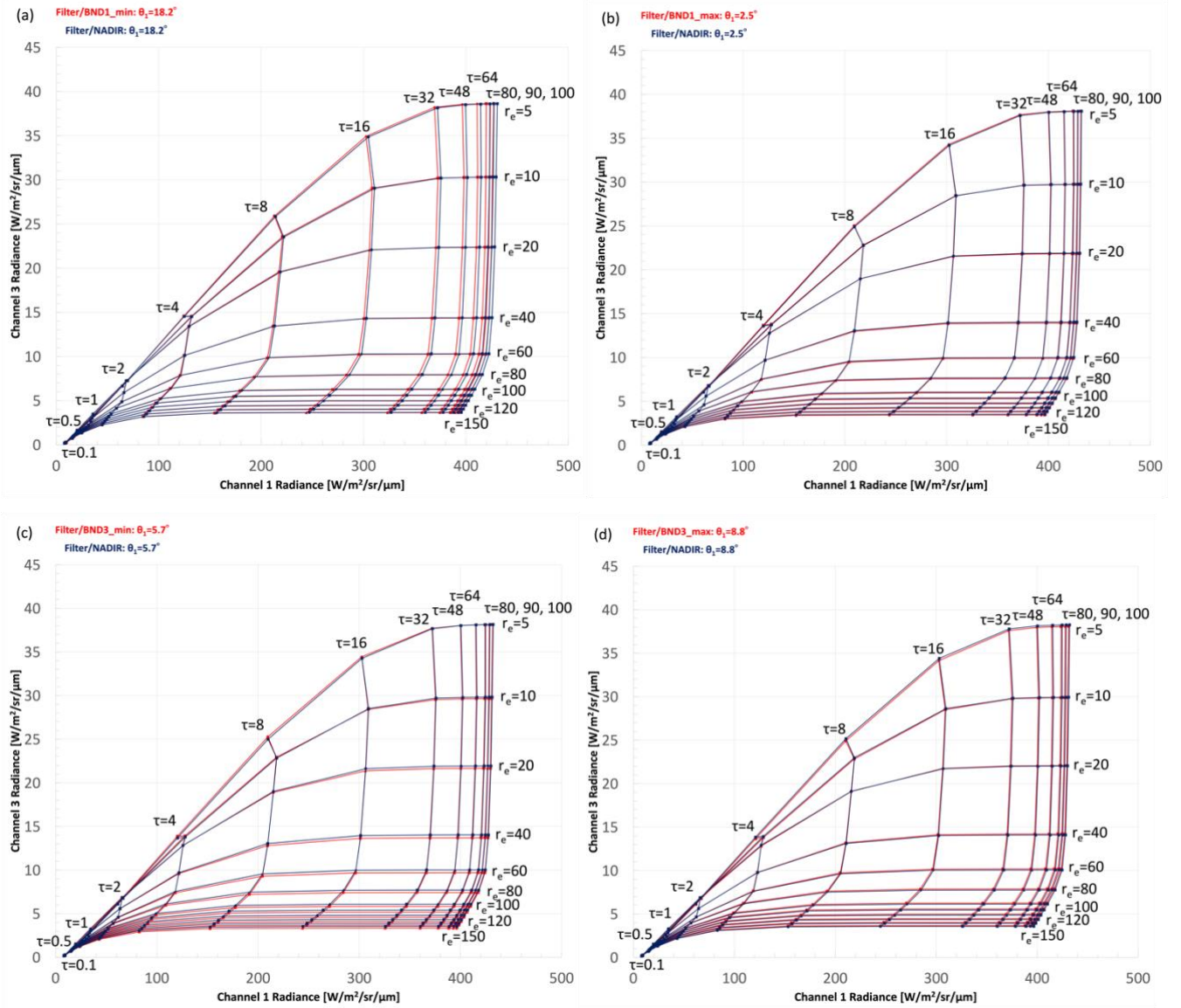
Figure 6: Nakajima-King diagrams for deep convective clouds at (a) pix_BND1_min, (b) pix_BND1_max, (c) pix_BND3_min, and (d) pix_BND3_max for a solar zenith angle of 20^\circ . The red lines show the results from the response function with SMILE. The black lines show the results from the nadir response function.
