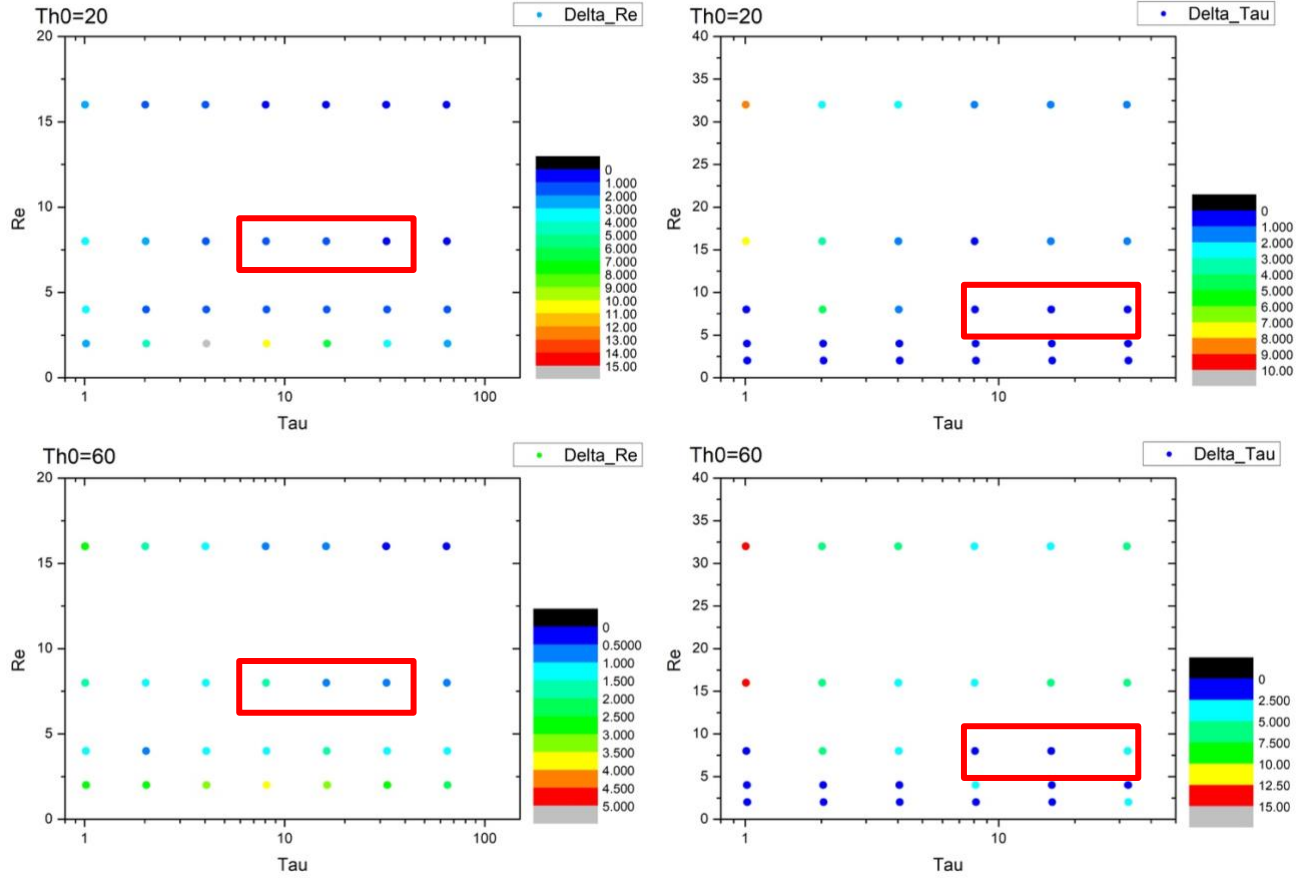
280 Figure 7: Error distributions of COT and CDR from the Nakajima-King diagram for shallow warm clouds at pix_BND1_min. Upper left panel: distribution of \Delta Re for a solar zenith angle of 20^\circ . Upper right panel: distribution of \Delta \tau for a solar zenith angle of 20^\circ . Lower left panel: distribution of \Delta Re for a solar zenith angle of 60^\circ . Lower right panel: distribution of \Delta \tau for a solar zenith angle of 60^\circ . The red frames indicate the presence of typical shallow warm cloud. COT = 8 or 32, CDR = 8 \mu m .
