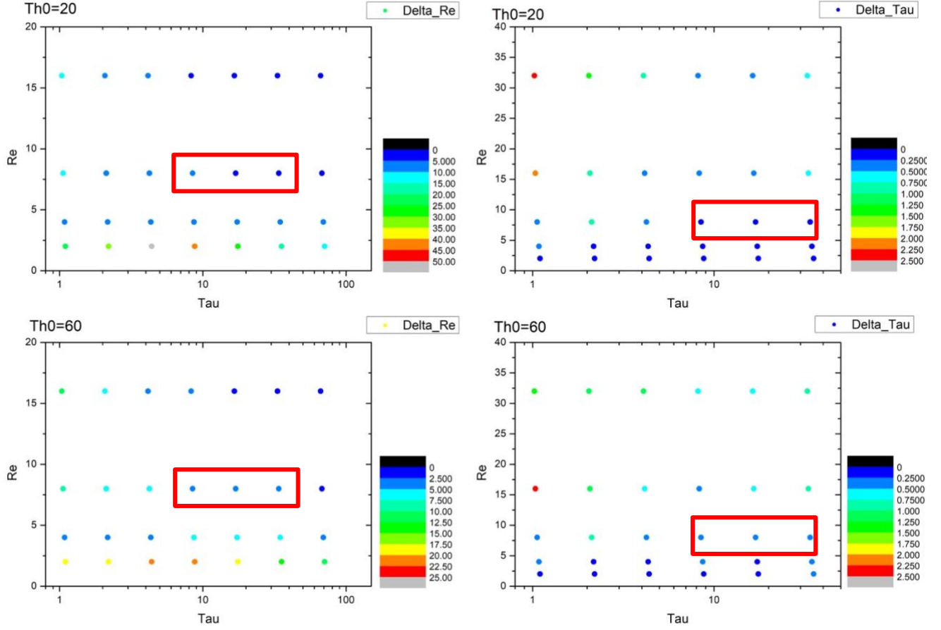
Figure 9: Error distributions of COT and CDR from the Nakajima-King diagram for shallow warm clouds at pix_BND3_min. Upper left panel: distribution of \Delta Re for a solar zenith angle of 20^\circ . Upper right panel: distribution of \Delta \tau for a solar zenith angle of 20^\circ . Lower left panel: distribution of \Delta Re for a solar zenith angle of 60^\circ . Lower right panel: distribution of \Delta \tau for a solar zenith angle of 60^\circ . The red frames show the presence of typical shallow warm cloud. COT = 8 or 32, CDR = 8 \mu m .
