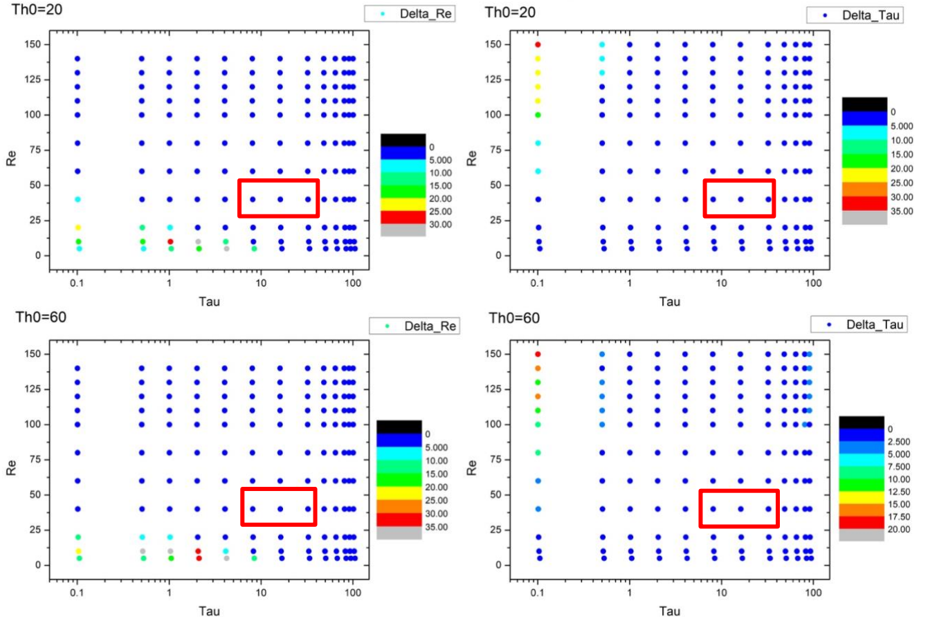
Figure 13: Error distribution of COT and CDR from Nakajima-King diagram for deep convective clouds, at pix_BND3_min. Upper left panel: distribution of \Delta Re for a solar zenith angle of 20^\circ . Upper right panel: distribution of \Delta \tau for a solar zenith angle of 20^\circ . Lower left panel: distribution of \Delta Re for a solar zenith angle of 60^\circ . Lower right panel: distribution of \Delta \tau for a solar zenith angle of 60^\circ . The red frames show the presence of typical deep convective clouds.
