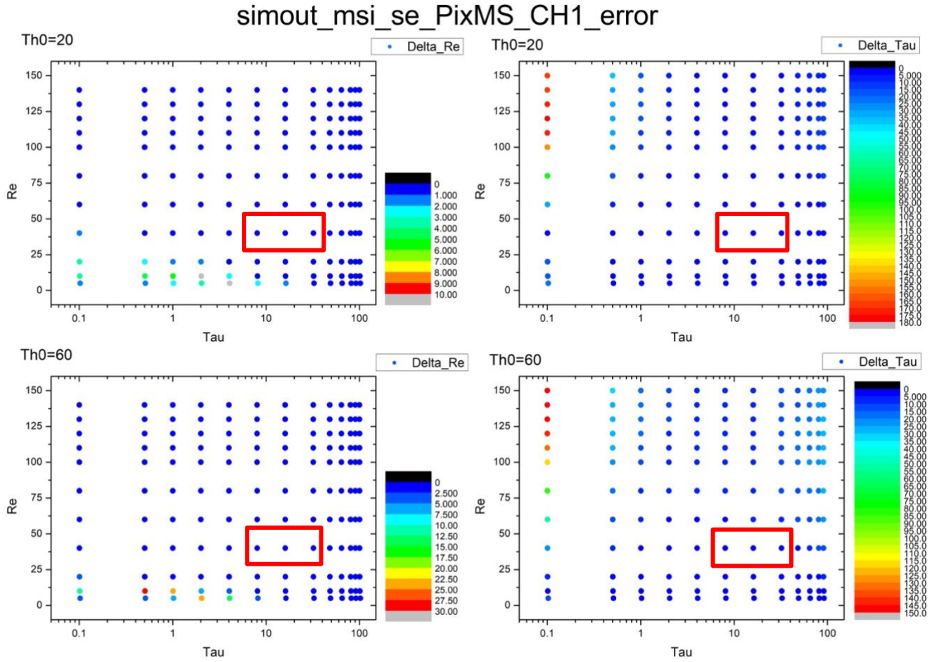
Figure 11: Error distributions of COT and CDR from the Nakajima-King diagram for deep convective clouds at \text{pix\_BND1\_min} . Upper left panel: distribution of \Delta \tau_e for a solar zenith angle of 20^\circ . Upper right panel: distribution of \Delta \tau for a solar zenith angle of 20^\circ . Lower left panel: distribution of \Delta \tau_e for a solar zenith angle of 60^\circ . Lower right panel: distribution of \Delta \tau for a solar zenith angle of 60^\circ . The red frames show the presence of typical deep convective clouds. COT = 8 or 32, CDR = 40 \mu\text{m} .
