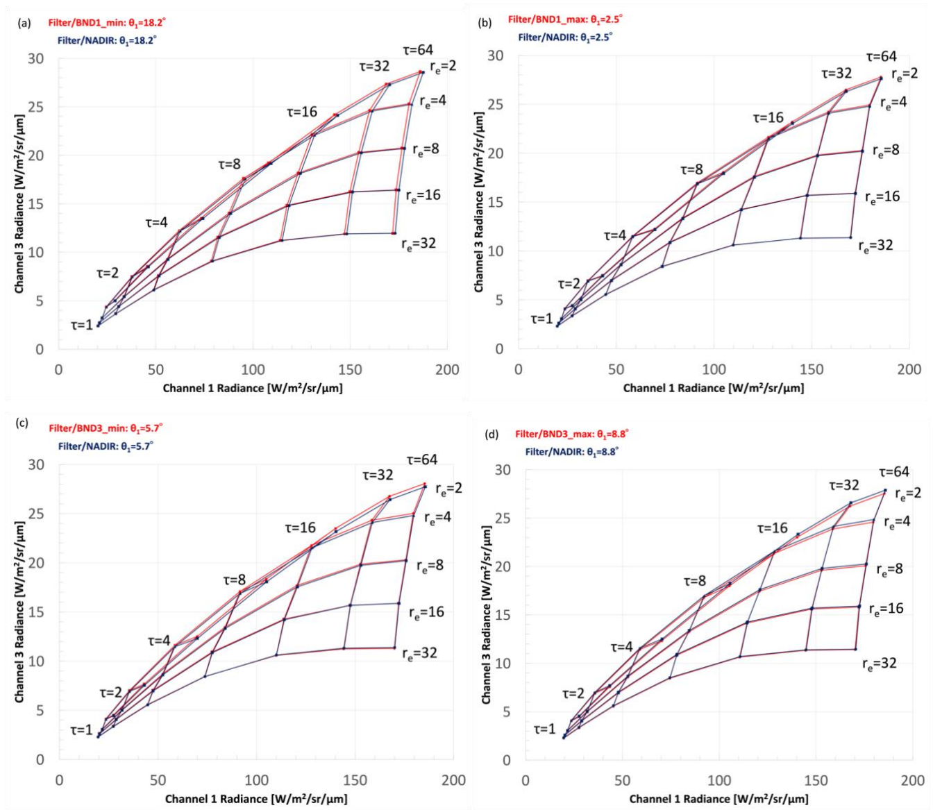
Figure 3: Nakajima-King diagrams for shallow warm clouds at (a) pix_BND1_min, (b) pix_BND1_max, (c) pix_BND3_min, and (d) pix_BND3_max for a solar zenith angle of 60^\circ . The red lines show the results from the response function with SMILE. The black lines show the results from the nadir response function.
