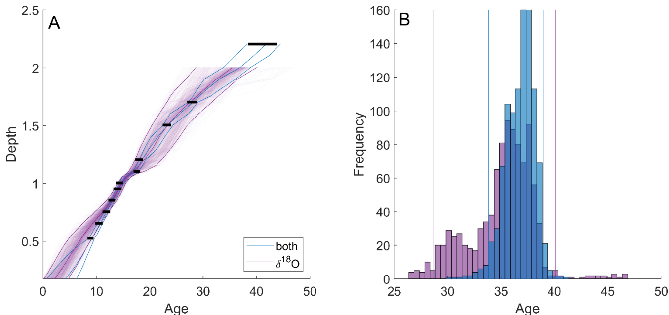
545 Figure 7: (A) Sample density of the \delta^{18}\text{O} -only age model for GIK13289-2. The median age model and 95% confidence bands are plotted as solid purple lines. The multiproxy median age model and 95% confidence bands are also plotted (solid blue lines) along with the calibrated radiocarbon ages (horizontal black lines). (B) Histogram of \delta^{18}\text{O} -only age samples (purple) and multiproxy age model samples (blue) for the last depth in the \delta^{18}\text{O} -only age model (approximately 2 m). Vertical lines mark the Confidence 95% credible intervals at the same depth widths for both age models are indicated with vertical lines.
