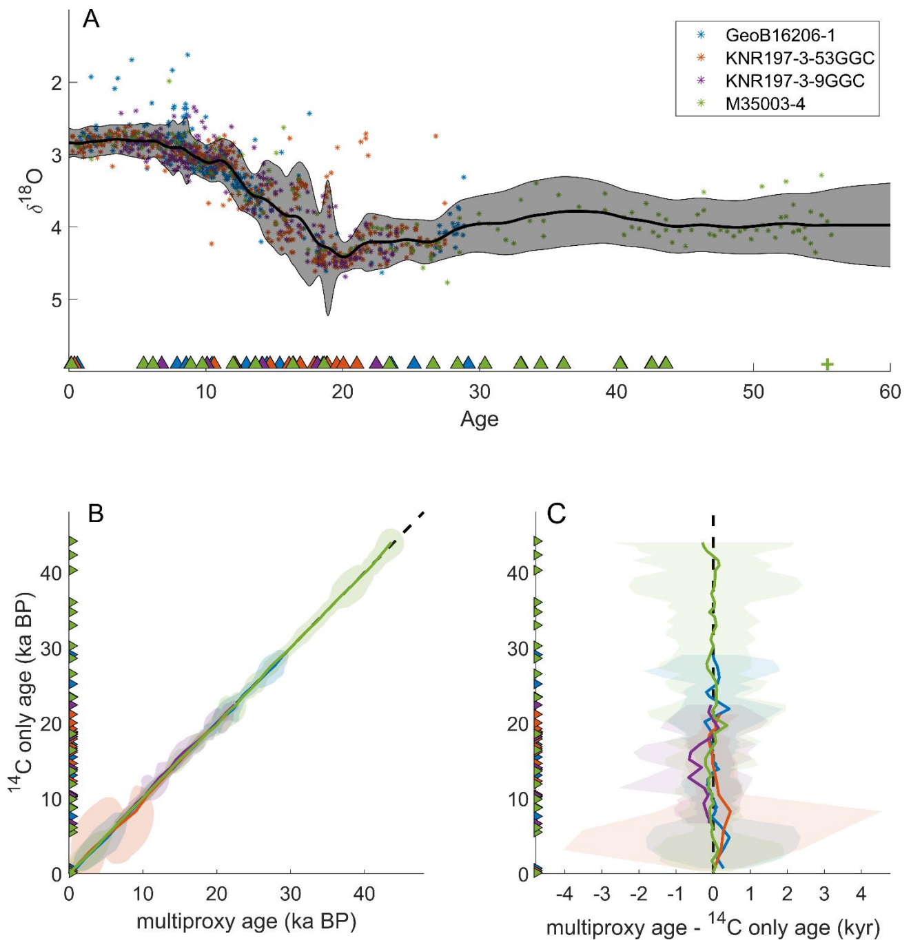
500 Figure 4: The Intermediate Tropical West Atlantic (ITWA) stack. (A) The solid black line and shaded region represents the median 505 stack value and 2-sigma upper and lower bounds. Filled circles are the shifted and scaled \delta^{18}\text{O} data points from each core on the multiproxy age models. Filled triangles mark radiocarbon ages from the respective cores. The green cross is the tie point for M35003- 4 from Hulz et al., (2000). (B) ^{14}\text{C} -only age models vs. the multiproxy age models for each core in the ITWA stack. Each core plots along the black dashed 1:1 line. (C) The difference between the multiproxy age models and the ^{14}\text{C} age models for each core. Coloured shading shows the joint uncertainty distribution for ^{14}\text{C} and multiproxy age estimates for each core.
