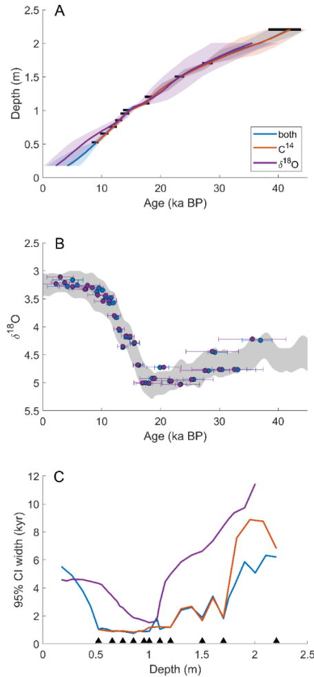
Figure 6: Comparison of a \delta^{18}\text{O} -only age model, radiocarbon-only age model, and multiproxy age model for GIK13289-2. (A) Age vs. depth plot, solid black lines represent calibrated radiocarbon ages. (B) The shifted and scaled \delta^{18}\text{O} for the \delta^{18}\text{O} -only age model and multiproxy age model aligned to the DNEA stack. (C) 95% confidence-credible interval widths for each age model. Black triangles indicate the depths of the radiocarbon ages. Note that the radiocarbon-only age model does not extend beyond the top ^{14}\text{C} date of ~10 ka BP, and we do not display the ^{14}\text{C} age model in panel (B).
