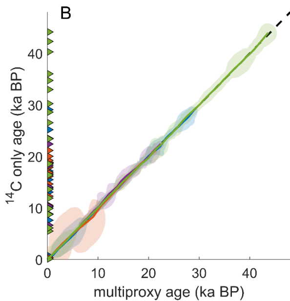
490 Figure 3: The Deep Northeast Atlantic (DNEA) stack. (A) The solid black line and shaded region represents the median stack value and 2-sigma upper and lower bounds. Filled circles are the shifted and scaled \delta^{18}\text{O} data points from each core on the multiproxy age models. Filled triangles mark the radiocarbon ages from the respective cores. Purple crosses are the tie points for MD95-2042 taken from Lisiecki & Stern (2016). (B) ^{14}\text{C} -only age models vs. the multiproxy age models for each core in the DNEA stack. Each core plots along the black dashed 1:1 line. (C) The difference between the multiproxy age models and the ^{14}\text{C} age models for each core in 495 the DNEA stack. Coloured shading shows the joint uncertainty distribution for ^{14}\text{C} and multiproxy age estimates for each core.
