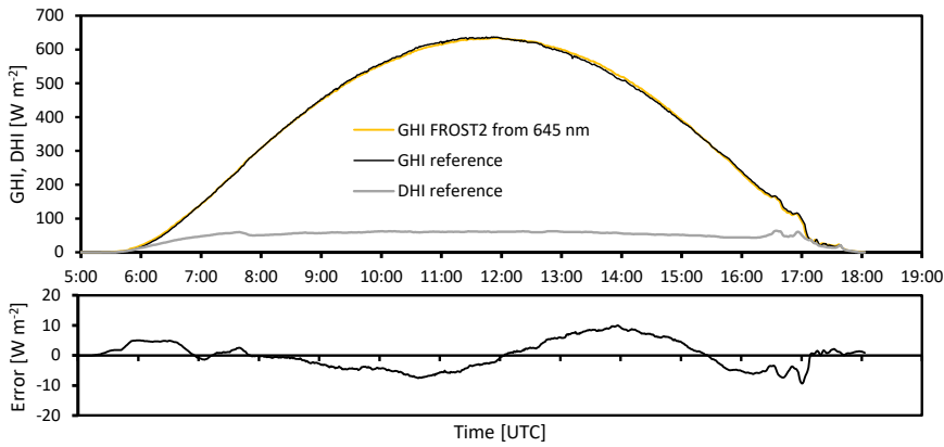
461 Figure 13: Comparison between GHI measured using a pyrliometer and diffuse radiation sum (on a 462 suntracker and correcting for zenith angle) and a calibrated FROST2 with 2 mm PTFE diffuser and 1 463 correction filter, diffuse horizontal irradiance (DHI) measured with pyranometer mounted on a suntracker 464 with shading ball, Veenkampen weather station, 19 March 2022. Relative errors at GHI >200 W m -2 are 465 <2% and mainly related to horizontal misalignment causing an asymmetric error before/after noon.
