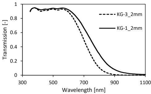
339 340 Figure 7: Correction filters for the infrared crosstalk: Schott heat-absorbing filters (adapted from Schott 341 AG manufacturer data).
