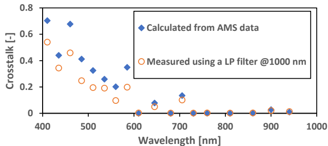
283 284 Figure 5: Measured spectroscopy sensor infrared crosstalk from wavelengths >1000 nm, tested with a 285 Xenon lamp and an optical long pass filter (LP at 1000 nm) and calculated from spectral response data as 286 supplied by the manufacturer (AMS). Crosstalk is defined as the fraction of light wavelengths >1000 nm 287 the sensor is responding to, for example at 410 nm 55% of the measured signal is actually originating 288 from wavelengths >1000 nm.
