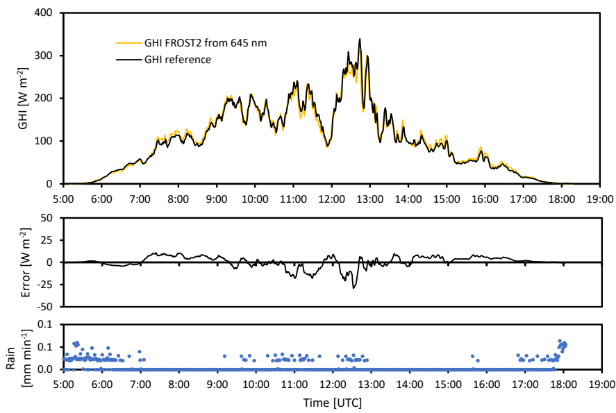
479 Figure 15: Calibrated FROST2 GHI from 645 nm (calibrated on a clear day, 19 March, see Fig. 13), 480 calibration tested under rainy weather conditions, 1 minute averaged data, error plot 10 min running 481 mean to suppress differences due to spatial separation of FROST and reference (145 m apart), 482 Veenkampen weather station, 31 March 2022. Relative errors at GHI >100 W m -2 are <7% and mainly 483 related to spatial separation between FROST and reference.
