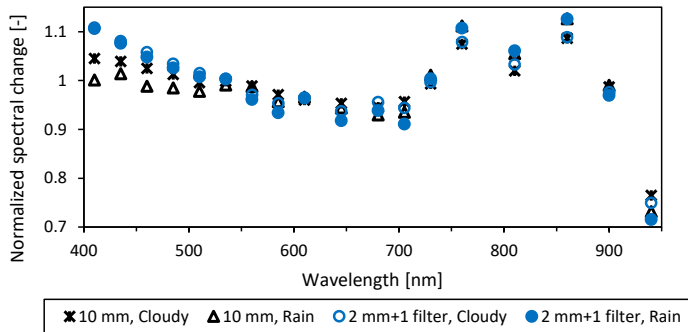
506 507 Figure 16: Two FROST instruments, one with a 10 mm diffuser (FROST1) and one with a 2 mm diffuser 508 and correction filter (FROST2). The normalized spectral cloud modification factor, is the spectral change 509 of cloudy (14 March, 2022) and rainy weather (31 March, 2022) compared to a cloud-free day (19 March 510 2022), Veenkampen weather station, data averaged between 11 and 12 UTC for each day.
