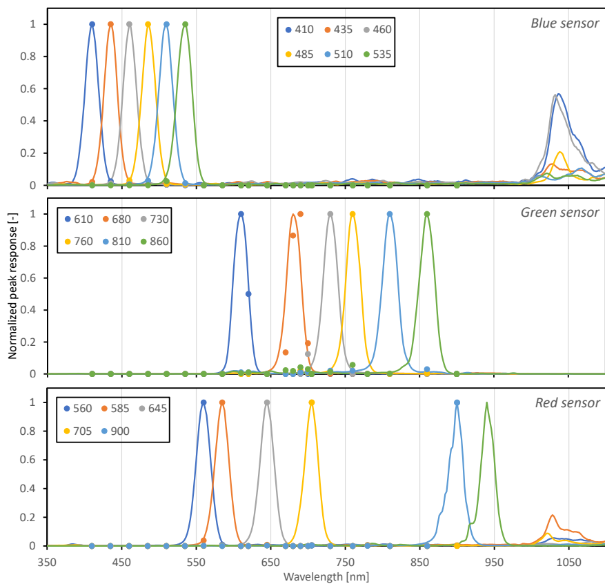
308 Figure 6a: Normalized peak spectral response of the triple AMS sensor (denoted as blue, green and red 309 sensor), data provided by manufacturer after consultation (solid lines) and our measured response up to 310 900 nm (dots) as measured with a sensor placed inside a Cary 4000 UV-Vis spectrophotometer equipped 311 with a universal measurement accessory.
