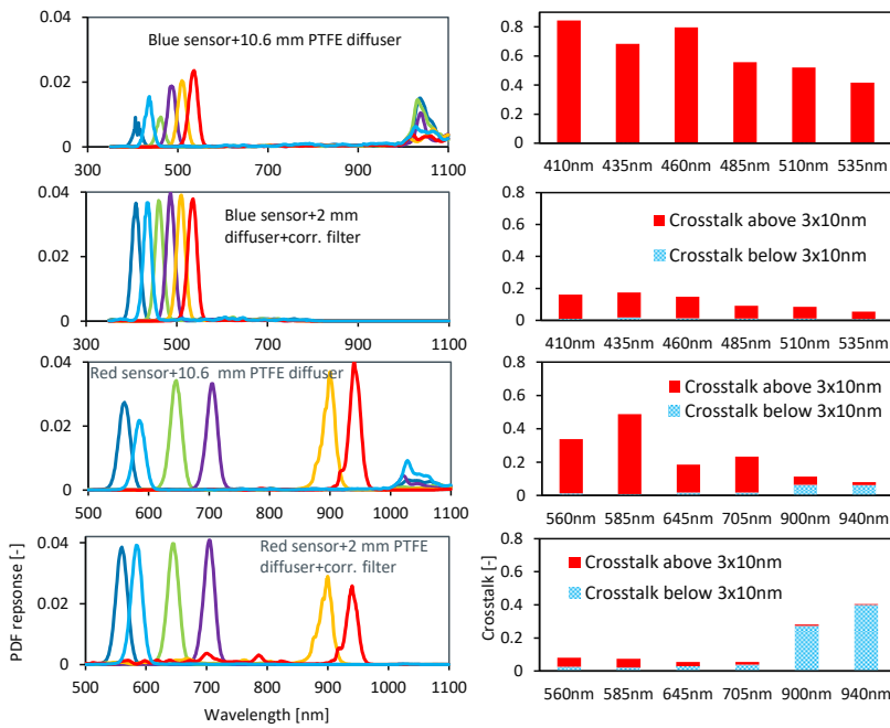
343 344 Figure 8: Spectral response and crosstalk (for a flat spectrum) of the blue and red sensor, without or 345 with correction filter. First row: Blue sensor with 10.6 mm PTFE diffuser. Second row: Blue sensor with 2 346 mm PTFE diffuser including a heat absorbing filter (Schott KG-3). Third row: Red sensor with 10.6 mm 347 PTFE diffuser. Fourth row: Red sensor with 2 mm PTFE diffuser and heat absorbing filter (Schott KG-1), 348 calculated from manufacturer data of sensor spectral response, transmission data of the Schott optical 349 correction filter, and measured transmission of PTFE diffusers.
