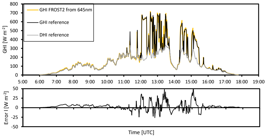
469 Figure 14: Calibrated FROST2 GHI from 645 nm (calibrated on a clear day, 19 March, see Fig. 13), 470 calibration tested with cloudy weather conditions. Cloudy weather conditions in the morning, some 471 clearing in the afternoon, 1 minute averaged data, error plot 10 min running mean to suppress 472 differences due to spatial separation of FROST and reference (145 m apart), Veenkampen weather 473 station, 14 March 2022. Relative errors at GHI >100 W m -2 are <7% and mainly related to spatial 474 separation between FROST and reference.
