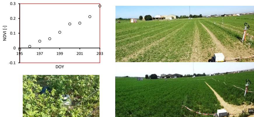
602 Figure 21: NDVI measurements calculated from FROST1 (with 10 mm diffuser) 680 and 730 nm 603 wavebands located inside an alfalfa canopy. Bottom left: FROST (top at about 8 cm height) placed on the 604 surface in between alfalfa, crop height 30 cm, (18 July). Top right: alfalfa crop on 14 July (crop height 23 605 cm). Bottom right: alfalfa crop (height 48 cm) on 22 July; Spain from 14-22 July 2022.
