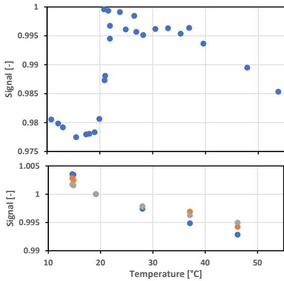
426 Figure 11: Temperature response; upper panel PTFE diffuser, lower panel 3 random light sensors (-250 427 ppm).
