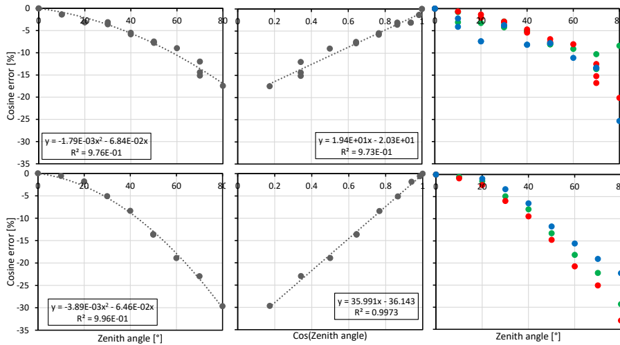
440 Figure 12: Upper graphs: 10.6 mm diffuser (black sides). Bottom graphs: 2 mm diffuser (sides painted 441 black). The right panels are color-coded for each sensor integrated circuit.
