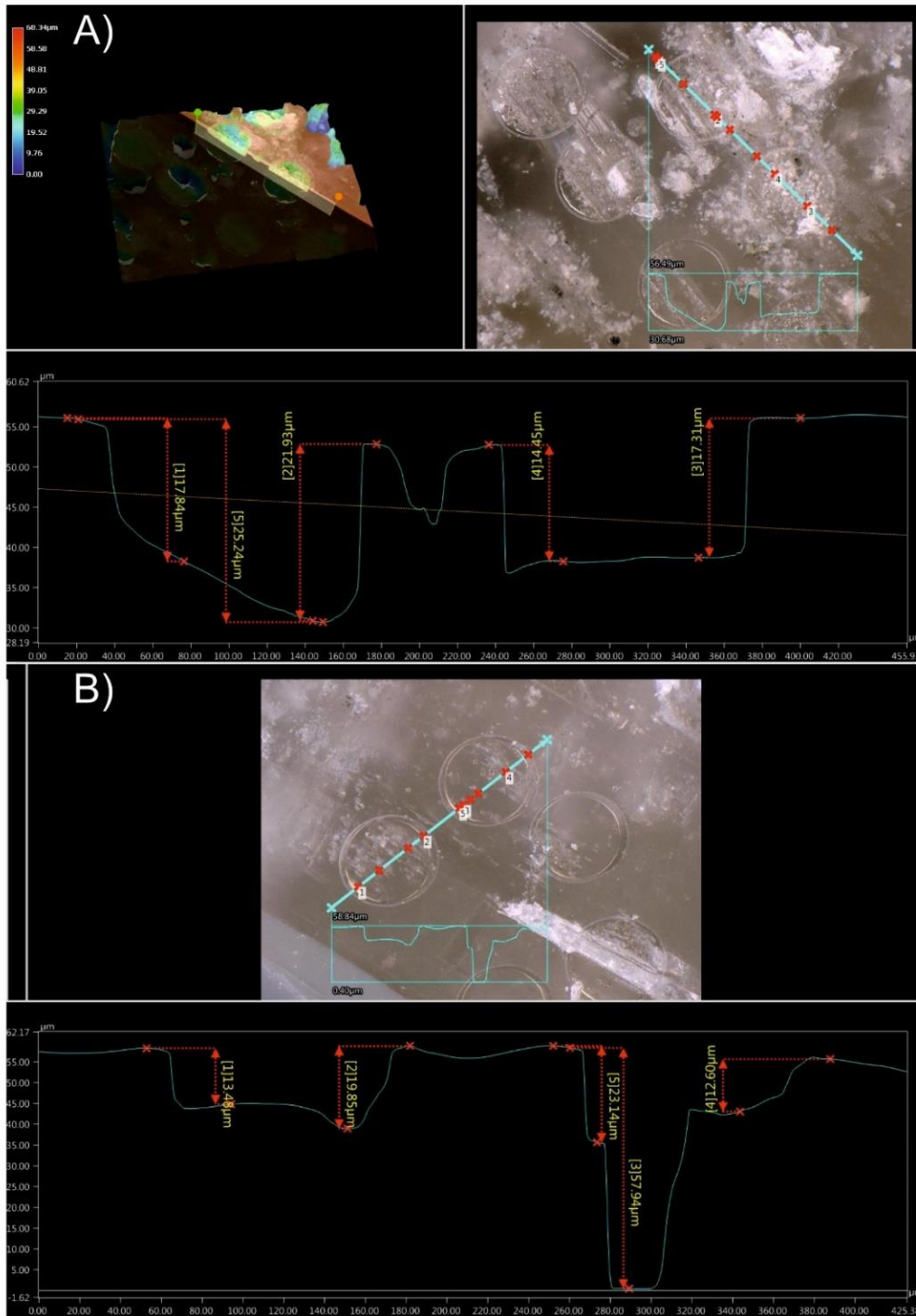
Fig. 4: Pit depth profile of the samples MTO 11-3 (a) and BCR 9644 (b). Whereas the pit shape is roughly homogeneous in the MTO 11-3, the sample BCR 9644 displays deeper areas in some of the pits. The profiles are measured using a Keyence digital microscope VHX-6000.
