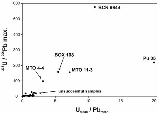
Fig. 2: Diagram showing \text{U}_{\text{mean}} \text{ content} / \text{Pb}_{\text{mean}} \text{ content} vs. maximum value on ^{238}\text{U} / ^{206}\text{Pb} axis. The successfully dated samples have a distinctively higher U/Pb heterogeneity.
