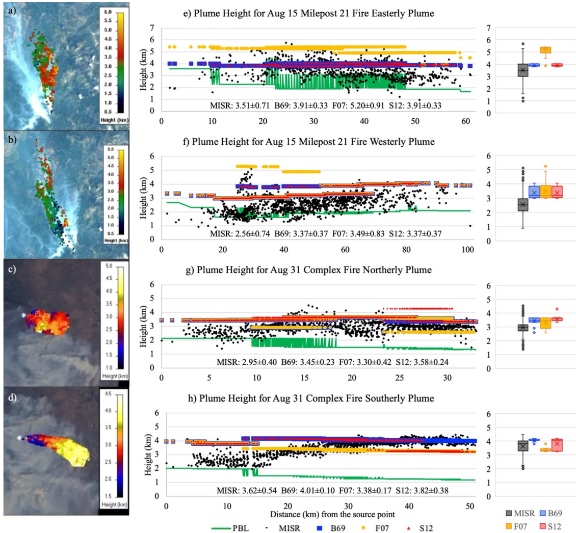
270 Figure 3: MISR plume heights superposed on the MODIS Terra visible images** (a-d) and the comparisons of the observed plume height with the simulated plume heights (e-h) for the August 15 th Milepost 21 fire easterly plume (a, e), westerly plume (b, f), August 31 st Complex fire northerly plume (c, g), and southerly plume (d, h).
