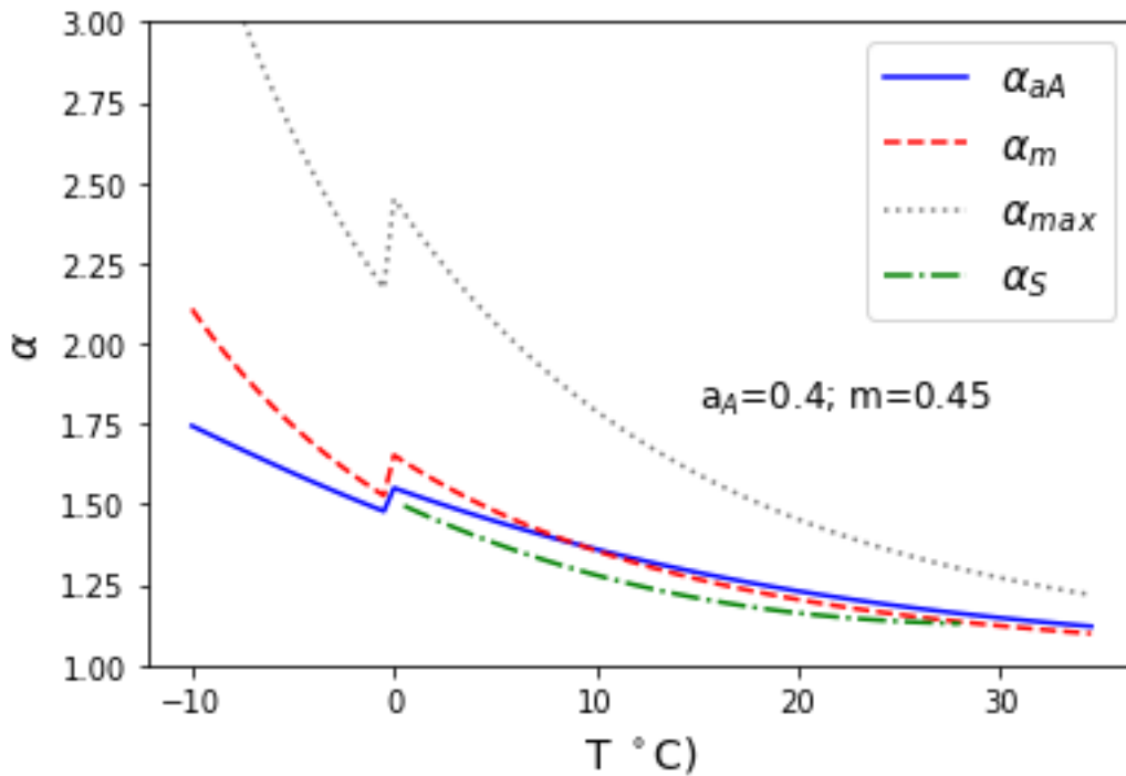
505 Figure 5. Variability of \alpha from (8) and (9) with wet surface temperature. The value a_A=0.4 was chosen because it was recommended by Andreas (2013); the value of m=0.45 was chosen to approximately mimic the trends with the Andreas method. Here \alpha_{max}=1+\gamma/\Delta_{T0} , the maximum value of \alpha suggested by Priestley and Taylor (1972). The green dash-dot line is \alpha_S , based on the third-order polynomial suggested by Szilagyi et al., 2014, on the basis of their analysis of ERA-Interim data over saturated surfaces.
