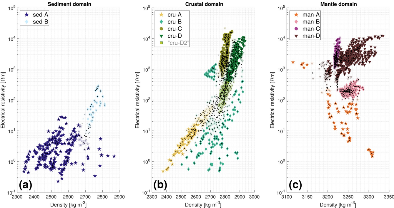
305 | Figure 3: Cross-plots of electrical resistivity and density and their identified clusters. Colour saturation of symbols is proportional to the posterior probability within Gaussian mixture model. Less saturated symbols depict decreased certainty of the cluster classification. Full saturation of symbols indicates a certainty above 90%, transparent symbols indicate a certainty between 60 and 80%, dots without color saturation indicate a certainty below 60%. (a): Sediment domain (depth extent defined by seismic models of Fromm et al. (2017a) and Planert et al. (2017)). (b): Crustal domain (depth extent defined as sediment basement to Moho derived from Laske et al. (2013) and Maystrenko et al. (2013)). Cluster “cru-D2” is manually defined by dividing the identified cluster cru-D horizontally at 400 \Omega\text{m} . (c): Mantle domain (below Moho).
