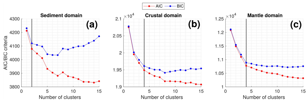
295 | Figure 2: Theoretical information criteria AIC (Akaike information criteria) and BIC (Bayesian information criteria) to determine the number of clusters in each of the three domains: (a) Sediment domain, (b) Crustal domain, (c) Mantle domain. The vertical black line marks the chosen number of clusters, which is two in the sediment domain, and four in the crustal- and mantle domain, respectively.
