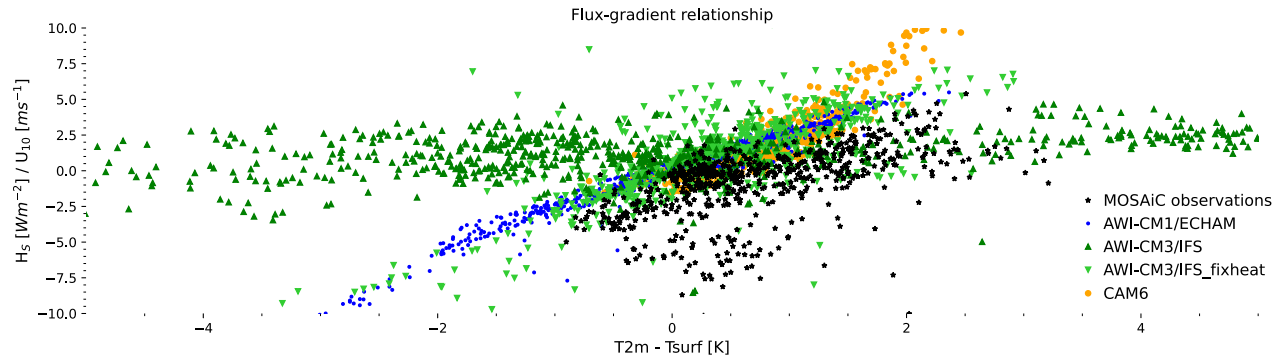
Figure 8. Relationship between near-surface temperature gradients and sensible heat fluxes (positive downwards) using hourly averages.
