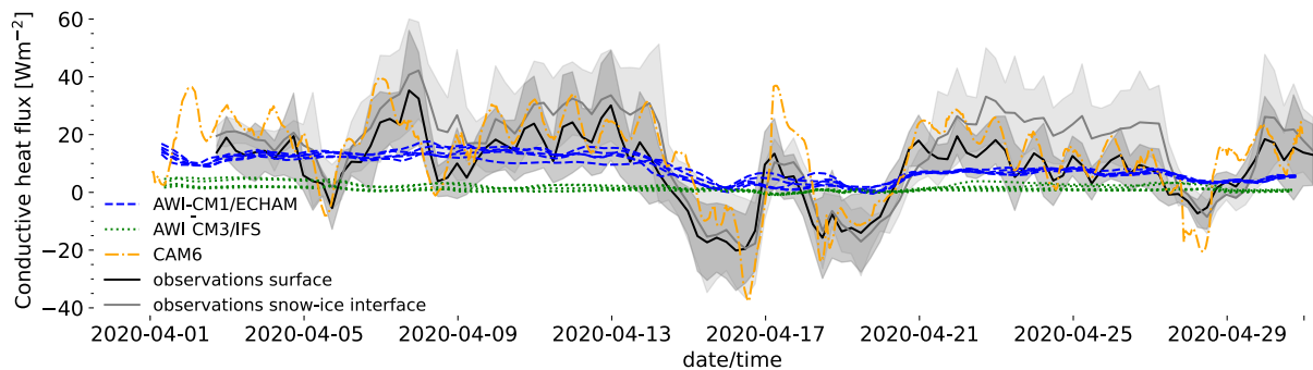
Figure 7. Observed and modelled 6-hourly conductive heat fluxes (positive towards the surface, i.e. upwards) during April 2020. Dotted lines show Grey shading shows the range of one standard deviation around the mean observational value. Note that measurements are for the uppermost snow layer at the surface and the snow-ice interface, whereas ECHAM data is for conductive heat flux through the ice. For CAM6, the heat flux between the snow surface and the atmosphere was reconstructed from the atmospheric fluxes at the surface.
