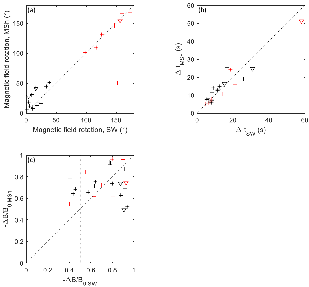
Figure 6. Magnetosheath values versus solar wind values for all 26 magnetic holes. Panel (a): magnetic field rotation across the magnetic hole, (b): temporal scale size, (c): magnetic field depth (with the limits of \Delta B/B_0 = -0.5 indicated). Black symbols represent linear magnetic holes, and red rotational holes. The triangles indicate heavier smoothing, as described in the main text.
