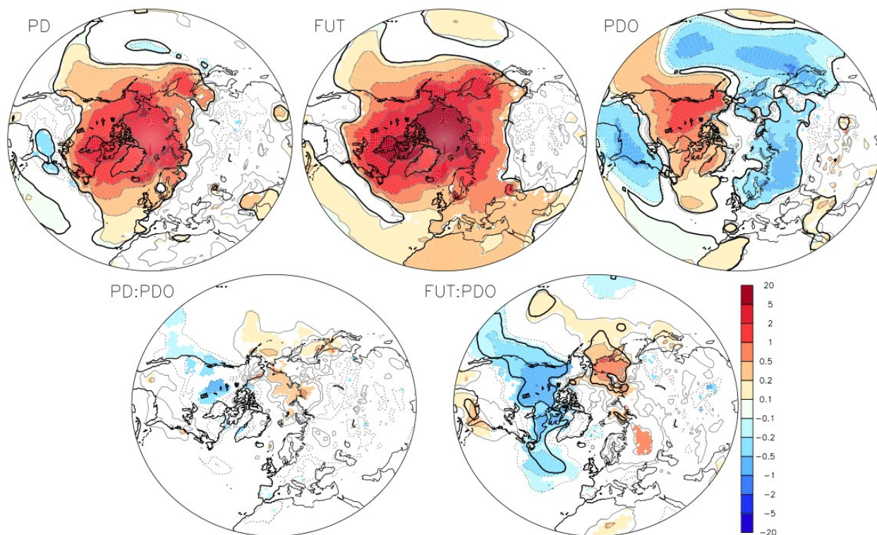
Figure 3: Surface air temperature at 2m (in °C) in response to sea-ice loss and PDO in the coupled simulations when using an analysis of the covariance: (top-left panel) effect of the PD sea-ice loss ( \beta_{PD} in Eq.(2)); (top-middle) effect of the FUT sea-ice loss ( \beta_{FUT} in Eq. (2)) (top-right) effect of a warm PDO ( \beta_{PDO} in Eq. (2)); (bottom-left) effect of the interaction between PD sea-ice loss and the PDO ( \beta_{PD:PDO} in Eq. (2), and (bottom-right) effect of the interaction between the FUT sea-ice loss and the PDO ( \beta_{FUT:PDO} in Eq. (2)). The color shades a p-value below 10%. The black line indicates field significance, as given by the false discovery rate.
