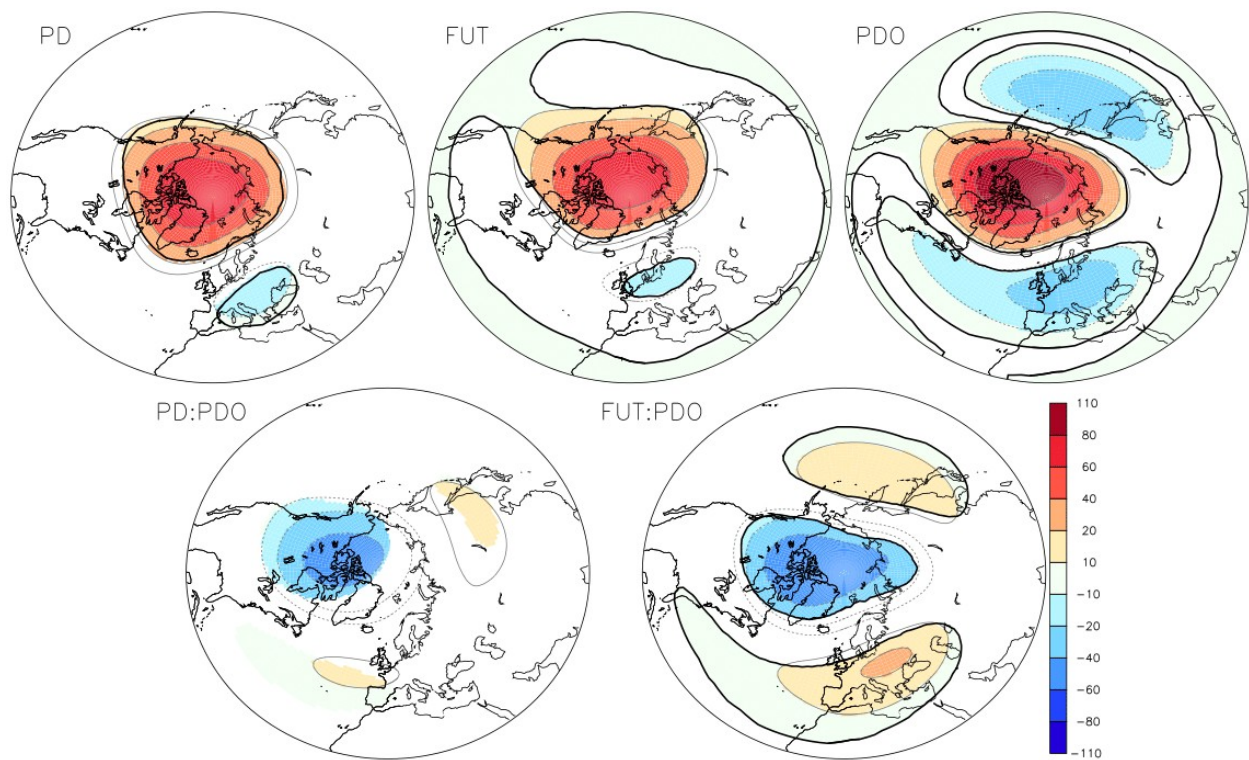
Figure 6: Same as Figure 3 but for geopotential height at 50 hPa, in m.
