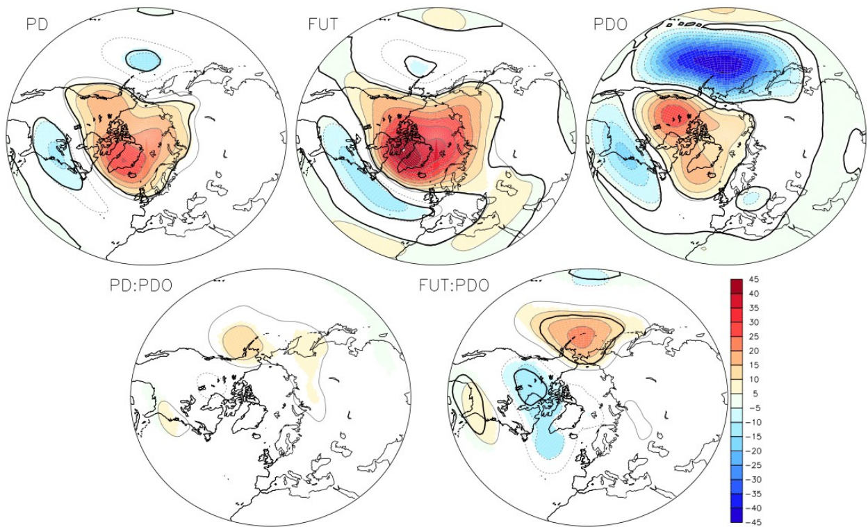
Figure 5: Same as Figure 3 but for geopotential height at 500 hPa, in m.
