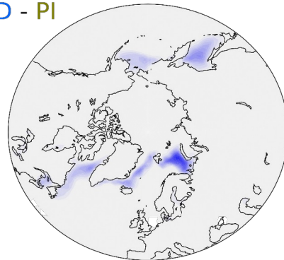
Figure 1: (Top) Arctic sea-ice area (in 10^6 km 2 ) for the ensemble mean of coupled model simulations using constrained SIC for (red, dash-dotted line) FUT, (blue, dotted line) PD and (green, dash line) PI. The corresponding target sea-ice is shown with solid lines. Vertical bars represent the 95% confidence interval for the ensemble mean. (Center) Simulated Arctic sea-ice concentration fraction changes in the coupled model ensembles for PI minus FUT and (Bottom) PI minus PD averaged from December to February.
