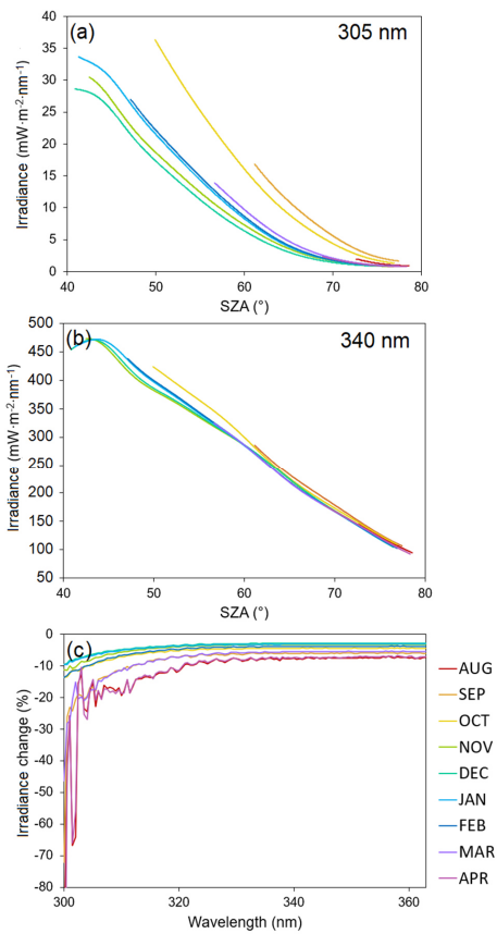
790 Figure 7: Modelled relationships between UV irradiance and SZA for individual different months, and mean absolute and relative changes in spectral UV irradiance caused by SZA change, while Panel (a) and (b) represents show the modelled SZA effect UV irradiance at 305 nm (a) and 340 nm, respectively, (b) as a function of SZA. Panel (c) and (d) modelled mean absolute and shows the relative change in spectral UV irradiance induced by a 1° resulting from an increase in SZA, while the relative changes were by 1°, calculated with reference to the monthly median spectra.
