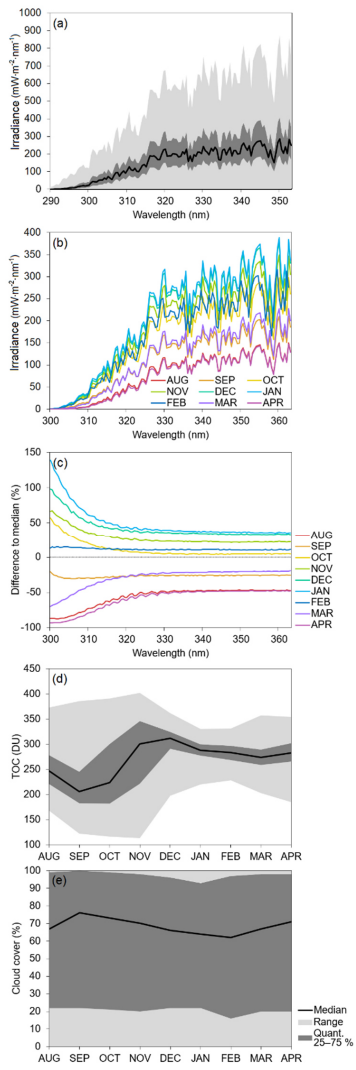
Figure 4: Observed solar UV spectra and variables related to them obtained at Marambio Base in 2010–2020, whilewhere (a) represents statistical characteristics of all spectra, (b) monthly medians, and (c) relative differences of monthly medians to overall median, and (d), and (e) show the climatology of TOC, and cloud cover, respectively.
