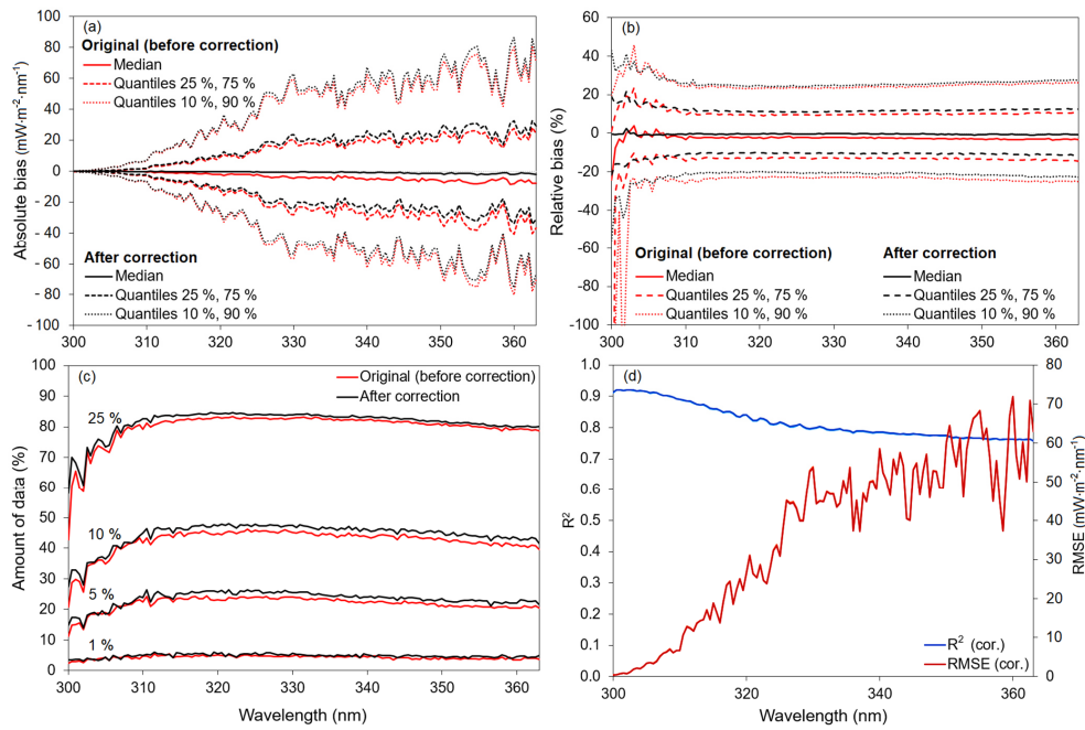
Figure 3: Validation of the ANN model before and after the median correction, where (a) represents the absolute bias quantiles, (b) are the relative bias quantiles, (c) is the amount of data within 1, 5, 10, and 25 % from observations, and (d) is the R-squared and RMSE.
