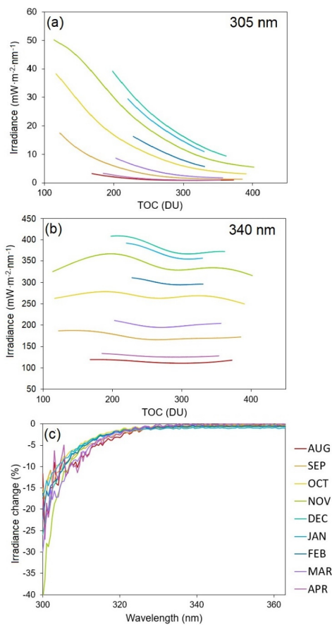
Figure 8: Modelled relationships between UV irradiance and TOC for individual different months, and mean absolute and relative changes in spectral UV irradiance caused by TOC change, while (a) and (b) represent, Panel (a) and (b) show the modelled TOC effect UV irradiance at 305 nm (a) and 340 nm, respectively; (b) as a function of TOC. Panel (c) and (d) modelled mean absolute and shows the relative change in spectral UV irradiance induced by a 10 DU resulting from an increase in TOC, while the relative changes were by 10 DU, calculated with reference to the monthly median spectra.
