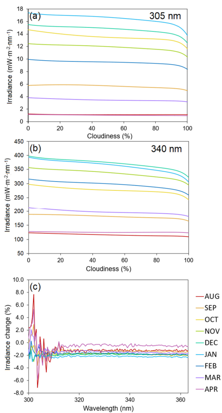
805 Figure 9: Modelled relationships between UV irradiance and cloudinesscloud cover for individualdifferent months, and mean absolute and relative changes in spectral. Panel (a) and (b) show the modelled UV irradiance caused by the change in cloudiness, while (a) and (b) represent the modelled effect of cloudiness at 305 nm (a) and 340 nm, respectively, (b) as a function of cloud cover. Panel (c) and (d) modelled mean absolute andshows the relative change in spectral UV irradiance induced by a resulting from an increase in cloud cover by 10 % increase in cloudiness, while the relative changes were%, calculated with reference to the monthly median spectra.
