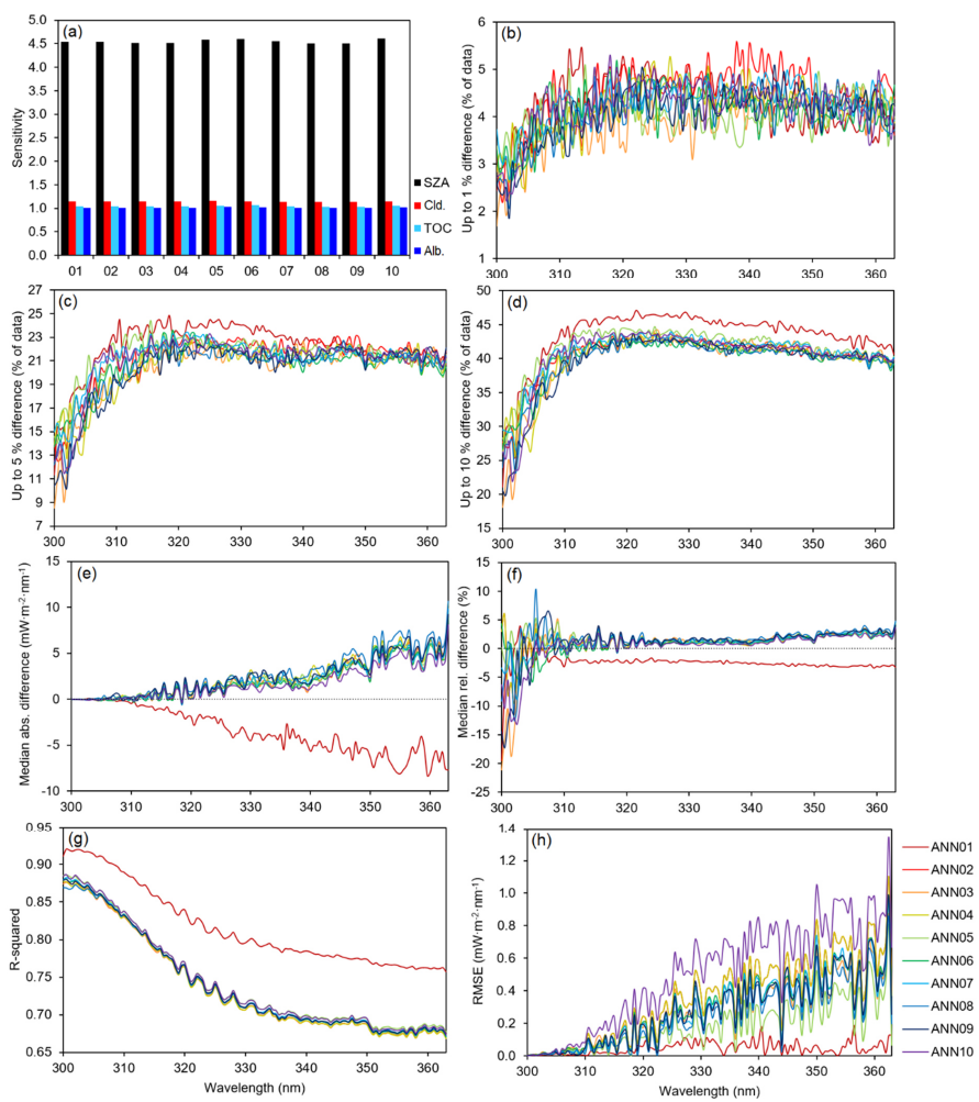
825 Figure A2: Development and validation of the 10 artificial neural network models, where (a) is the sensitivity of individual models to given variables; (b), (c) and (d) shows the amount of modelled data within 1, 5, and 10 % difference from observations, respectively; (e) and (f) are the absolute and relative median differences of the modelled data from the observations; (g) shows the R-squared, and (h) is the root mean square error of the individual models.
