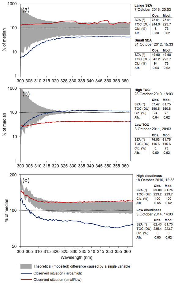
815 Figure 10: Spectral UV irradiance intensity relative to the monthly median on eight selected October days and the potential impact of selected variables (grey area) with extremely large/high or small/low (a) SZA, (b) TOC, and (c) cloudiness/cloud cover at Marambio Base in 2010–2020. The dissimilarities between the model output, where three out of four explanatory variables were set to their monthly median, and the actual observation, shows the combined impact of the three variables that were set to their medians in the model and whose values are shown in the tables on the right.
