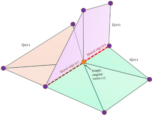
Figure 6: A representation of simple singular vertex (v) (Moulaeifard et al., 2023).
