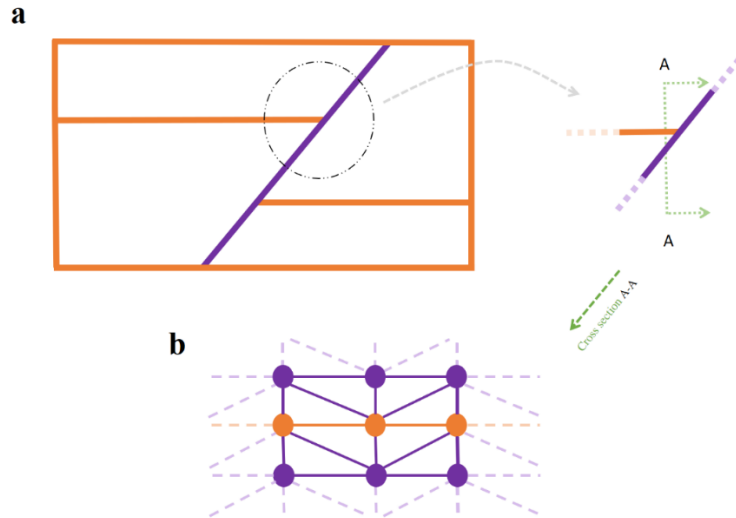
Figure 5: (a) A schematic representation of the intersection between a fault and a layer; (b) Mesh structure of the surface intersection includes the simple singular vertices (brown circles).
