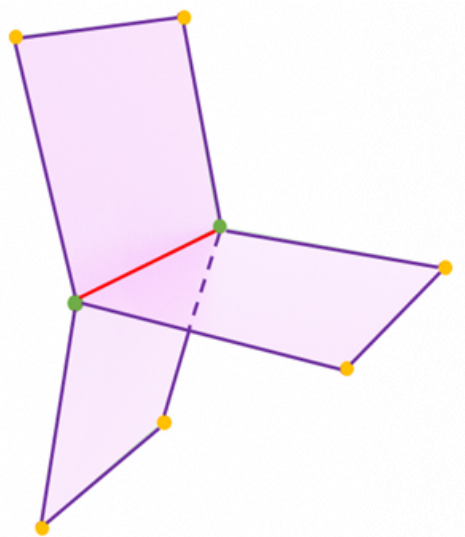
Figure 1: A common example of a non-manifold topology in geological modelling; multiple faces share one edge. Non-manifold vertices (green) and edge (red).
