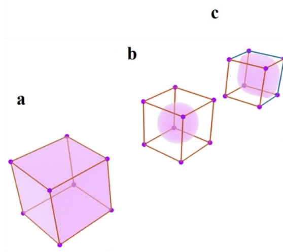
Figure 4: Generating creases on a mesh by applying three times subdivision surface algorithm (Moulaeifard et al., 2023); (a) Control mesh (b); All edges of the control mesh are smooth edges (red edges); (c) Four edges are crease edges (blue edges), and nine edges are smooth (red edges).
