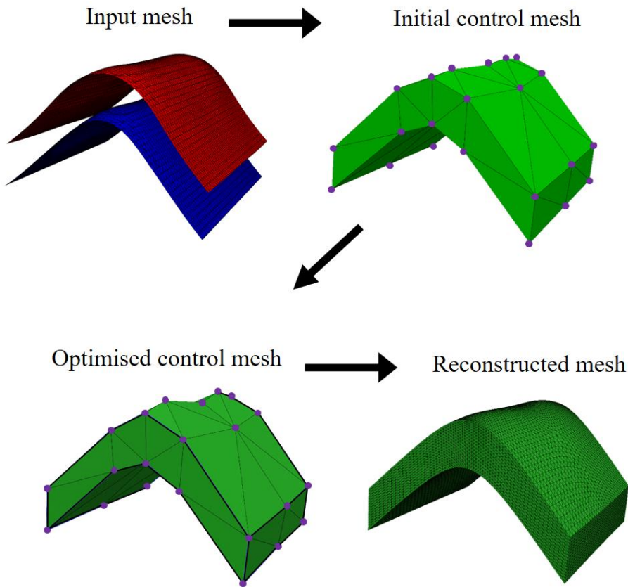
Figure 7: General workflow of subdivision surface fitting with an example of an anticlinal structure.
