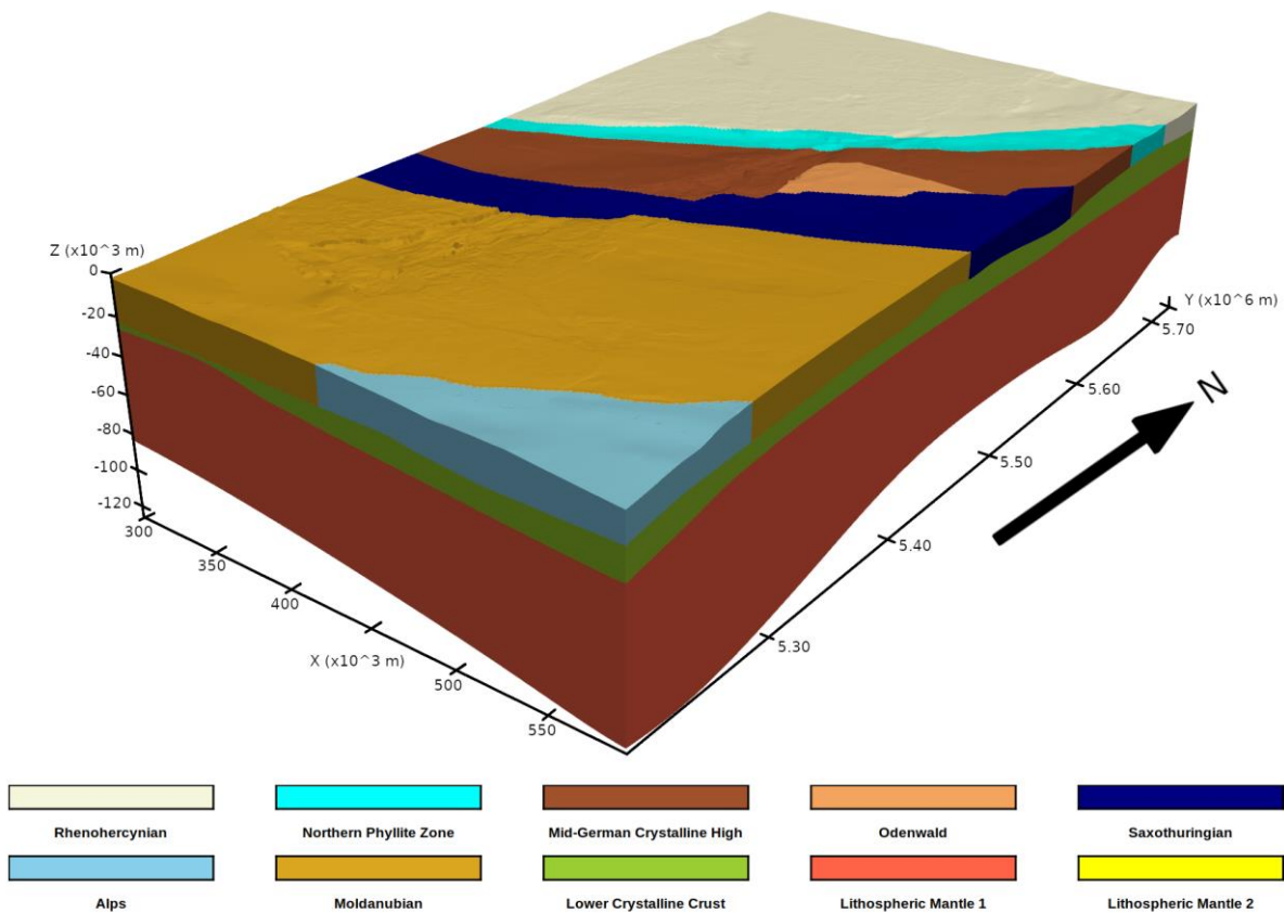
Figure 12: Grid-based representation of part of URG model which contains 616464 individual nodes and 10 different volumes generated based on the data of Freymark et al. (2020).
