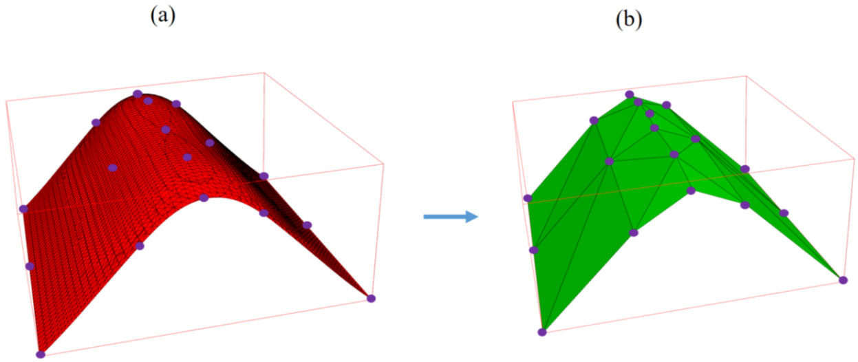
Figure 10: (a) Control points are generated based on the vertices of the input mesh; (b) Triangulated control mesh is constructed based on the control points and the Delaunay triangulation.
