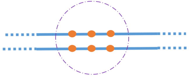
Figure 15: Distinguishing different parts of the surface by adding control points to avoid failure in the reconstruction process.
