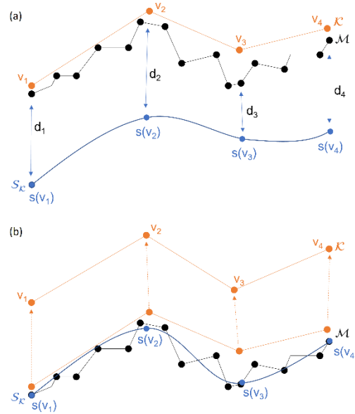
Figure 8: Synthesized and conceptualized approach for surface fitting with subdivision surfaces.
