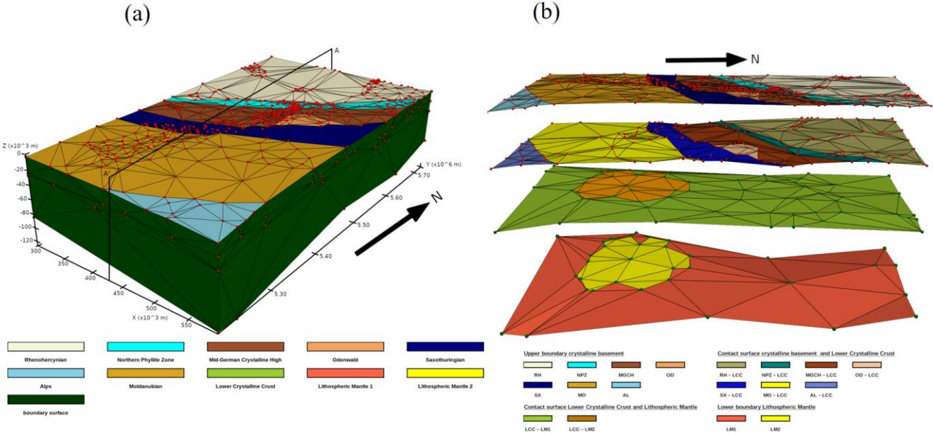
Figure 13: (a) Initial and unfitted control mesh of the URG model. Surfaces are coloured concerning the different geological units. The surfaces of the Lower Crystalline Crust and the Lithosphere mantle are hidden by the boundary surface. The 832 control points are coloured in red; (b) Approximately representation of the 3D side view of the model along the profile AA'.
