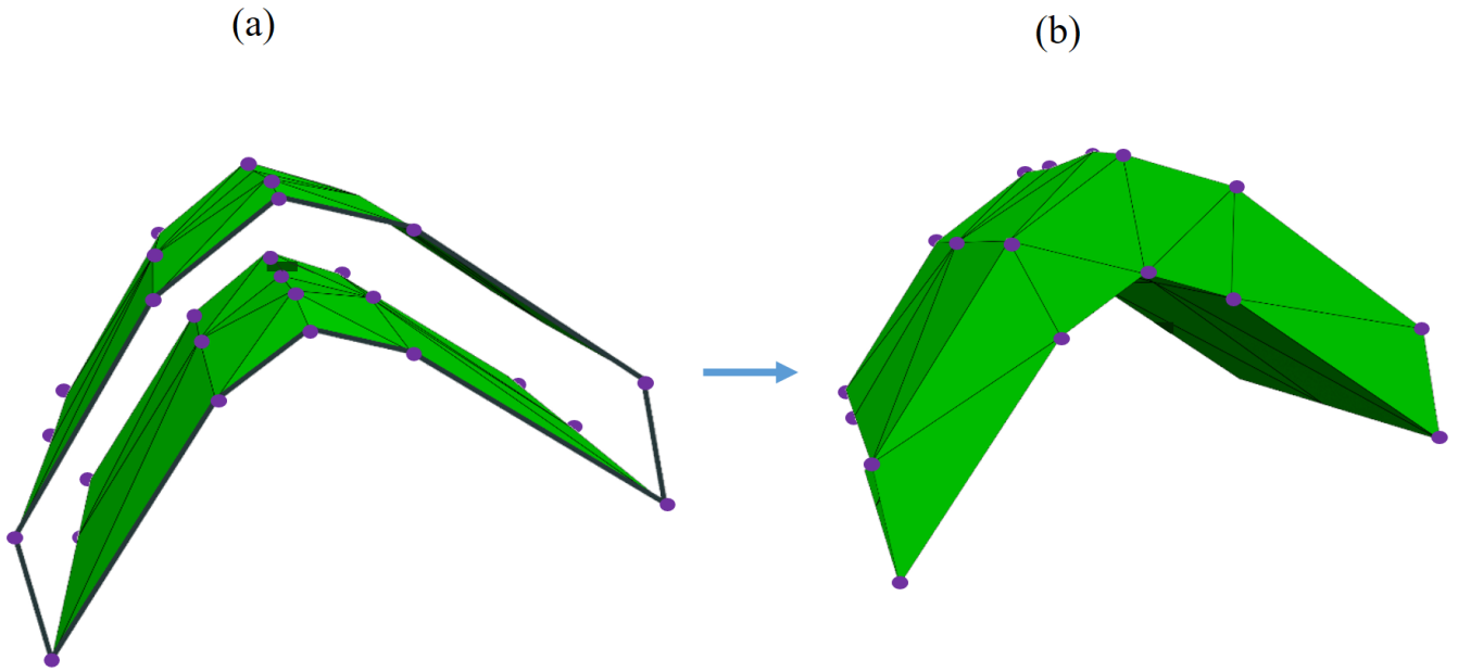
Figure 11: (a) Stitching and merging the different parts of the control mesh to make it watertight ; (b) Final watertight control mesh
