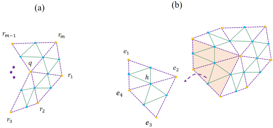
125 Figure 3: Averaging step of generating the smooth surface by Loop subdivision scheme; (a) Updating the position of the existing 130 vertices; (b) Updating the position of the new midpoint vertices.
