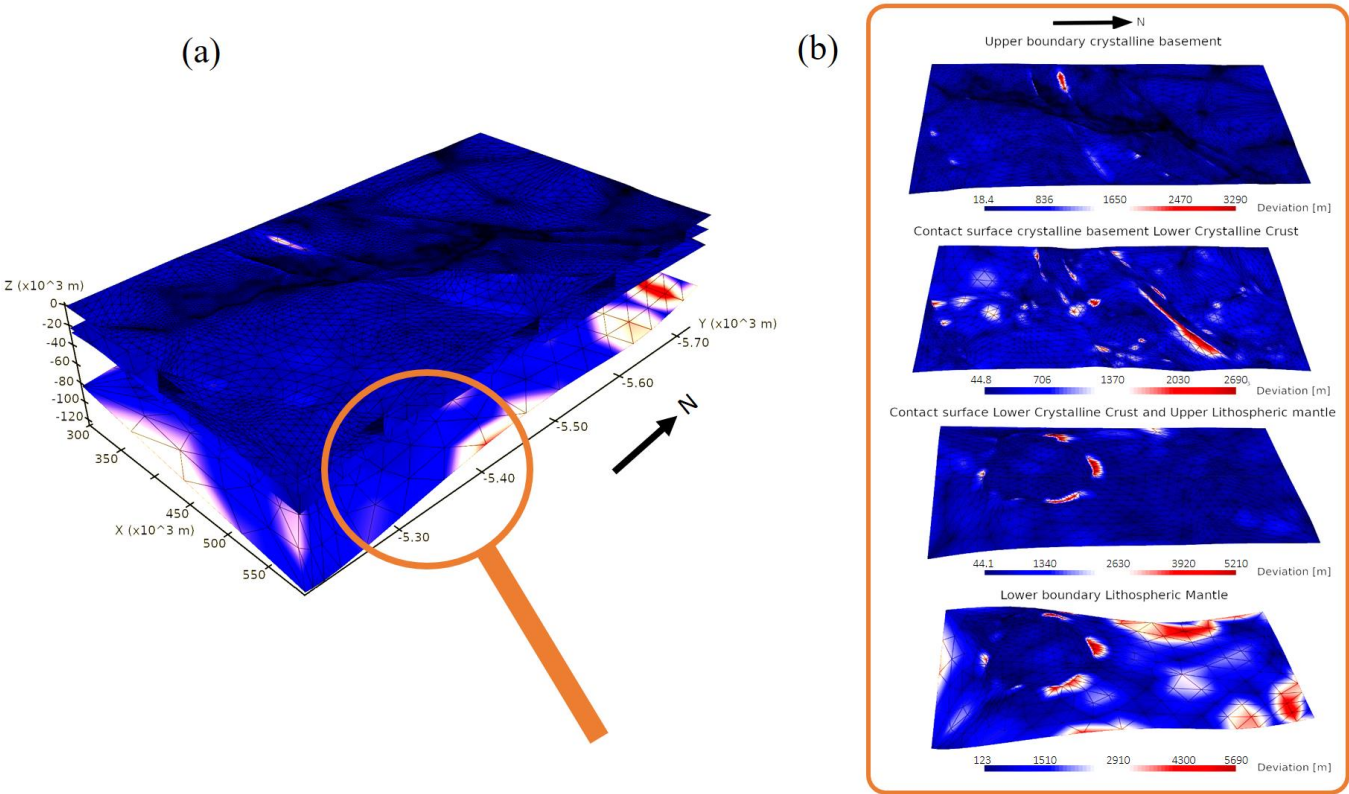
375 Figure 14: (a) Distance map of the subdivided surfaces compared to the input mesh (Fig. 12). Red areas indicate high deviation from the original input mesh while blue areas indicate low deviation; (b) Exploded view on the distance map of the four extracted sub- horizontal layers. Distances are scaled for each layer individually to emphasize the areas of high and low errors independent of the maximal global error.
