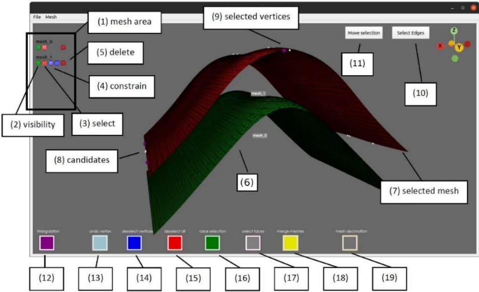
Figure 9: The GUI of PySubdiv allows the user to construct the control mesh for the (geological) model. The important GUI elements are labelled and explained in the following.
