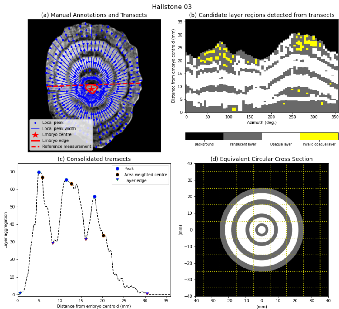
Figure 3. Demonstration of analysis procedure for hailstone 3: (a) manual annotations (red elements) and layer peak detection along radial transects (blue elements), (b) Transect analysis shown in the azimuth-range space, (c) Detection of layers from consolidated transect analysis, (d) Equivalent circular hailstone cross section where wet and dry growth is represented by gray and white shading respectively.
