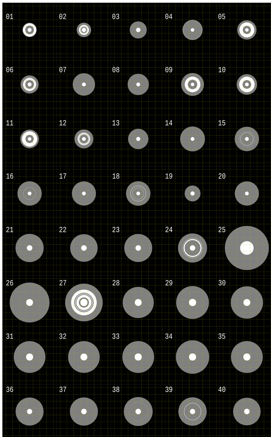
Figure 8. Circular hailstone cross sections generated from the ‘umax31’ storm of Kumjian and Lombardo (2020). White-shaded regions represents opaque dry-growth layers and gray shaded regions indicate translucent wet-growth layers. Grid lines shown at a 1 cm spacing starting from 0.5 cm from the embryo centroid.
