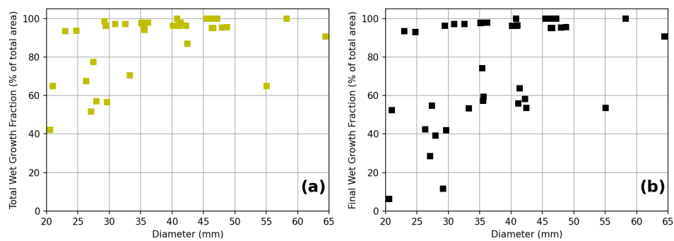
Figure 9. Hailstone properties derived from the ‘umax31’ storm of Kumjian and Lombardo (2020) as a function of diameter. These properties include the wet growth across the hailstone cross section as a fraction of the total area and the final wet growth layer as a fraction of the total area.
