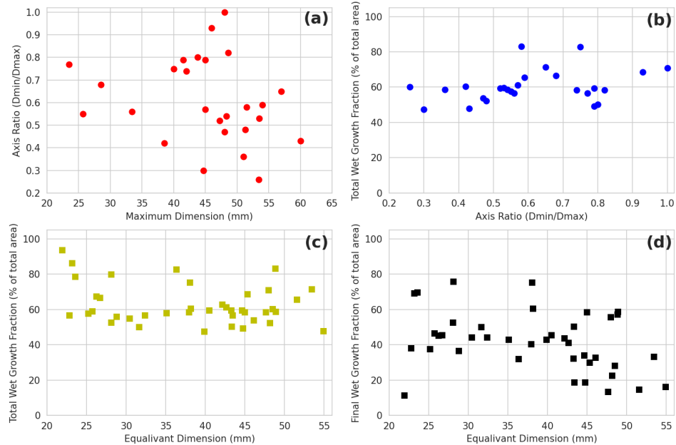
Figure 6. Hailstone properties derived from the LAT and manual measurements. Layer analysis technique derived properties include the wet growth across the hailstone cross section as a fraction of the total area and the final wet growth layer as a fraction of the total area. Equivalent dimension was calculated from an oblate spheroid model using the maximum and intermediate dimensions. Note that the minimum dimension used to calculate axis ratio was not measured for all hailstones and therefore panels (a) and (b) have a reduced sample size of 26 compared to the complete collection of 40 hailstones used in panels (c) and (d).
