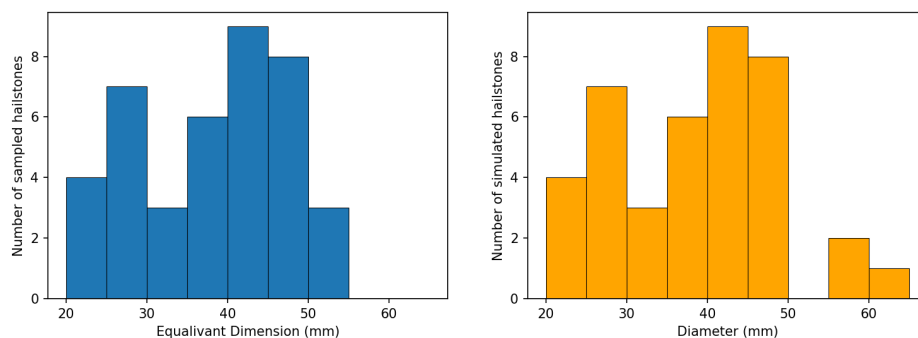
Figure 7. Equivalent dimension (oblate spheroid approximation using maximum and intermediate dimensions) distribution for hailstones observed for the Melbourne hailstorm (left) and diameter distribution of those simulated by the hail growth and trajectory model (right).
