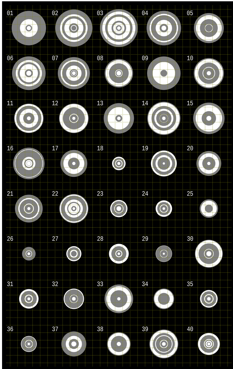
Figure 5. Equivalent circular hailstone cross sections generated from the layer analysis technique. White-shaded regions represents opaque dry-growth layers and gray shaded regions indicate translucent wet-growth layers. Grid lines shown at a 1 cm spacing starting from 0.5 cm from the embryo centroid.
