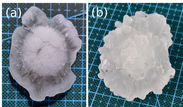
Figure 1. Examples of the two main hailstone shapes observed: (a) highly oblate, partly melted hailstones without lobes, (b) larger, approximately-spherical opaque hailstones covered in many small lobes. Photographs were captured prior to the extraction of cross sections. These hailstones are identified as numbers 5 and 4 respectively in subsequent figures.
