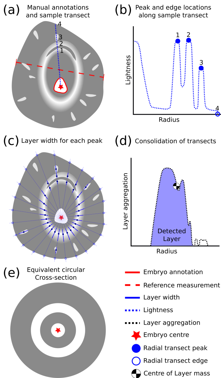
Figure 2. Conceptual diagram of analysis procedure: (a) manual annotations and sample transect with 3 peaks marked (1,2,3) and the edge location (4), (b) Representation of transect in radius-lightness space with peaks and edge marked from (a), (c) Measurement of layer width for each peak detected, (d) detected layer centre of mass from consolidated transect analysis, (e) Equivalent circular hailstone cross section where wet and dry growth is represented by gray and white shading, respectively.
