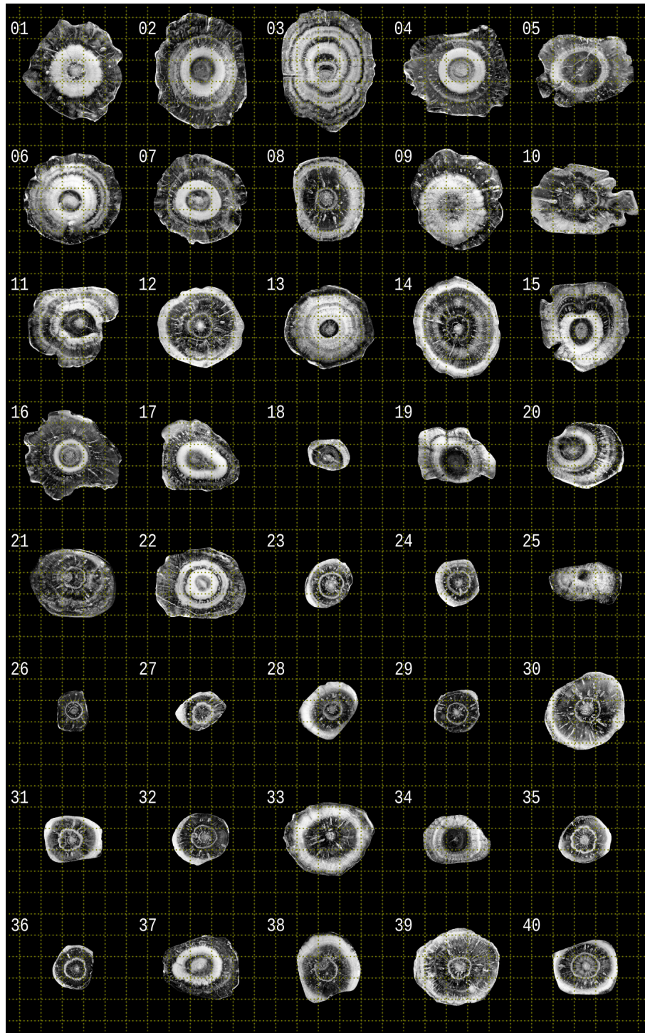
Figure 4. Hailstone cross sections from the Melbourne hailstorm event (19 January 2020). Grid lines shown at a 1 cm spacing.
