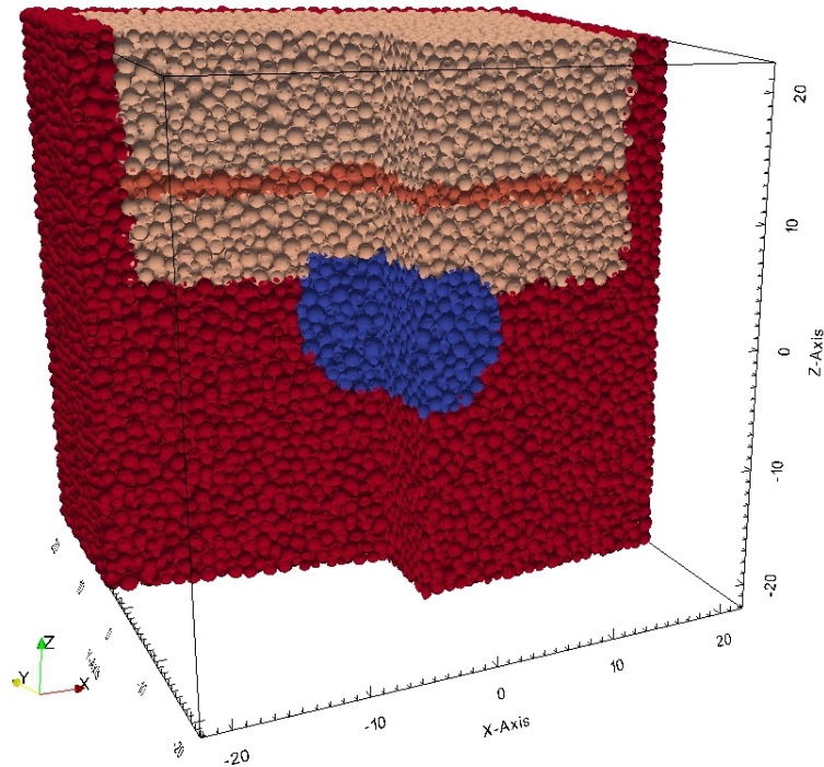
Figure 10. Setup of YADE mechanical model. The model is 50x50x50 m in size and filled with spheres irregularly packed. The colors of the sphere represent different layers: Upper peri-glacial sand (light brown), glacial till (orange), lower peri-glacial sand (light brown), chalk (red). Note that the sides of the modelling domain (also shown in red) are fixed.
