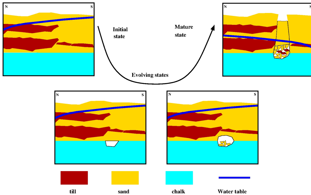
Figure 12. Evolution of collapse sinkhole. Light blue colours indicate chalk as soluble rock, yellow colours peri-glacial sand and brownish colours glacial till, the latter two as insoluble rocks. The dark blue line is the hypothetical water table, and the white area a void in the chalk.
