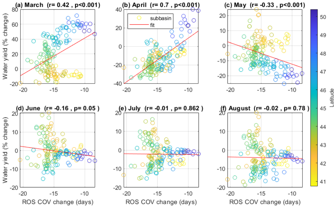
Figure 9. Correlations of the change in the center-of-volume (COV) for rain-on-snow melt events between the historic 1960-1999 period and mid-21 st century, with the percent change in monthly water yield during that time, for spring and summer months. Markers represent projections of the RCP 4.5 ensemble mean for individual major river basins. Colors are coded with the latitudinal gradient. The water year lasts from 1 October to 30 September.
