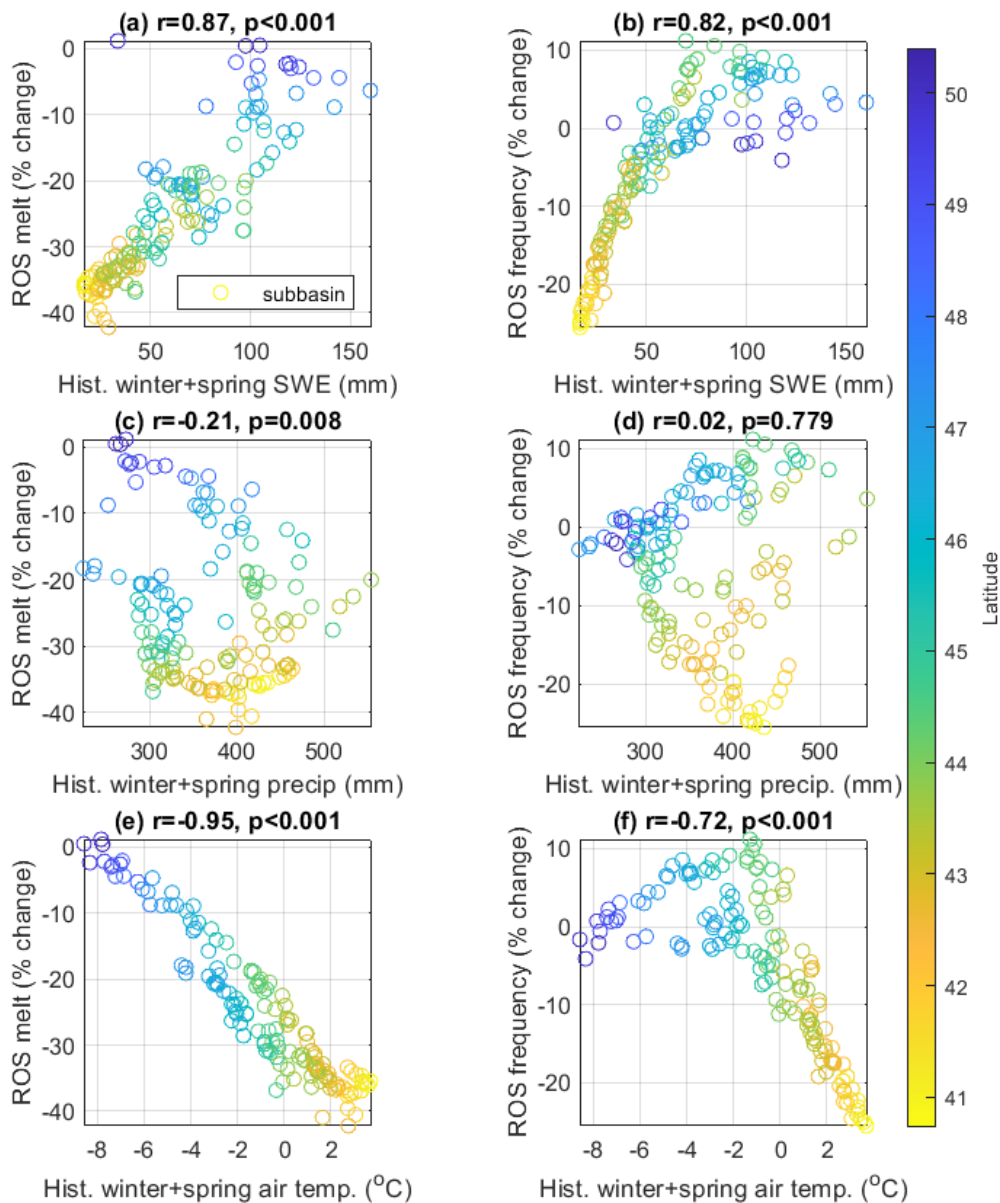
Figure 8. Relationships between the historic 1960-1999 conditions and the percent change from the historic period to mid-21 st century for RCP 4.5 ensemble means. A) historic winter+spring snow water equivalent (SWE) and rain on snow (ROS) melt amount change, b) historic winter+spring SWE and ROS frequency change, c) historic winter+spring precipitation and ROS melt change, d) historic winter+spring precipitation and ROS frequency change, e) historic winter+spring air temperature and ROS melt change, and f) historic winter+spring air temperature and ROS frequency change. Colors are coded with the latitudinal gradient.
