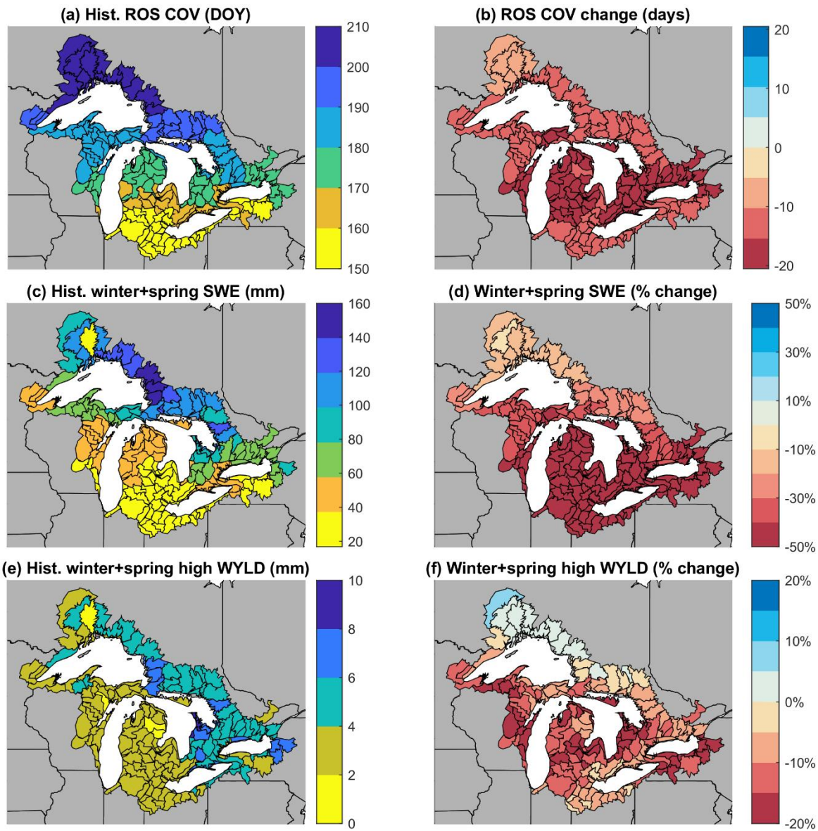
230 Figure 7. Changes in (a and b) the center of volume (COV) for rain-on-snow-melt (ROS) events (the day of the water year [DOY] when | half the total annual rain-on-snow melt is passed), (c and d) daily mean winter+spring snowpack SWE, and (e and f) high (0.95 quantile) | daily winter+spring water yields (abbreviated WYLD for brevity ) between the historic 1960-1999 period and mid-21 st century. Left panels indicate historic conditions, while right panels indicate percent changes. Projections represent the RCP 4.5 ensemble mean. The water year lasts from 1 October to 30 September.
