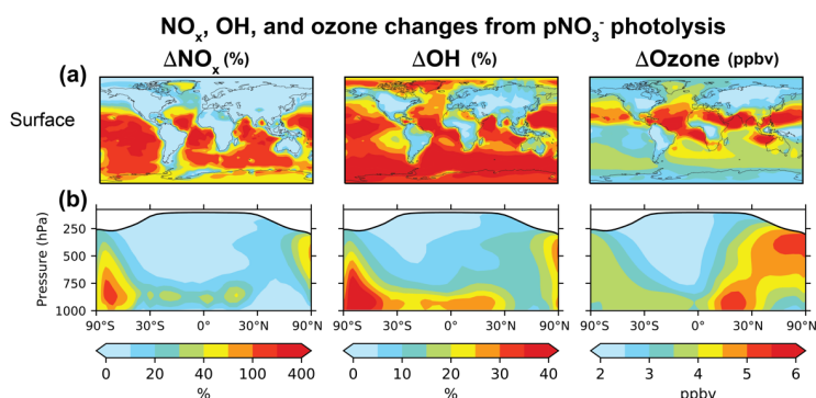
Figure 7. Annual mean (2015) changes in \text{NO}_x , OH, and ozone concentrations from including \text{pNO}_3^- photolysis in GEOS-Chem. Panel (a) shows changes at the surface and panel (b) shows the zonal means. Changes in \text{NO}_x and OH are shown as percent change of concentrations in our baseline simulation relative to that in the sensitivity simulation without \text{pNO}_3^- photolysis, and changes in ozone are shown as differences in concentrations (in ppbv) between the two simulations. The white shading in the zonal mean plots denotes the stratosphere.
