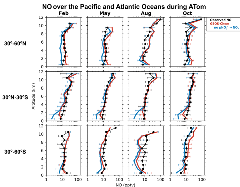
Figure 3. Median vertical profiles of \text{NO} concentrations over the Pacific and Atlantic Oceans during the ATom flight campaigns (2016–18), separated by seasons and latitude bands. Observations (black) are from the NOAA P-CL instrument. The data selection criteria are as described in the caption of Fig. 1. Horizontal bars show the interquartile ranges in 1-km altitude bins. Model results are from our baseline GEOS-Chem simulation and a sensitivity simulation without \text{pNO}_3 photolysis. The model is sampled along the flight tracks. \text{NO} concentrations are plotted on a log scale to show the values in the lower troposphere clearly.
