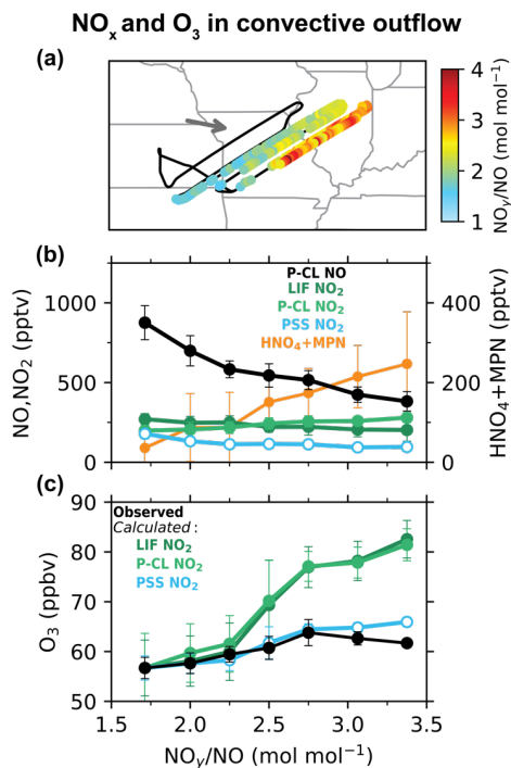
Figure 2. Evolution of NO x and O 3 concentrations in a thunderstorm outflow targeted for quasi-Lagrangian sampling by DC3 flight 17 over the central US at 12 km altitude. Panel (a) shows the flight track with data points within the outflow colored by the observed NO y /NO ratio as a measure of chemical aging. The arrow shows the mean wind direction. Panel (b) shows the measured concentrations of NO, NO 2 and the sum of HNO 4 and MPN as a function of the NO y /NO molar ratio. Also shown are the PSS NO 2 concentrations (Eq. 3). Panel (c) shows the measured ozone concentrations as a function of the NO y /NO molar ratio along with the ozone concentrations calculated from Eq. (4) with NO 2 concentrations from LIF, P-CL, or PSS NO 2 . The circles and the error bars in panels (b) and (c) show means and standard deviations for each NO y /NO bin.
