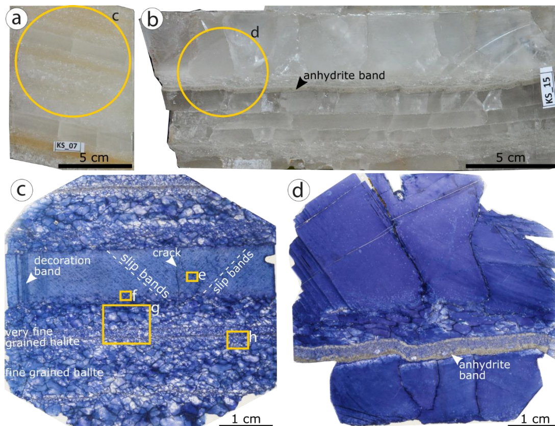
675 Figure 2: a) Reflected light photograph of slabs (KS-07 from Barradeel) used for microstructural analysis showing layered white and honey colored salt with variable grain sizes and milky Kristallagen with internal lamination. b) Slab specimen KS-15 of 680 Barradeel used for microstructural analysis showing layered transparent and white salt with Kristallagen up to 5 cm thicknesses with cracks. Small fold in 5 mm thick anhydrite band is bend following the displaced crystal layer. c) overview of gamma decorated thin section of sample KS-07 in transmitted light (location indicated in a) showing Kristallagen with abundant inclusions and decorated slip bands, dark blue decorated bands parallel to crack and layers of fine and very fine-grained halite with white cores and blue rims. d) overview of gamma decorated thin section of sample KS-15 in transmitted light (location indicated in b)) showing inclusion poor crystal layers that are slightly displaced and layers of fine-grained halite, with some grains showing a white overgrowth. Anhydrite-halite band is slightly bent and contains abundant halite mineral inclusions of up to 2mm.
