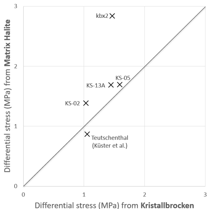
745 Figure 10: Comparison of differential stresses measured in Kristallbrocken and matrix halite, for samples were both were available ( \sigma = 107 * (D^{-0.87}) , D= subgrain size, (Carter et al., 1993; Schléder and Urai, 2005)). Measurements indicate comparable differential stresses for both halite types, but slightly lower values for differential stress in Kristallbrocken of this study. Differential stresses from Teutschenthal were measured based on micrographs presented in Küster et al. (2008) for matrix halite and Küster (2011) for Kristallbrocken and show comparable, slightly lower differential stresses.
