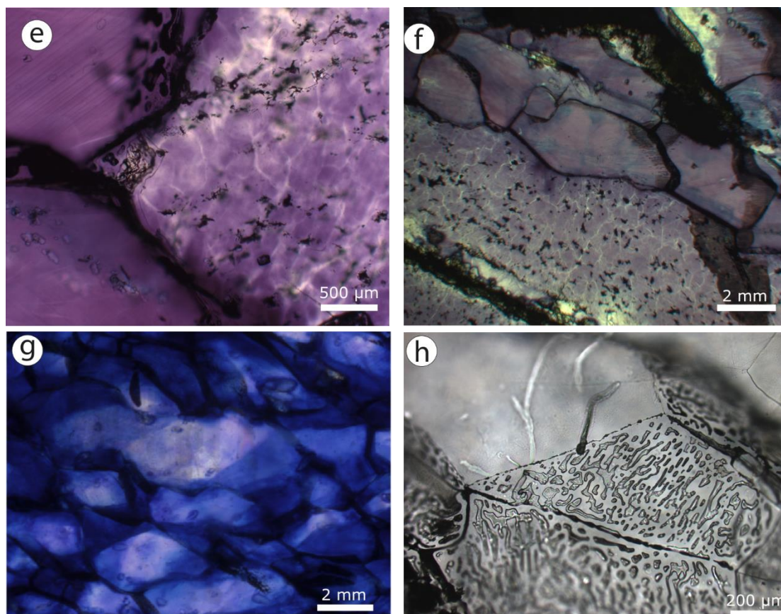
710 Figure 5: e) Transmitted light micrograph of gamma irradiated sample KS-13B (Zuidwending) showing Kristallbrocken grain with gamma decorated subgrains and abundant solid inclusions. Clear halite grain shows array of elongated anhydrite minerals parallel to grain boundary as well as abundant fluid inclusions at grain boundaries. f) Transmitted light micrograph of gamma irradiated Zuidwending sample KS-02 showing subgrain structures, abundant dark inclusions as well as clear elongated halite grains next to it. g) Transmitted light micrograph of gamma decorated halite grains showing light cores and directional overgrowth of elongated fine-grained halite in sample BS-B (Pieterburen). h) Transmitted light micrograph of thick section 715 showing abundant fluid inclusions at fine-grained halite grain boundary of Pieterburen sample.
