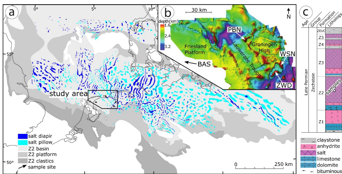
670 Figure 1: a) Zechstein salt structures in the Permian basin and Z2 carbonate facies distribution after (Laier, T. et al., 1998; Geluk, 2000). b) Study area (indicated in (a)) after Strozyk et al., (2014) showing top salt depth from seismic interpretation and well locations. BAS=Barradeel, PBN=Pieterburen, WSN=Winschoten and ZWD=Zuidwending. c) Stratigraphy of Zechstein salt in the Netherlands after Geluk et al. (2007) with stratigraphic position of studied samples.
