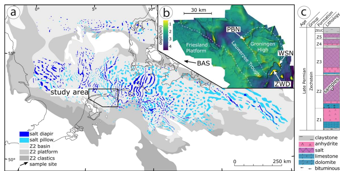
680 Figure 1: a) Zechstein salt structures in the Permian basin and Z2 carbonate facies distribution after (Laier, T. et al., 1998; Geluk, 2000). b) Study area (indicated in (a)) after Strozyk et al., (2014) showing top salt depth from seismic interpretation and well locations. BAS=Barradeel, PBN=Pieterburen, WSN=Winschoten and ZWD=Zuidwending. c) Stratigraphy of Zechstein salt in the Netherlands after Geluk et al. (2007) with stratigraphic position of studied samples.
