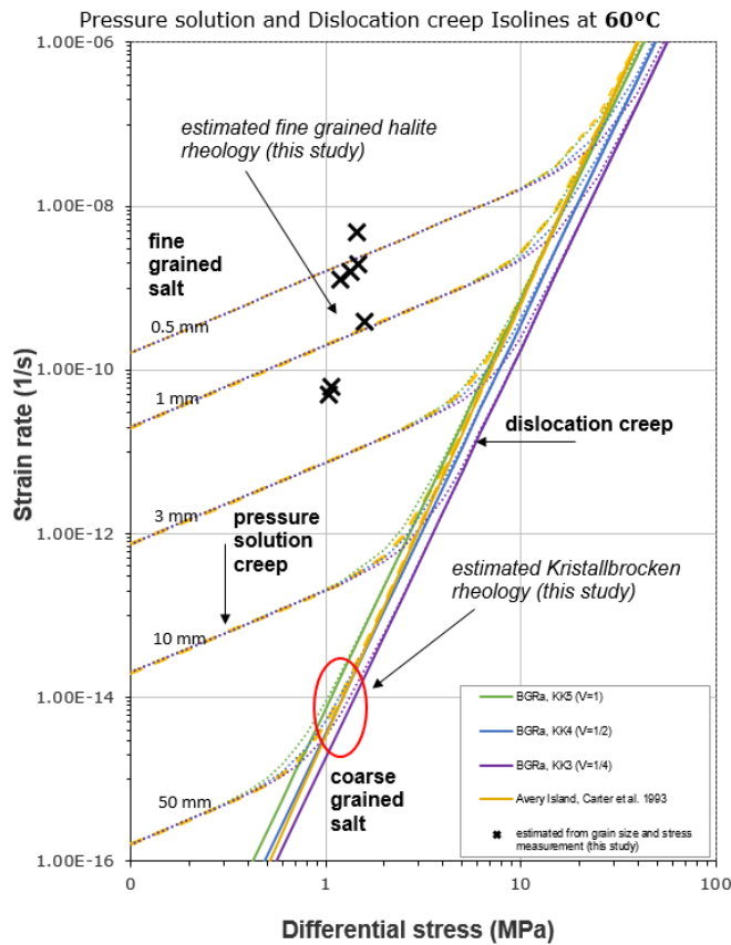
785 Figure 9: Differential stress vs strain rate diagram plotting selected flow laws at 60°C. For dislocation creep BGRa KK='Kriechklassen' 5, 4 and 3 calculated with Eq. 1, A = 2.083 \times 10^{-6} \text{ s}^{-1} , Q_{DC} = 54 \frac{\text{kJ}}{\text{mol}} and n = 5 (Liu, W. et al., 2017) as well as Avery Island samples calculated with Eq. 1, A = 1.6 \times 10^{-4} \text{ s}^{-1} , Q_{DC} = 68 \frac{\text{kJ}}{\text{mol}} and n = 5.3 from (Carter et al., 1993) are included for dislocation creep. Dotted lines show combined pressure solution (Spiers et al., 1990) and dislocation creep flow laws for different halite grain sizes calculated with Eq. 2, previous values for dislocation creep and B = 4.7 \times 10^{-4} \text{ s}^{-1} , Q_{PS} = 24.53 \frac{\text{kJ}}{\text{mol}} and m = 3 790 (Spiers et al., 1990). Results from this study are plotted based on measured median fine-grained halite grain sizes (Fig. 7) and differential stresses from subgrain size piezometry of Kristallbrocken for each sample (Supplement 2 and Table 1).
