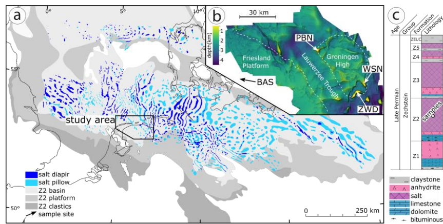
Figure 1: a) Zechstein salt structures in the Permian basin and Z2 carbonate facies distribution after (Laier, T. et al., 1998; Geluk, 2000). b) Study area (indicated in (a)) after Strozyk et al., (2014) showing top salt depth from seismic interpretation and well locations. BAS=Barradeel, PBN=Pieterburen, WSN=Winschoten and ZWD=Zuidwending. c) Stratigraphy of Zechstein salt in the Netherlands after Geluk et al. (2007) with stratigraphic position of studied samples.
