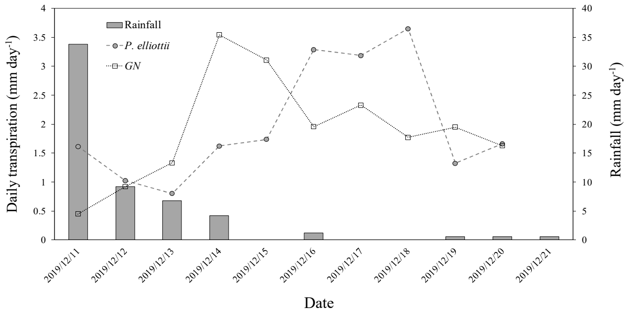
Figure 8. Ten-day daily transpiration (mm day -1 ) for 20-year-old P. elliotii and 8-year-old Eucalyptus grandis x Eucalyptus nitens clonal hybrid (GN) with corresponding rainfall (mm day -1 ) showing transpiration response by each specie to rainfall.
