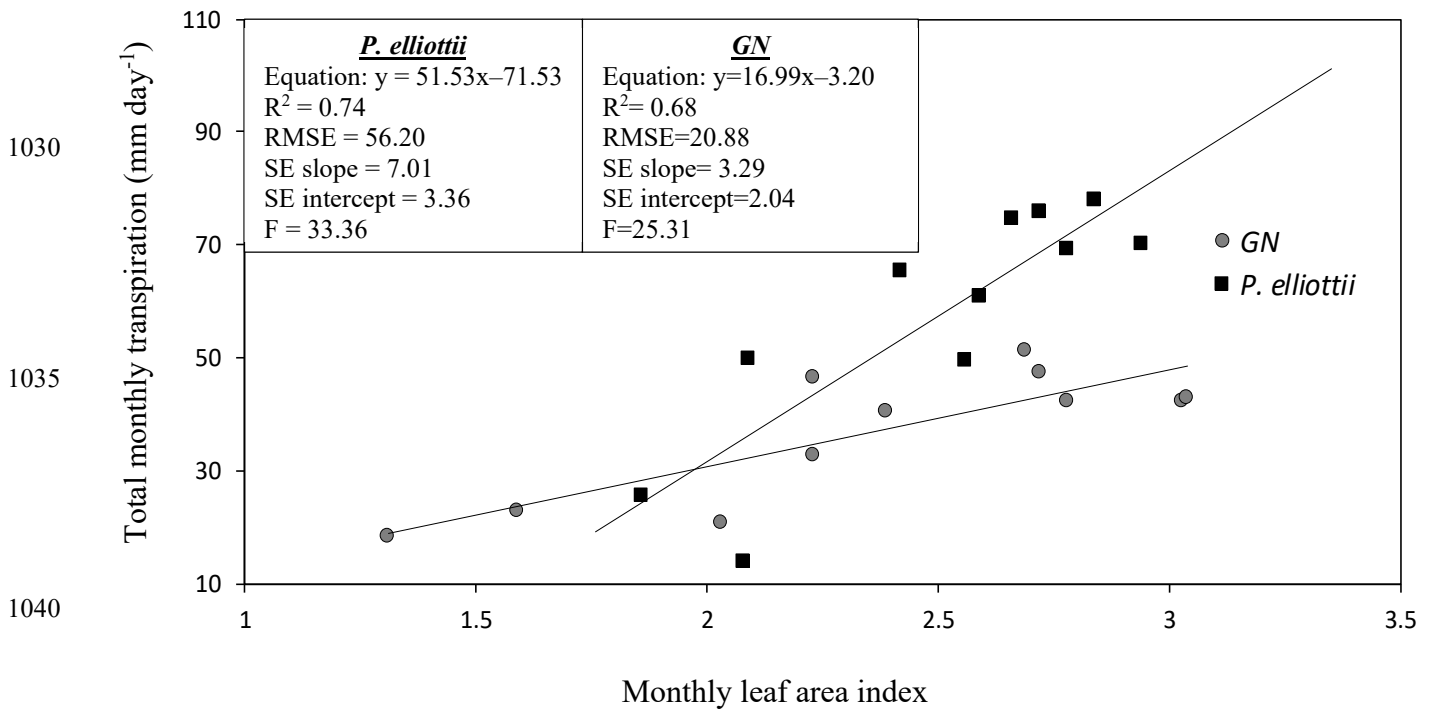
Figure 12. A linear relationship between total monthly transpiration ( T , mm day -1 ) and monthly measured leaf area index (LAI) for Eucalyptus grandis x E. nitens clonal hybrid ( GN ) and Pinus elliotii . The equation of the regression line, regression coefficient ( R^2 ), root mean square error (RMSE), the standard error of the regression slope (SE slope), the standard error of the y- intercept (SE intercept) and the ratio of variance (F) for each species is presented.
