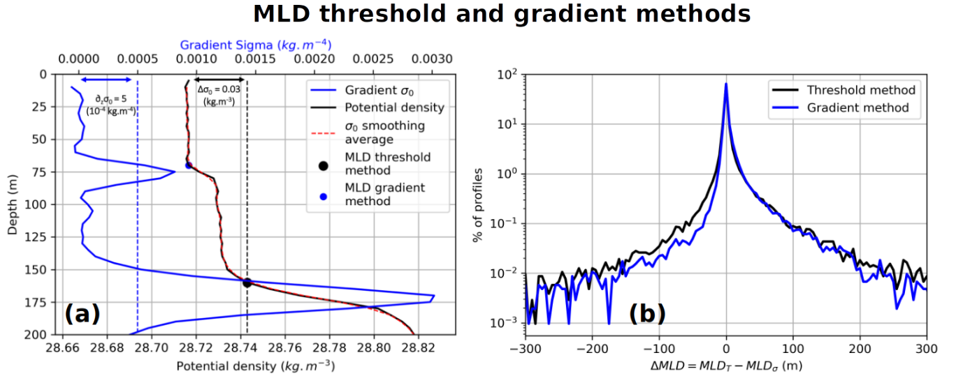
Figure 1. (a) MLD detection on one potential density profile with our gradient method (blue dot) and threshold method (black dot) and (b) fraction of the profiles as a function of \Delta \text{MLD} for the threshold (black line) and gradient (blue line) method
