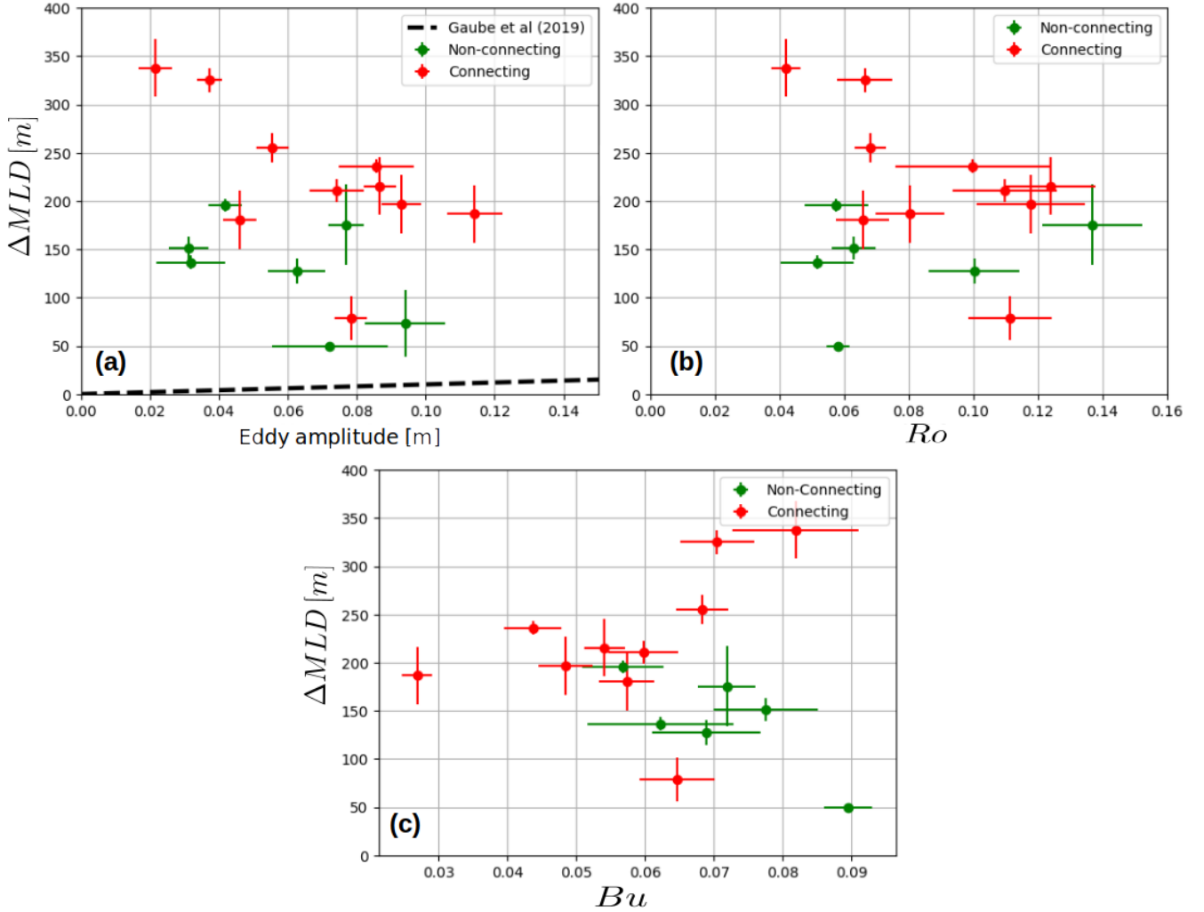
Figure 7. Relationship between maximal MLD anomaly ( \Delta MLD ) and eddy parameters possibly measured through remote sensing : (a) eddy SSH amplitude, compared with proposed 1m MLD for 1cm SSH relation (Gaubé et al., 2019), (b) Rossby number (eddy intensity), and (c) Burger number (non-dimensional eddy size).
