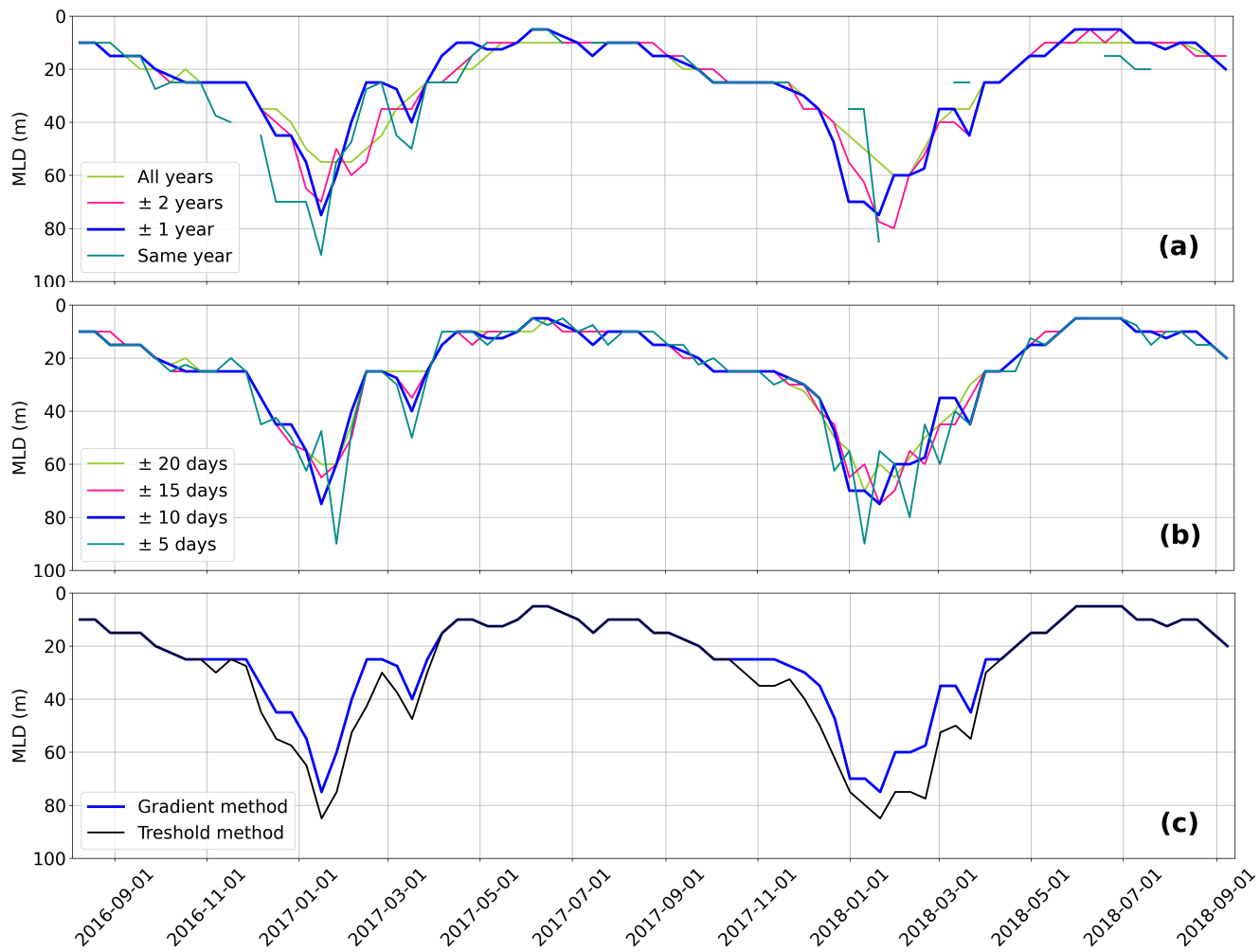
Figure A1. Sensitivity of the background MLD on the different parameters for events IER1-2 (see Table1 and Fig.10a) : (a) \Delta y (year interval) and (b) \Delta day (day interval). (c) Sensitivity to the MLD computation method. The background MLD method used throughout this study is \Delta day = 10 days, \Delta y = 1 year and the gradient method (common navy blue line on panels a-c).
