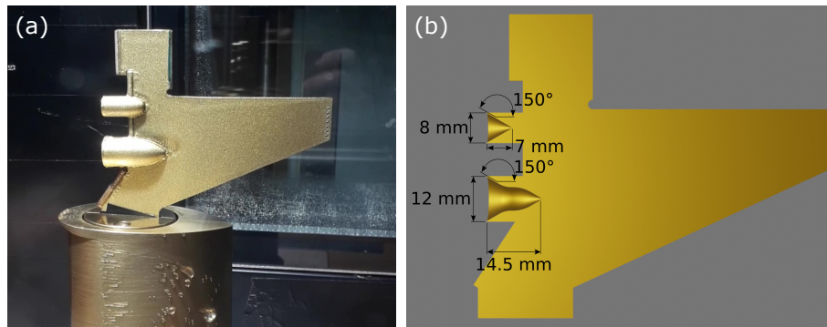
Figure 1. (a): Nevzorov probe in the BIWT with the new sensor head, which features a hotwire-an LWC sensor (top), an 8 mm total-water content-TWC collector cone (middle) and the new 12 mm total-water-content-TWC collector cone (bottom). The sensor head contains only one reference sensor which is positioned on the downwind side of the banneret that constitutes the top of the sensor head. (b): Cross section through the new Nevzorov sensor head and approximate dimensions of the sensors. The Nevzorov sensor heads are hand-made, therefore small differences may exist between sensor heads that are nominally the same model.
