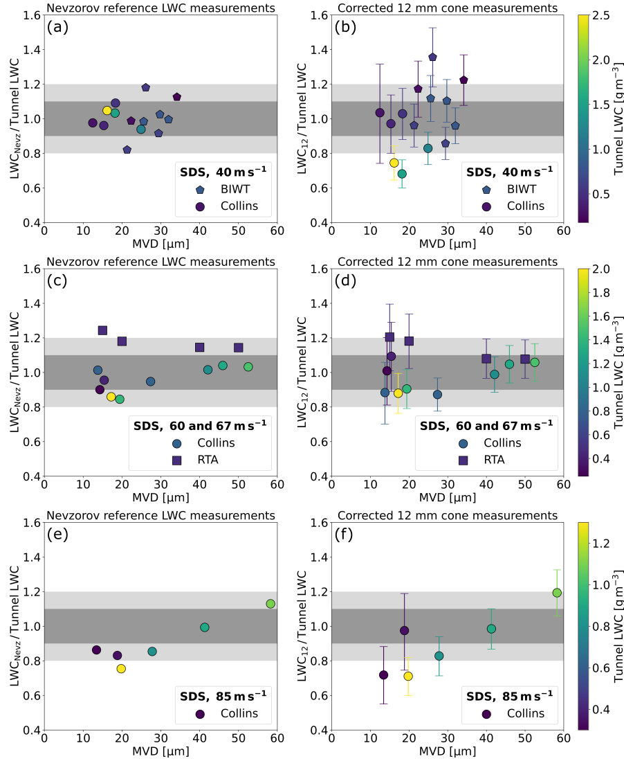
Figure 6. Comparison of the Nevzorov reference LWC and the corrected 12 mm cone LWC to the tunnel LWC for the three different airspeed groups. The error bars represent incorporate all uncertainty sources of the Nevzorov probe as detailed in Appendix A, including the uncertainty in the collision efficiency curve, that is described by the standard deviation of D_0 (see Table 5). They The error bars do not incorporate other uncertainty sources, such as biases in consider uncertainties not related to the Nevzorov 's response or probe, e.g. the IWT variability. For high MVDs, the error bars are in some cases too small to extend outside the marker.
