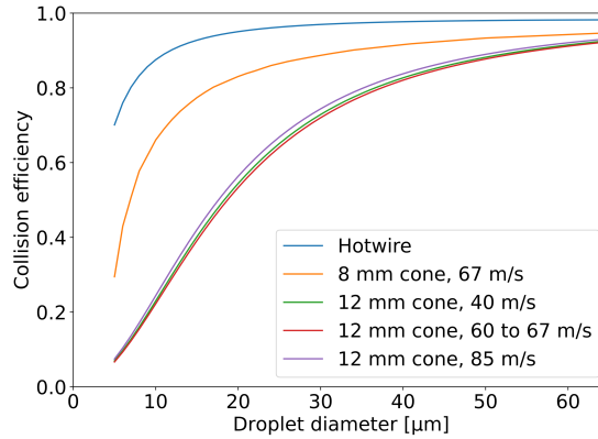
Figure 5. Collision efficiency curves of the 12 mm cone for the three airspeed groups, the collision efficiencies of the Hotwire-LWC sensor and the 8 mm cone from the literature are shown for comparison.
