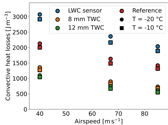
Figure A1. Convective heat losses of the Nevzorov sensors per volume of air. The volume of air that a sensor is exposed to is computed from the sample area and the airspeed. Turbulence and blockage effects that may occur around the sensors are not considered for this plot.
