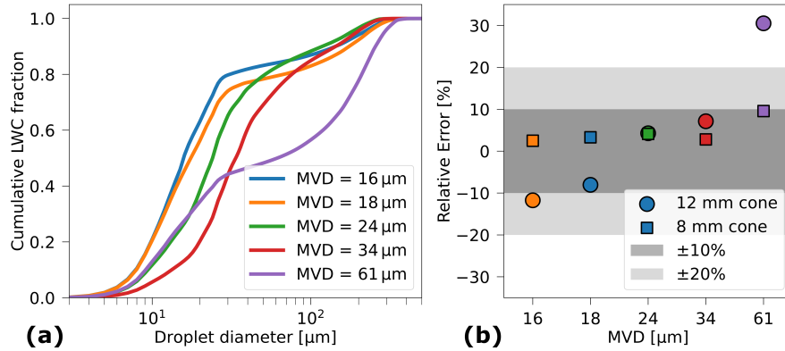
Figure 8. (a): Cumulative liquid water content of the bimodal DSDs measured in the BIWT. The distributions with the MVDs of 16, 18, and 61 \mu\text{m} have a small droplet mode centered around 15 \mu\text{m} and a large droplet mode at approximately 230 \mu\text{m} . They differ mainly in the ratio of LWC contained in small droplets to LWC contained in large droplets. The distributions with MVDs of 24 and 34 \mu\text{m} have their small droplet mode centered at 20 and 30 \mu\text{m} respectively and their large droplet mode at 165–166 \mu\text{m} . (b): Relative error of the LWC estimate that is introduced when approximating the collision efficiency from the MVD as compared to the collision efficiency estimated using the droplet size distributions DSDs shown on the left side.
